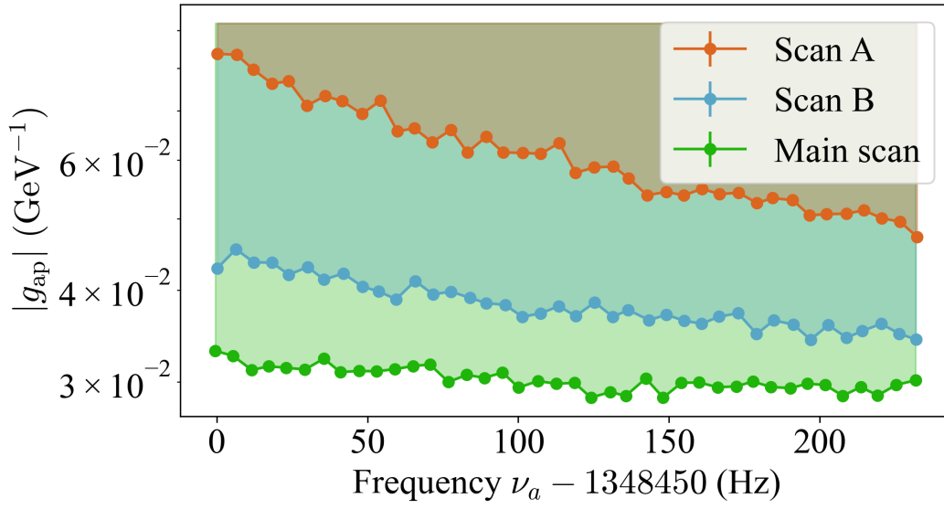
Figure 4.5: ALP gradient-proton coupling excluded at 95 % confidence level by the three sequential scans. Each data point represents the sensitivity for one scan step. The variation in sensitivity between scans reflects the daily modulation of the ALP wind direction relative to the bias field. Reproduced from Ref. [39].
