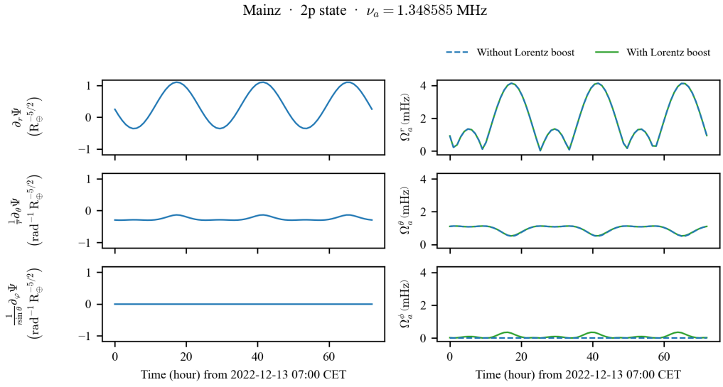
Figure 2.6: Daily modulation of the gradient component for the 2p state (n, l, m) = (2, 1, 0) at the location of CASPER-G (Helmholtz Institute Mainz). The modulation is due to the rotation of the Earth.
