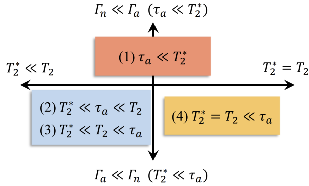
Figure 2.1: Regimes of the spin-precession experiment based on the relative magnitudes of T_2 , T_2^* , and \tau_a . Reproduced from Ref. [45].
