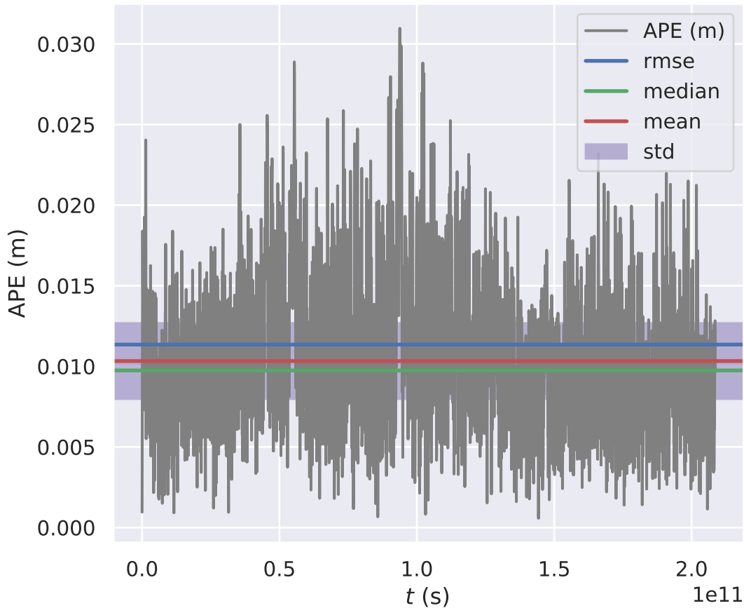
APE w.r.t. translation part (m) (with Sim(3) Umeyama alignment)
