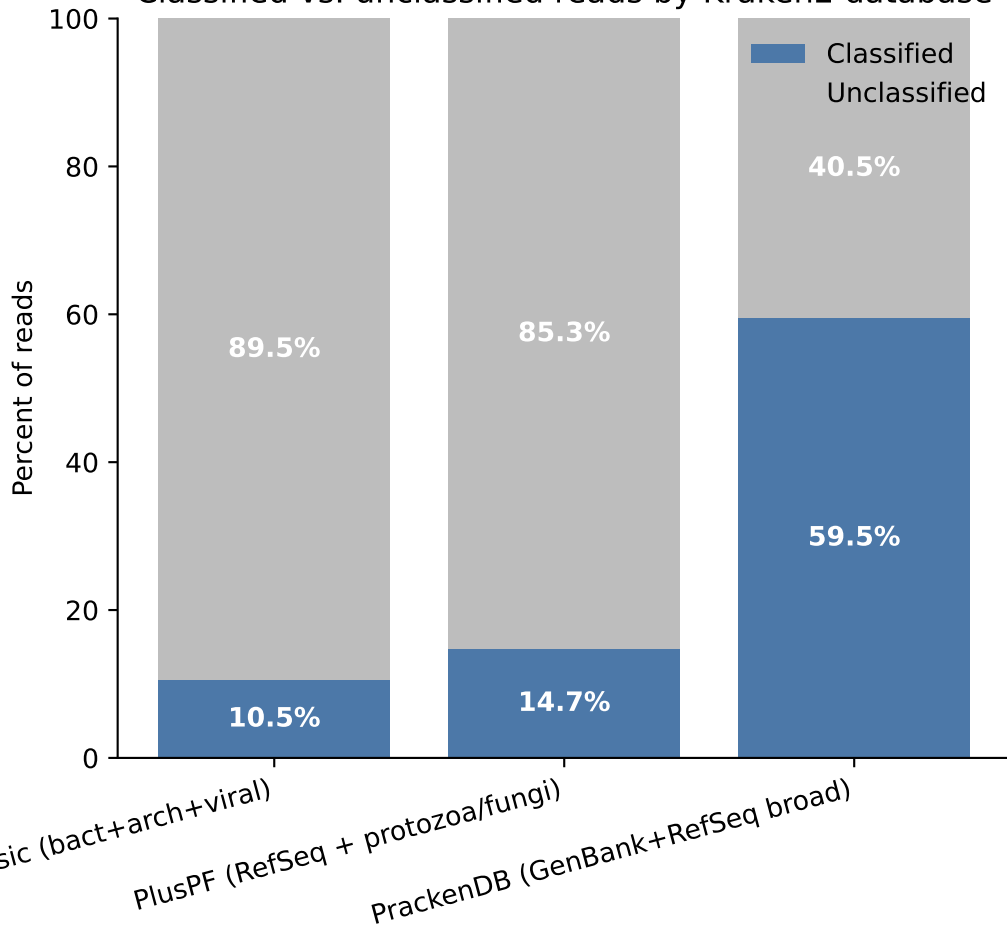
Classified vs. unclassified reads by Kraken2 database
