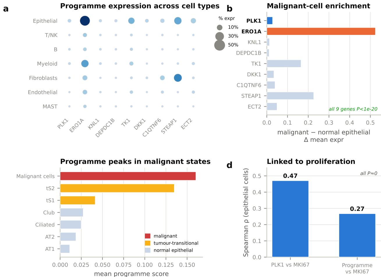
Figure 6 Single-cell (GSE131907, 208,506 cells): the programme is malignant-epithelial-specific
