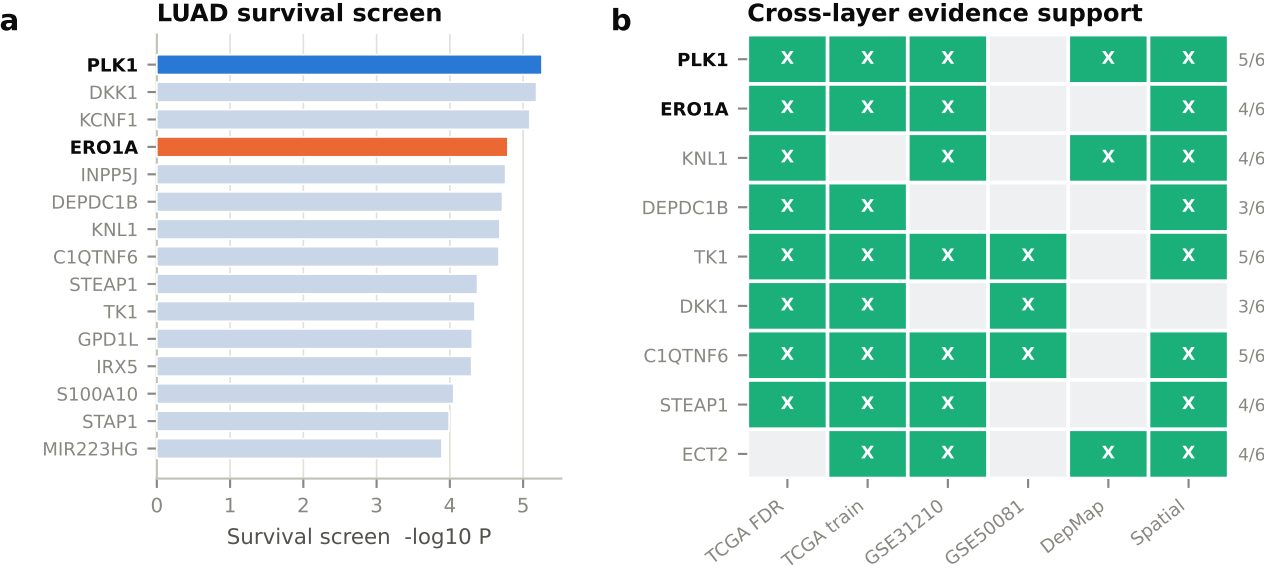
Figure 1 Literature-guided TCGA discovery of a PLK1-centred mitotic/redox programme
