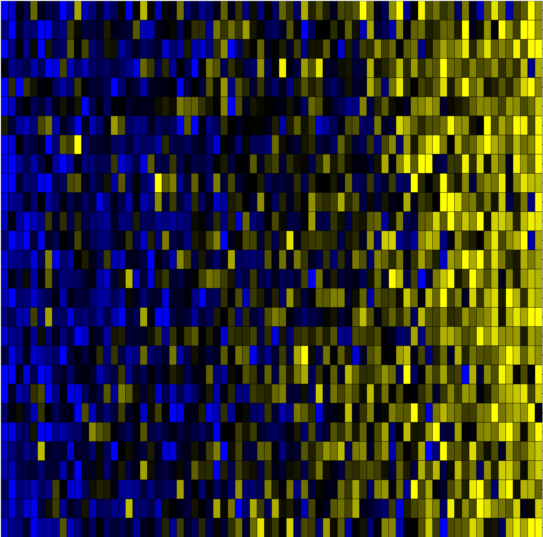
Expression Data
