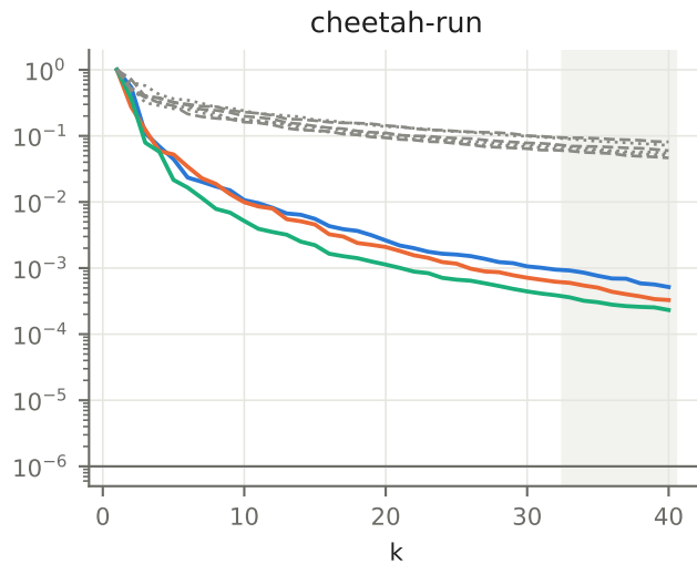
Pooled Hankel singular values, H = 64 ( \sigma/\sigma_1 )
