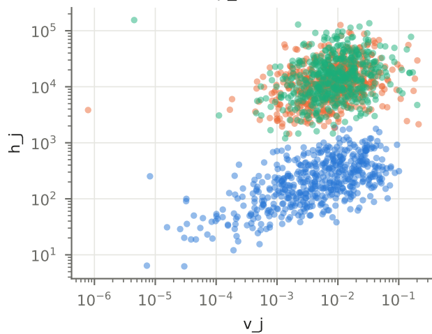
humanoid-walk \rho_S = 0.54, 0.55
