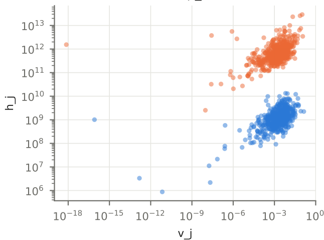
humanoid-walk \rho_S = 0.54, 0.55
