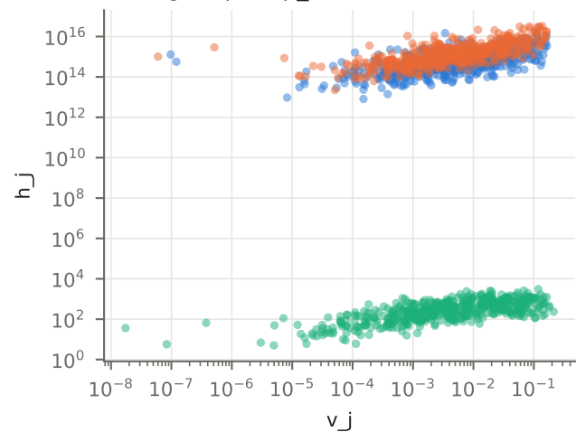
finger-spin \rho_S = 0.65, 0.73, 0.66
