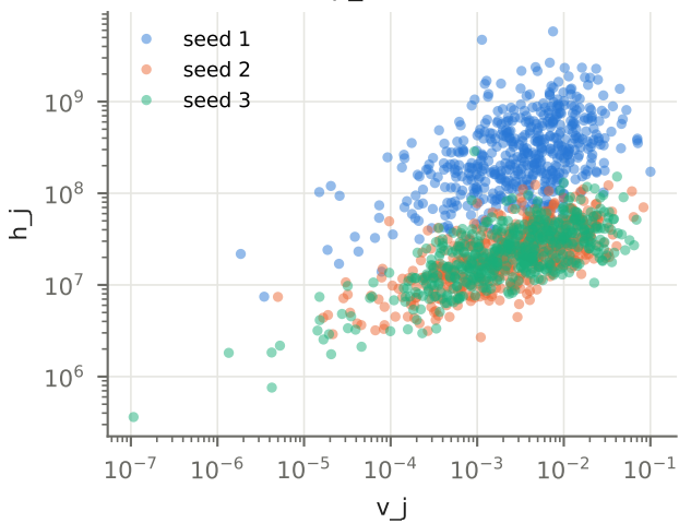
quadruped-run \rho_S = 0.24, 0.31, 0.40
