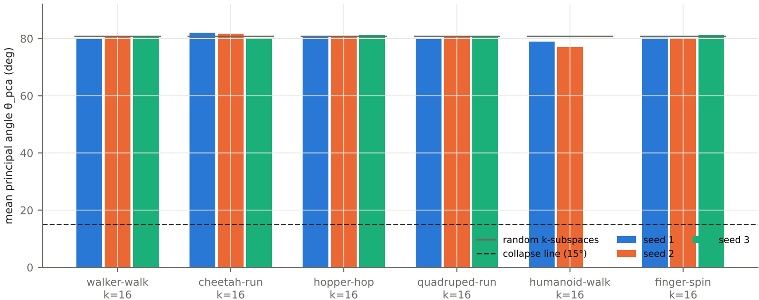
Balanced vs PCA subspace
