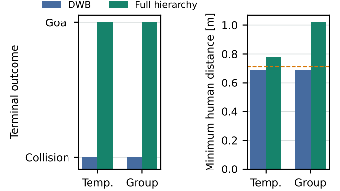
Fig. 4. Two cross-family validation examples. Each pair uses one scenario, seed, and code revision for both methods. The full hierarchy reaches the physical goal after the corresponding DWB collision; the dashed line marks the 0.71 m geometric collision threshold. These single pairs are not pooled for significance testing.
