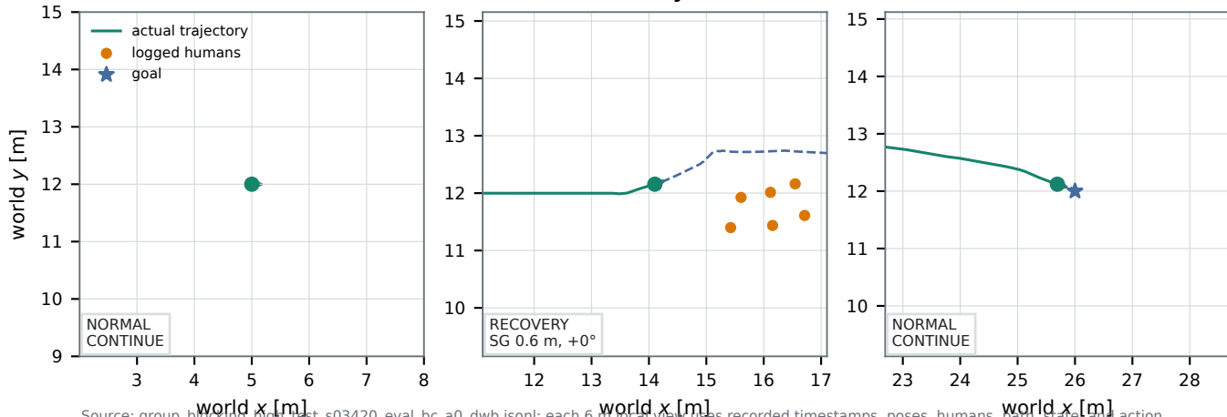
Logged PGRR runtime sequence — group_blocking / high (successful triggered recovery) (a) Start: t=0.0 s (b) First recovery: t=38.5 s (c) Terminal: t=143.8 s
