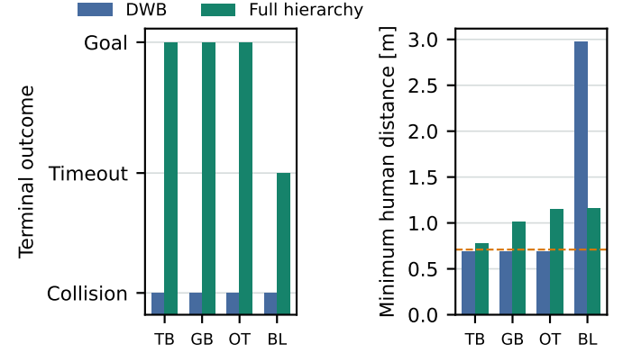
Fig. 4. Four cross-family validation examples: temporary blockage (TB), group blocking (GB), overtaking (OT), and blind corner (BL). Each pair uses one scenario, seed, and code revision for both methods. The dashed line marks the 0.71 m geometric collision threshold. These single pairs are not pooled for significance testing.
