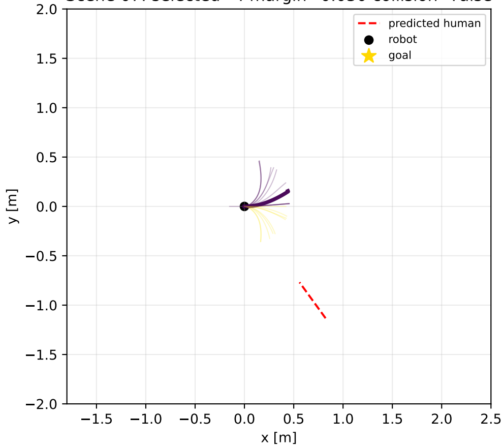
Scene 07: selected=4 margin=0.030 collision=False
