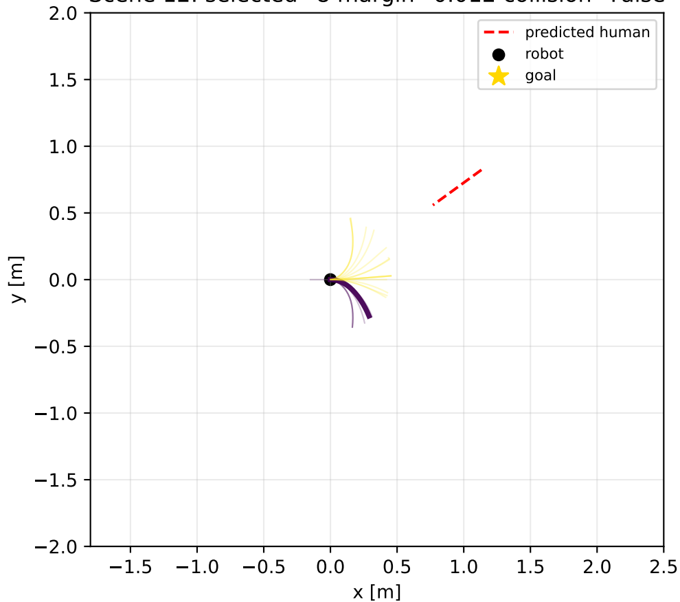
Scene 12: selected=8 margin=0.012 collision=False
