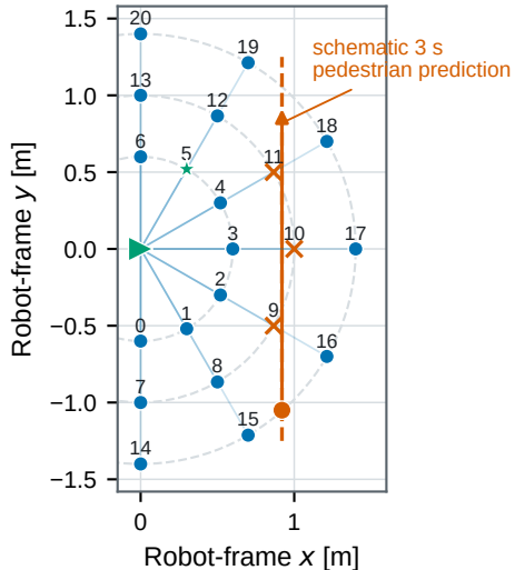
(a) Temporary subgoals
