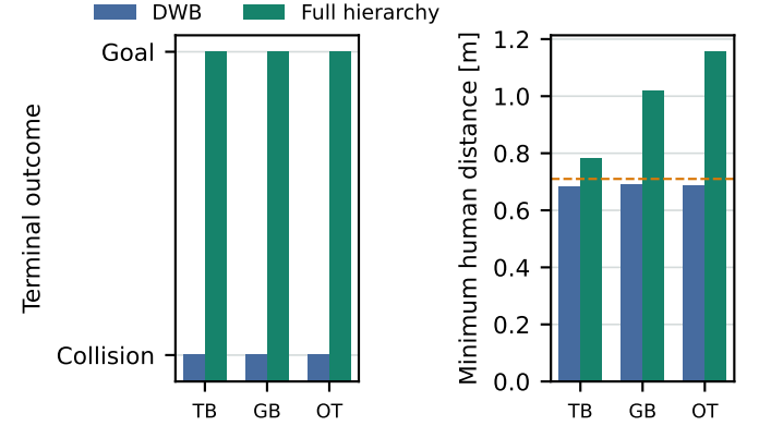
Fig. 4. Three cross-family validation examples: temporary blockage (TB), group blocking (GB), and overtaking (OT). Each pair uses one scenario, seed, and code revision for both methods. The full hierarchy reaches the physical goal after the corresponding DWB collision; the dashed line marks the 0.71 m geometric collision threshold. These single pairs are not pooled for significance testing.
