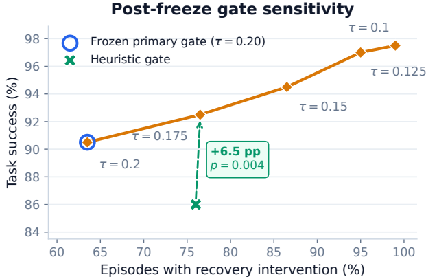
Fig. 3. Post-freeze gate sensitivity on a separate set of 200 paired Meta-World seeds at 20% disturbance. Each point is labeled by \tau_{on} ; the green cross is the semantic heuristic evaluated on the same serialized CRN bank. The circled 0.20 operating point remains the frozen primary gate, while the dashed comparison at 0.175 exposes matched intervention burden. This diagnostic was not used for model or threshold selection.
