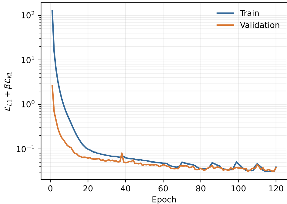
ACT objective
