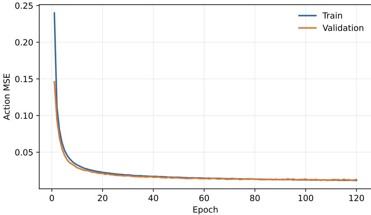
Shared multi-task MLP-BC
