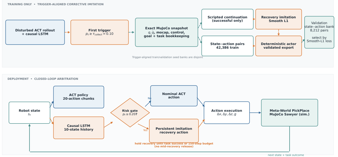
Fig. 1. REIM training and deployment architecture. The environment block is explicitly the Meta-World PickPlace task running in MuJoCo with a simulated Sawyer model. Dashed training-only paths denote exact simulator snapshot capture, scripted corrective demonstrations, and validation-loss checkpoint selection; the scripted expert is never queried during evaluation.
