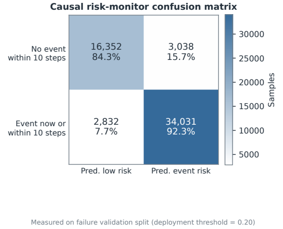
Fig. 4. Causal risk-monitor confusion matrix on the trajectory-grouped validation split at \tau = 0.20 . Counts are (TN, FP, FN, TP) = (16,352, 3,038, 2,832, 34,031).
