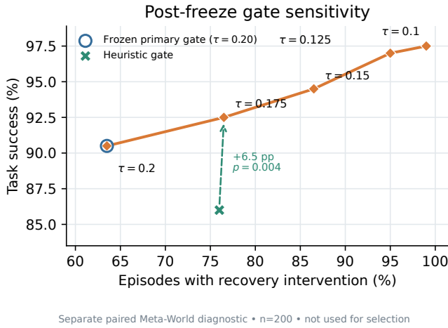
Fig. 3. Post-freeze gate sensitivity on a separate set of 200 paired Meta-World seeds at 20% disturbance. Each point is labeled by \tau_{on} ; the green cross is the semantic heuristic evaluated on the same serialized CRN bank. The circled 0.20 operating point remains the frozen primary gate, while the dashed comparison at 0.175 exposes matched intervention burden. This diagnostic was not used for model or threshold selection.
