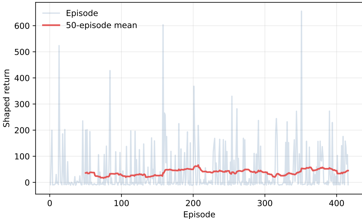
PPO Recovery Training
