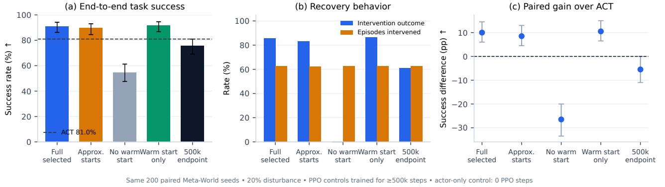
Fig. 9. Recovery training-design controls on the same 200 paired Meta-World seeds at 20% disturbance. (a) End-to-end success with 95% Wilson intervals; the dashed line marks the ACT reference. (b) Recovery intervention outcome and intervened-episode rates. (c) Paired success difference over ACT with 95% bootstrap intervals. PPO controls receive at least 500k environment steps; the actor-only row receives zero.
