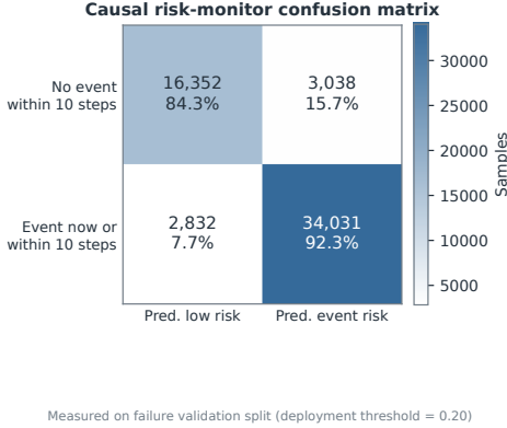
Fig. 5. Causal risk-monitor confusion matrix on the trajectory-grouped validation split at \tau = 0.20 . Counts are (TN, FP, FN, TP) = (16,352, 3,038, 2,832, 34,031).
