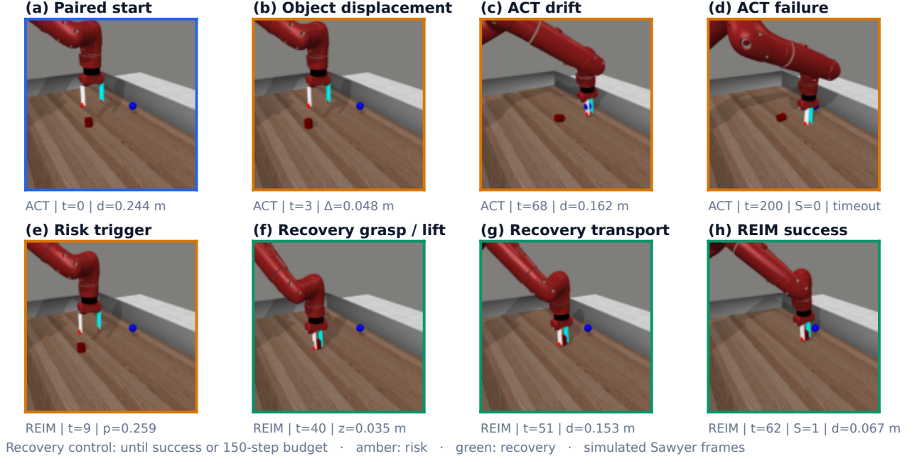
Fig. 6. Paired qualitative operation sequence from separate simulation seed 8,300,042 at 20.0% disturbance. With the frozen evaluation gate \tau_{\text{on}} = 0.20 , ACT does not complete the task within 200 steps, whereas REIM triggers once and completes in 62 steps, including 53 supervised-recovery actions. These are rendered Meta-World/MuJoCo frames of the simulated Sawyer model, not hardware photographs. This selected trace explains controller operation and does not estimate aggregate success.
