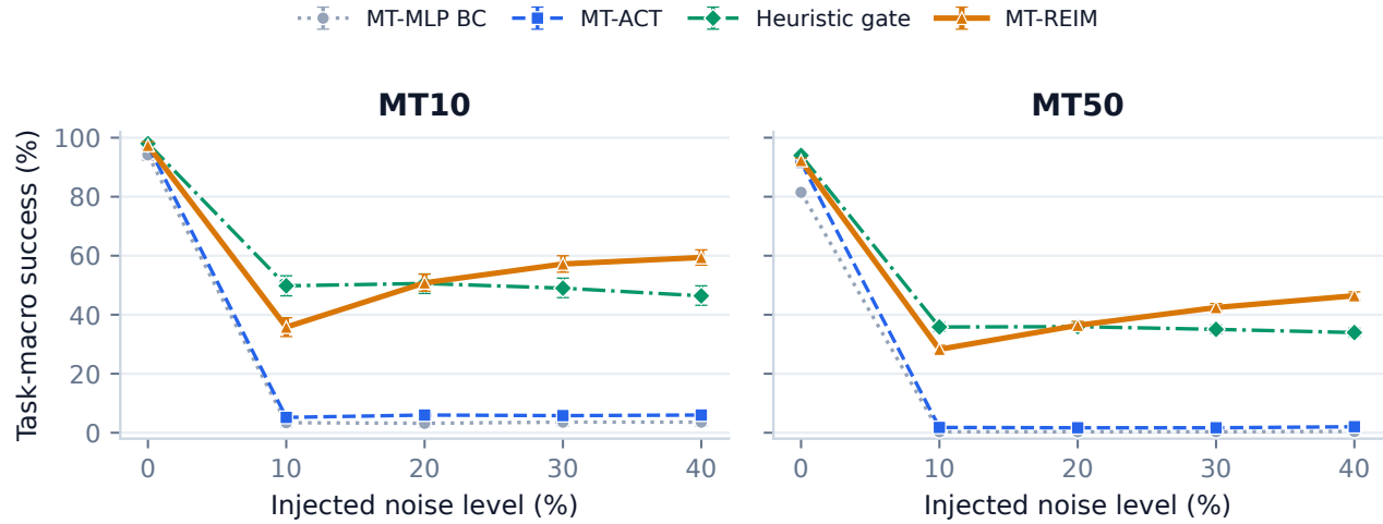
REIM robustness extension — task-universal action/observation noise; not official Meta-World scores
