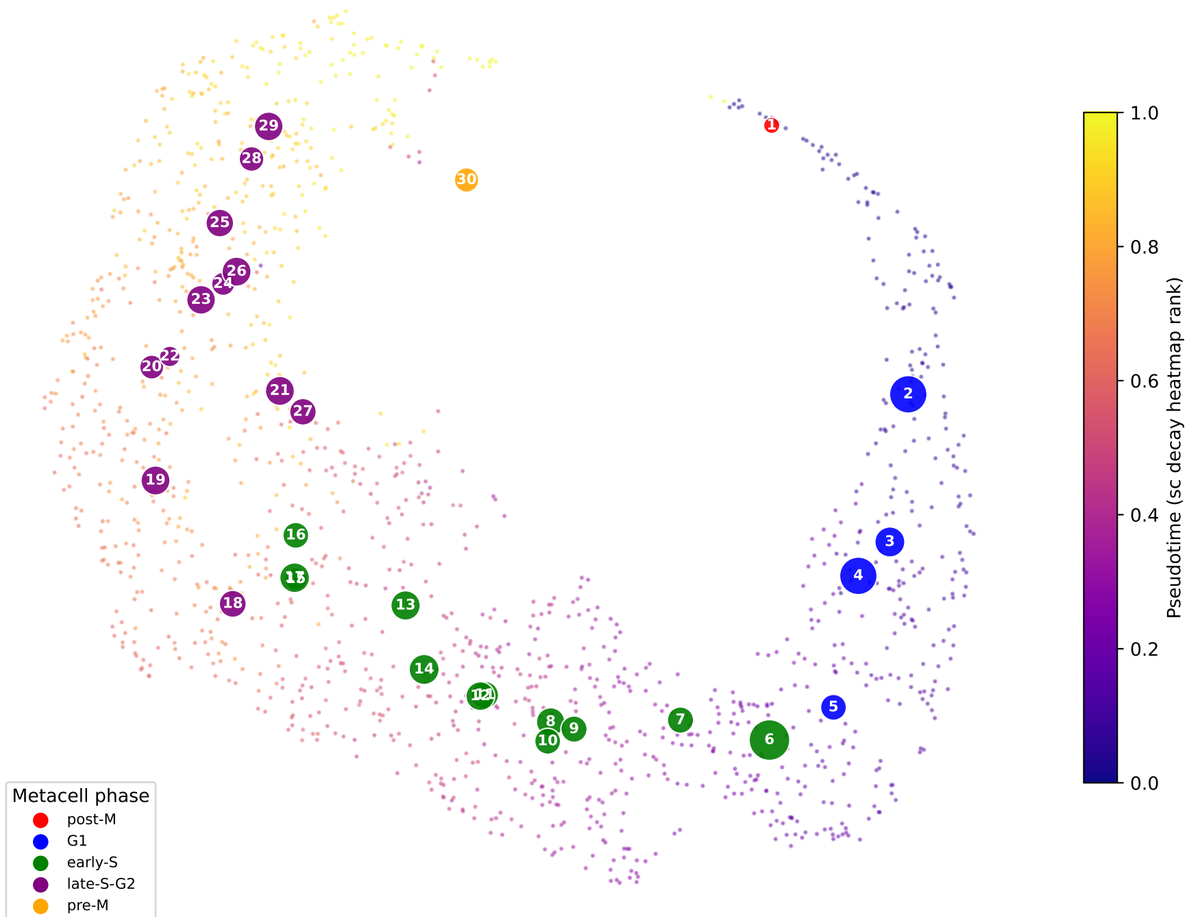
Decay-profile UMAP Single cells: pseudotime color | Metacell: phase color + rank label
