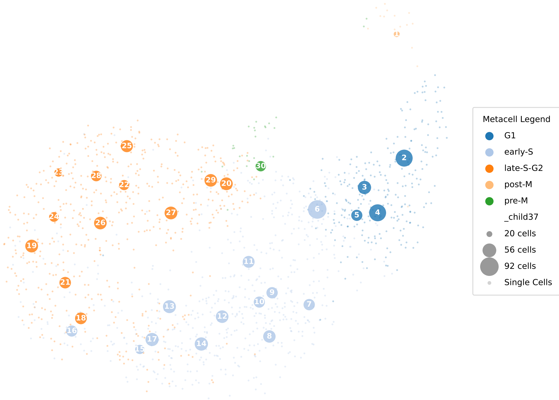
Metacell Pseudotime Order (Metacells: 30, pseudotime rank labeled)
