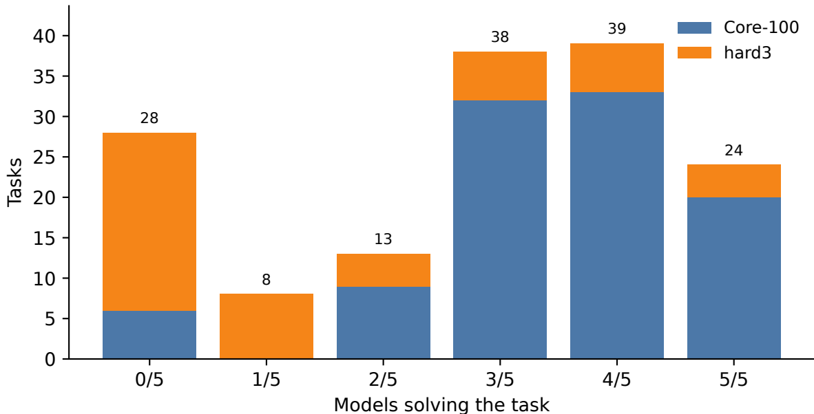
Models solving each task (5 backends, no GLM)
