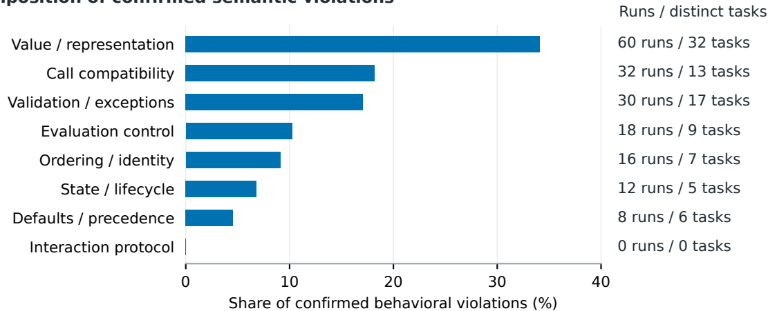
(a) Composition of confirmed semantic violations
