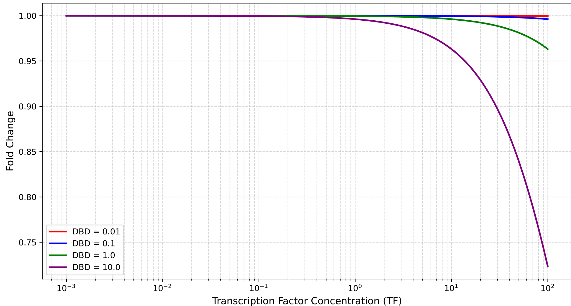
Rob Phillips Model: Fold Change vs TF Concentration At Fixed DBD Concentrations (Inducer Fixed)
