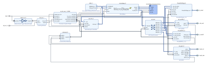
Fig. 8: Vivado Block Diagram showing MicroBlaze Processor and Pmod Peripherals.
