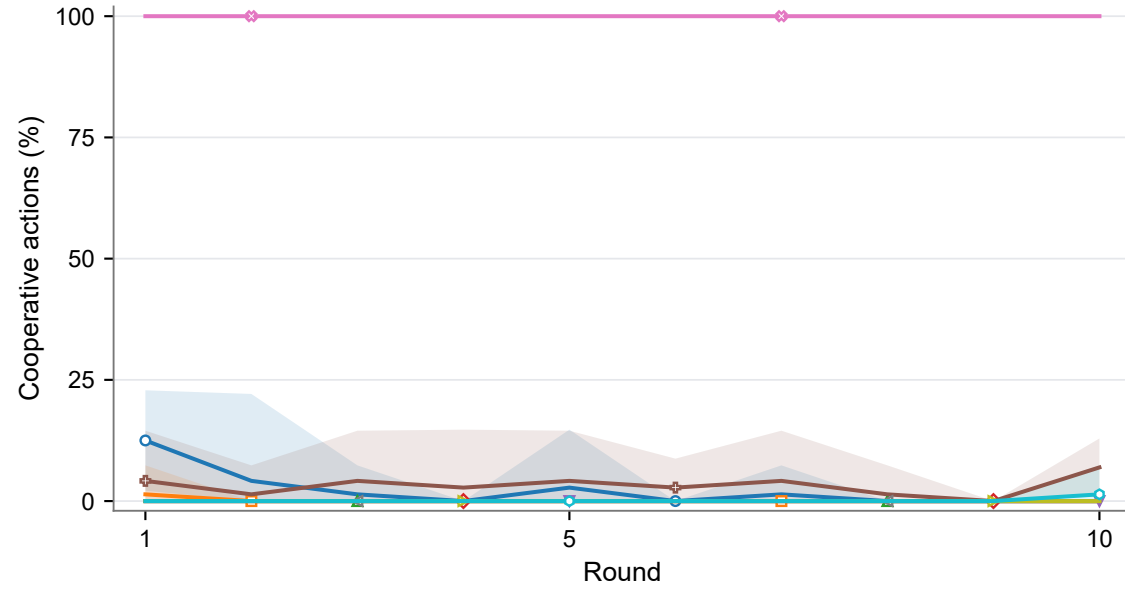
a Prisoner's dilemma
