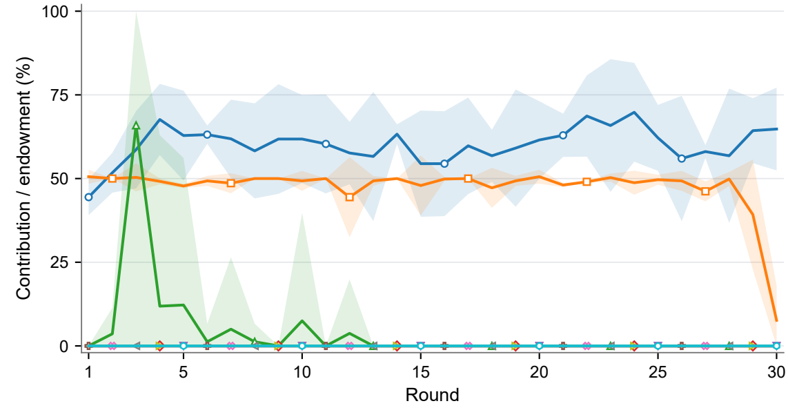
b Public-goods game
