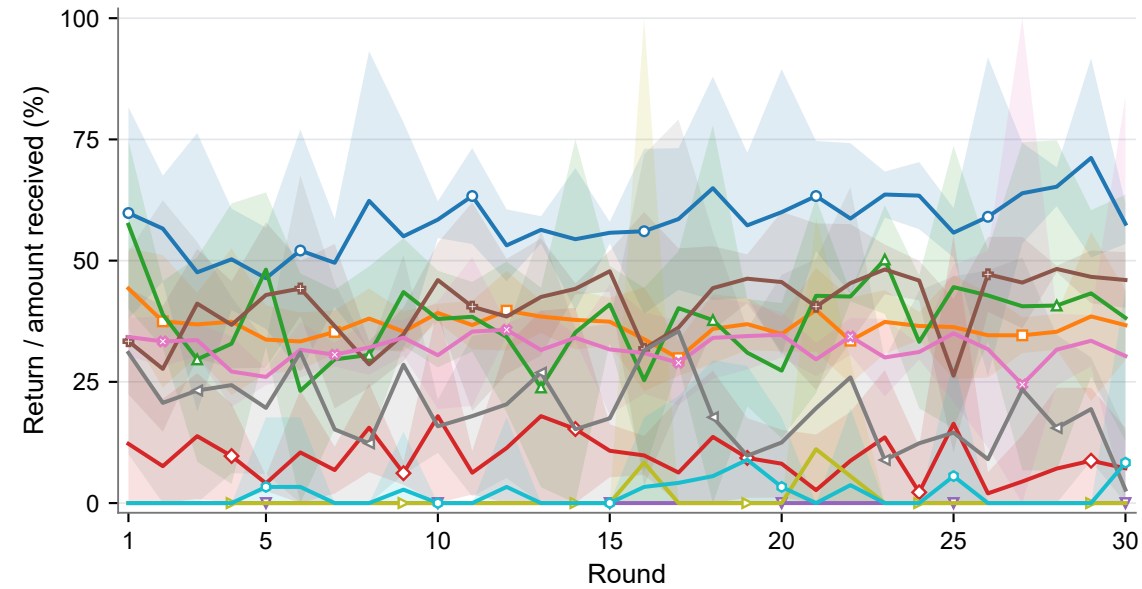
d Trust game: Receiver
