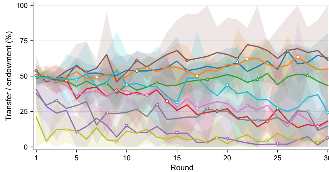
c Trust game: Sender
