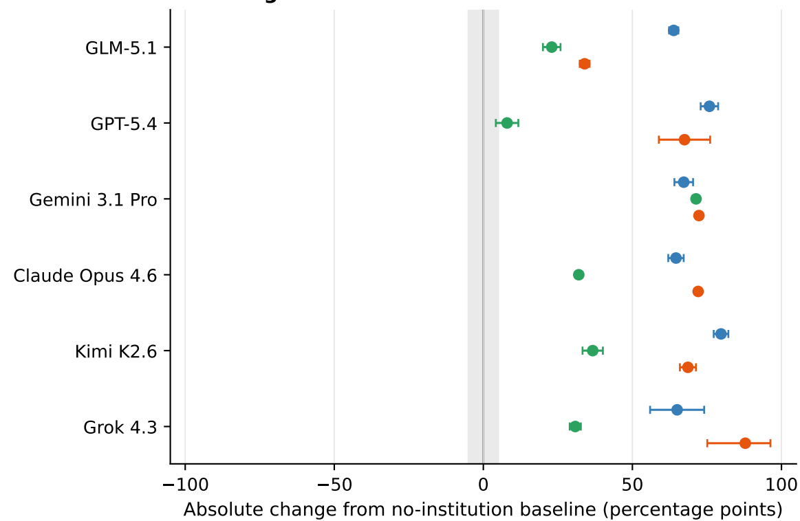
C Trust game: Sender transfer
