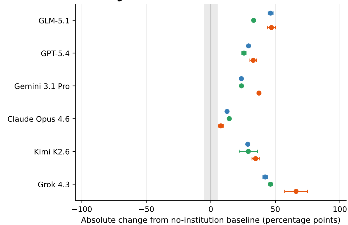
D Trust game: Receiver conditional return
