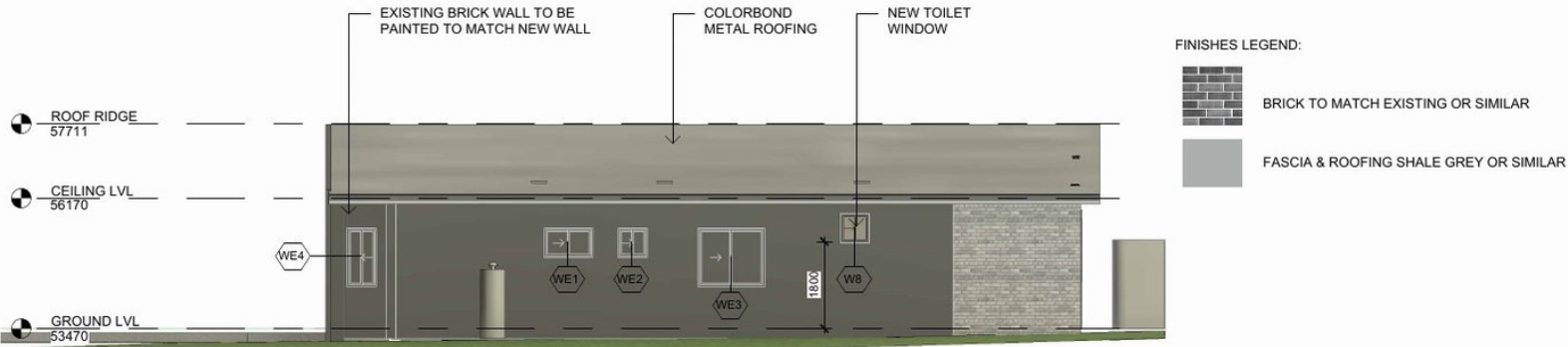
1 WEST ELEVATION 1 : 100
