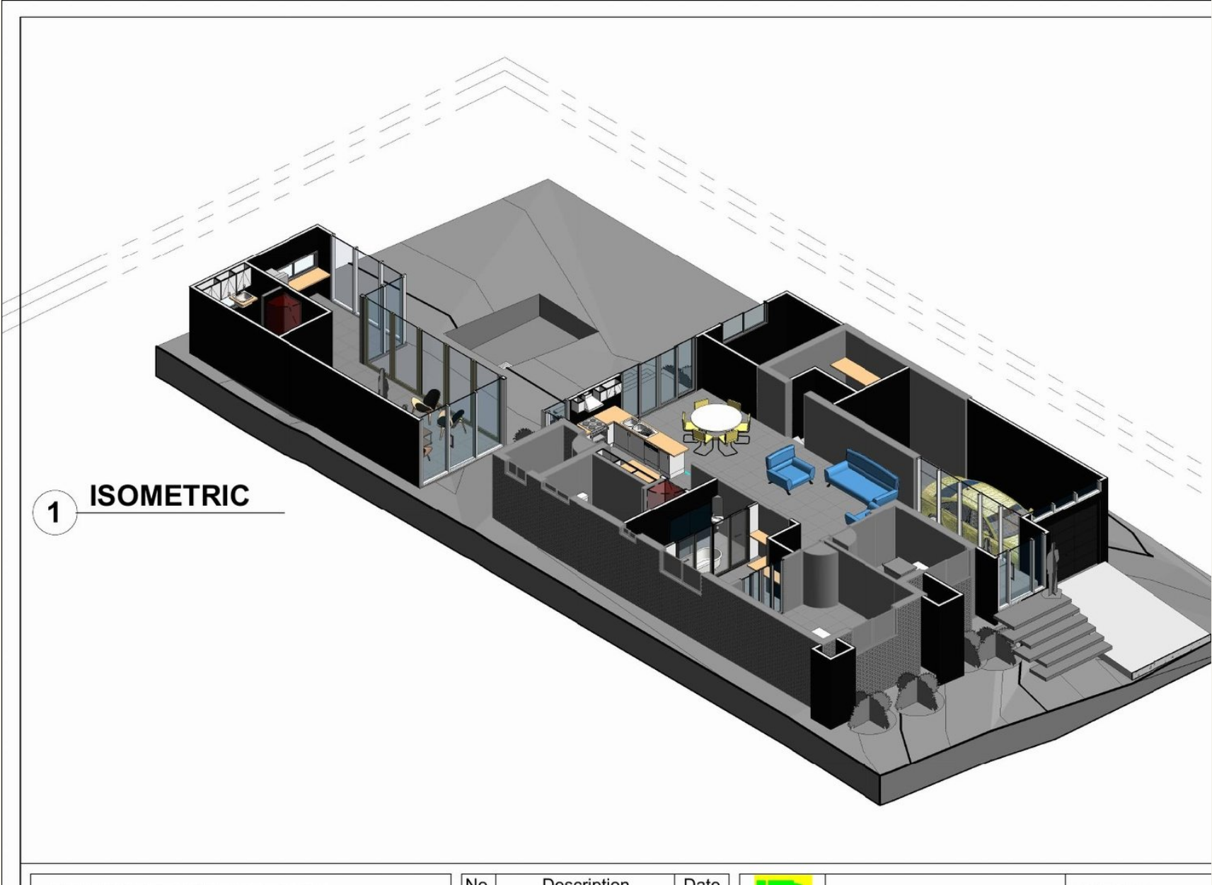
Market Street Residence Smithfield, NSW | Renovation + addition | Isometric study
