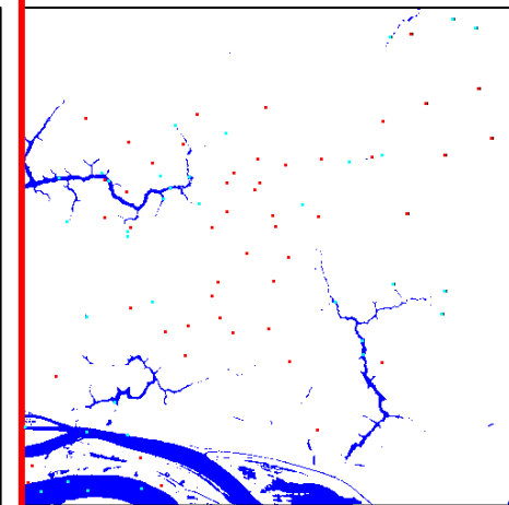
Rede Neural
