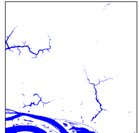
Rede Neural
