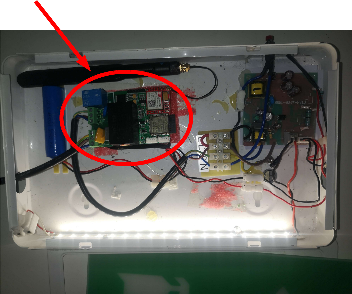
Retro-Fitted exitLight health check monitor
