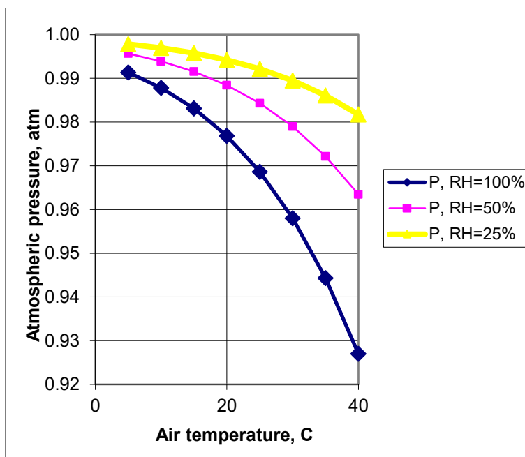
Figure 68. Atmospheric pressure correction as a result of vapor pressure correction assuming original atmospheric pressure is 1 atm.
