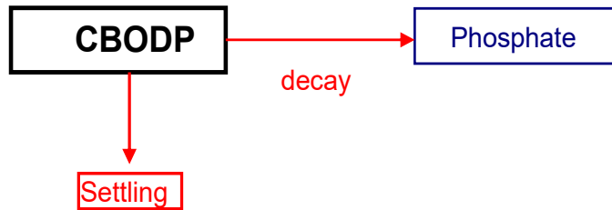
Figure 86. Internal flux between and other compartments.
