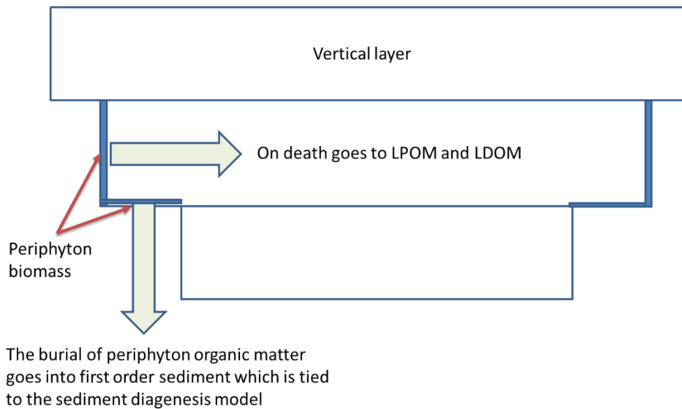
Figure 91. How epiphyton/periphyton transfer organic matter to the water column at death and to the sediment during burial.
