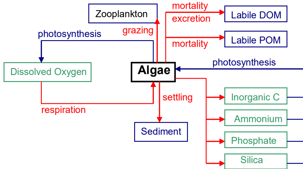
Figure 88. Internal flux between algae and other compartments.
