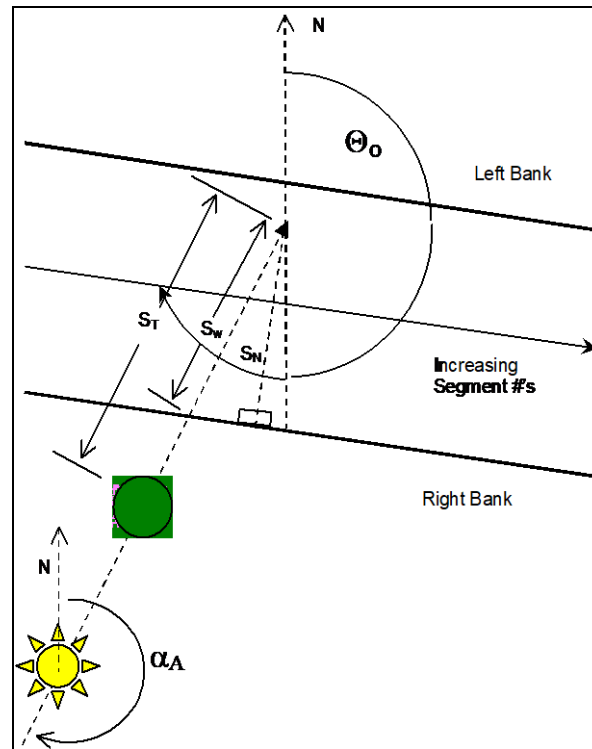
Figure 60. Azimuth angle, \alpha_A , and stream orientation, \Theta_o .
