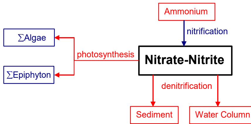
Figure 96. Internal flux between nitrate + nitrite and other compartments.
