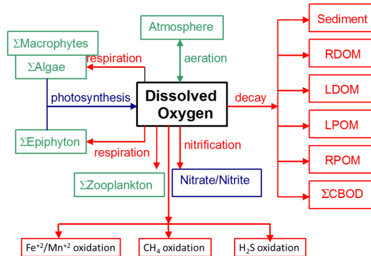
Figure 99. Internal flux between dissolved oxygen and other compartments.
