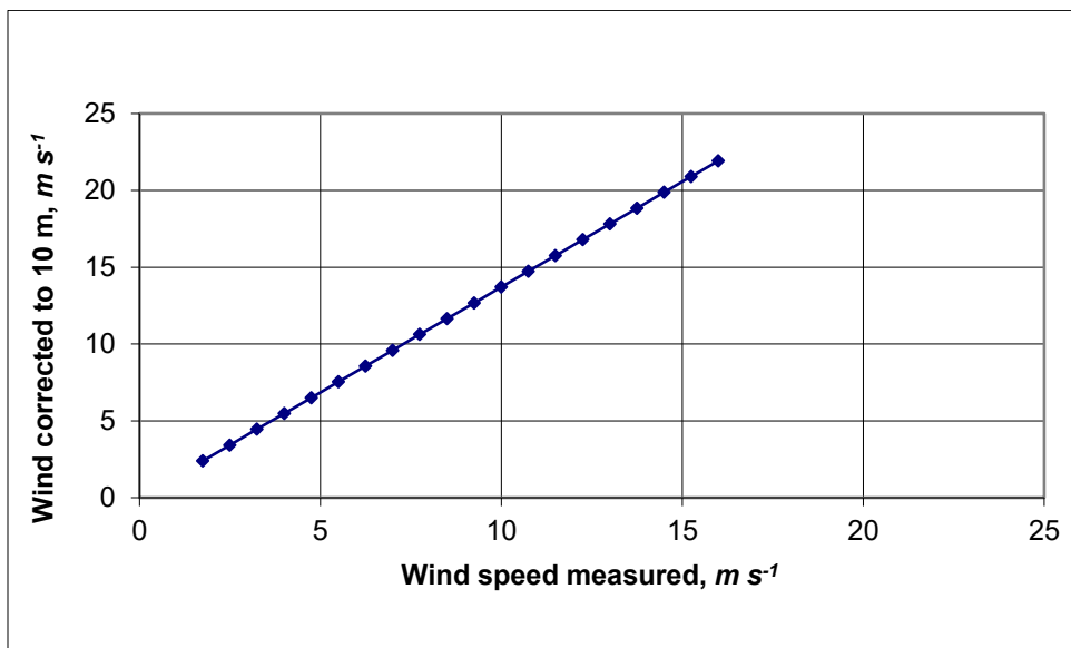
Figure 104. Wind corrected to 10 m based on wind measured on land.
