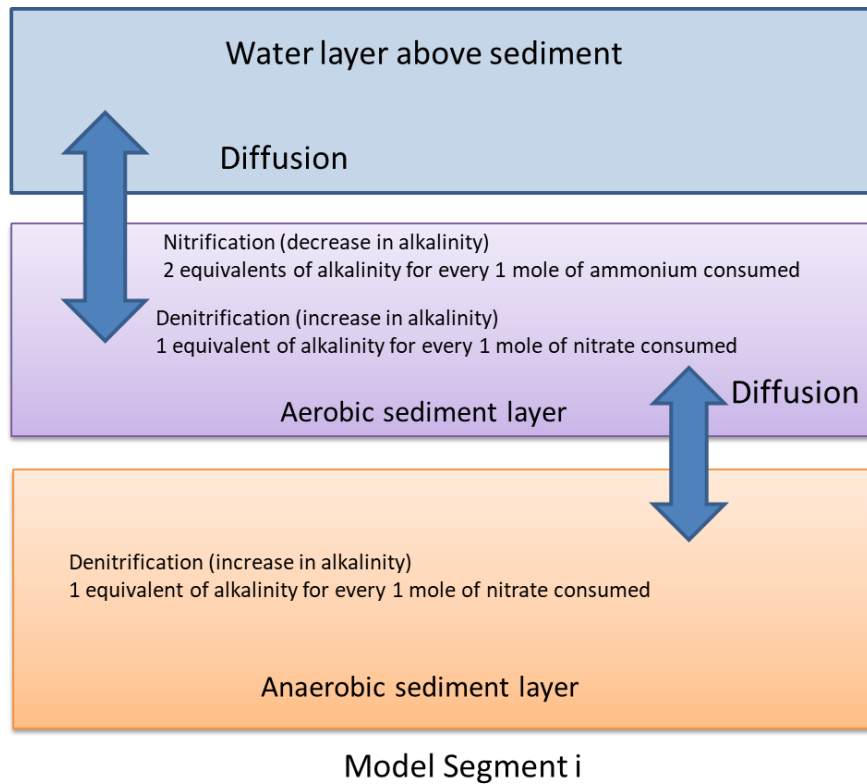
Figure 114. Sources and sinks of the sediment alkalinity model.
