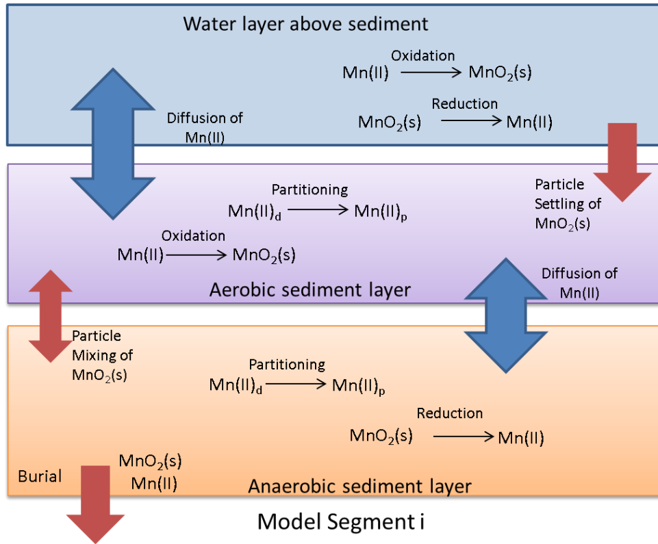
Figure 117. Schematic of manganese model (DiToro, 2001).
