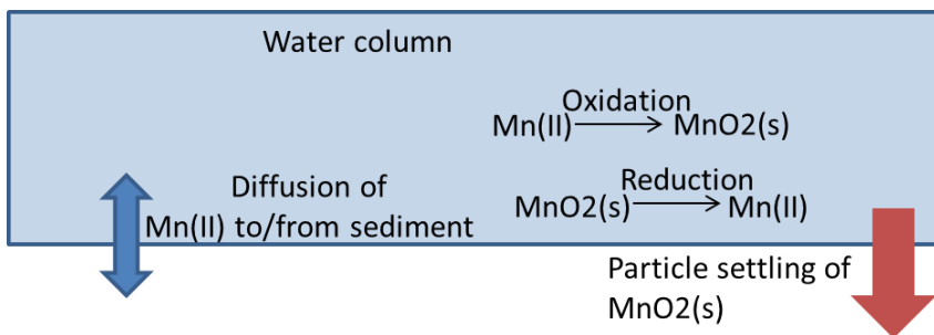
Figure 73. Sources and sinks of Mn in the water column.
