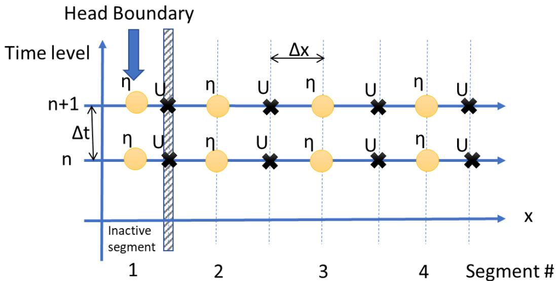
Figure 126. Grid for computation of a head boundary in x . U , the longitudinal velocity, at the flow boundary or at the right-hand side of inactive segment 1 is computed from the head difference between the boundary head (at center of inactive segment 1) and the head at the first grid cell (segment 2).
