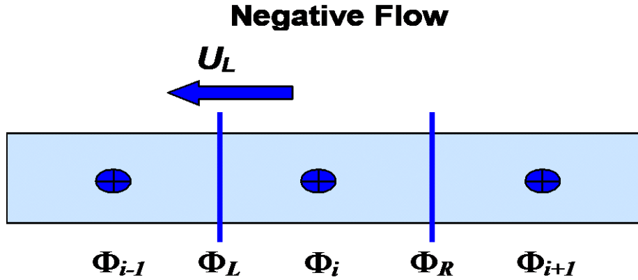
Figure 134. ULTIMATE schematization for negative flow.
