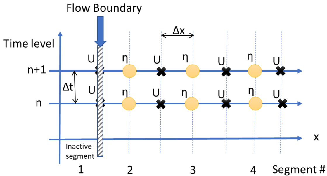
Figure 125. Grid for computation of a flow boundary in x . U , the longitudinal velocity, at the flow boundary or at the right-hand side of inactive segment 1 is computed from the flow rate.
