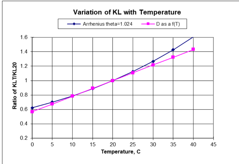
Figure 105. Variation of K_{LT}/K_{L20} as a function of temperature.
