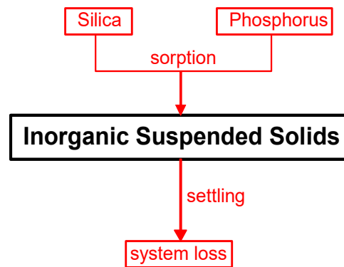
Figure 74. Internal flux for inorganic suspended solids.
