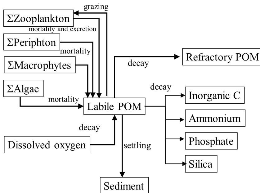
Figure 78. Internal flux between Labile POM and other compartments.
