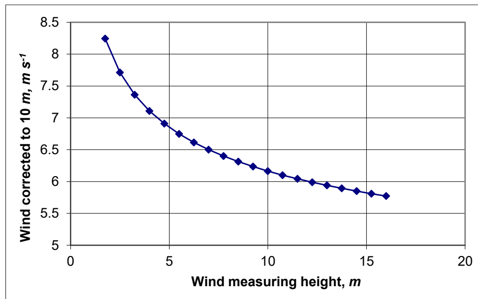
Figure 102. Wind speed of 5 m s^{-1} and a fetch of 5 km corrected to 10 m as a function of measuring height on land.
