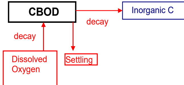
Figure 85. Internal flux between CBOD and other compartments in Version 3.7 and later.
