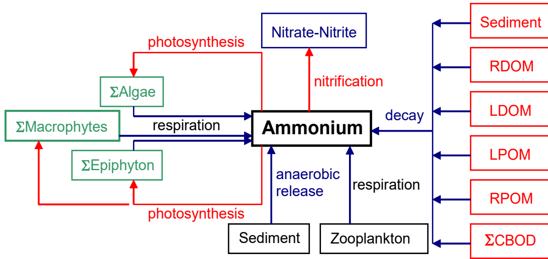
Figure 95. Internal flux between ammonium and other compartments.
