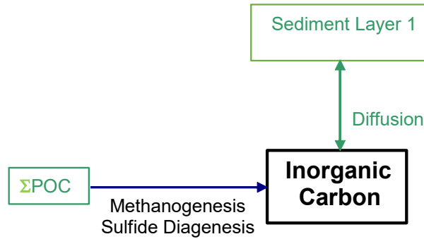
Figure 113 Internal flux between inorganic carbon within the anaerobic sediment layer 2 and other compartments.
