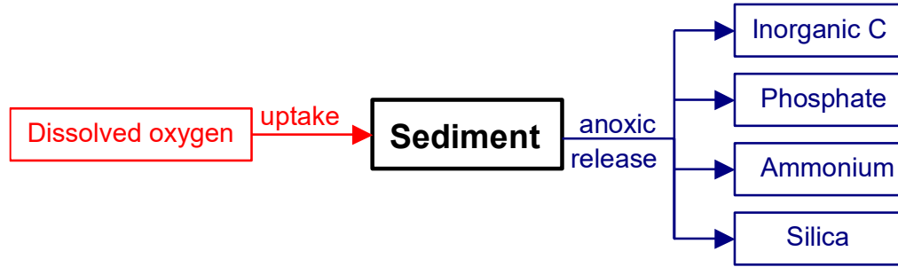
Figure 106. Internal flux between 0-order sediment compartment and other compartments.
