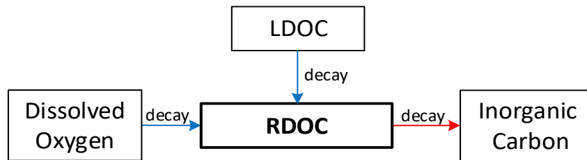
Figure 83. Kinetics of RDOC in the water column.
