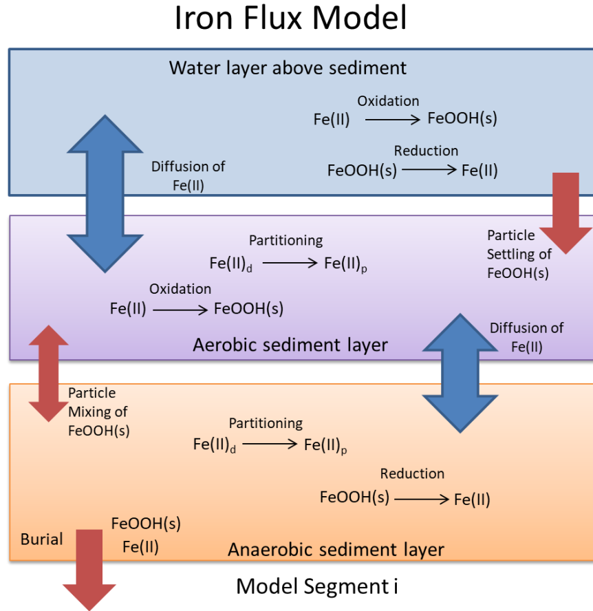
Figure 116. Schematic of iron model (Ditiro, 2001).
