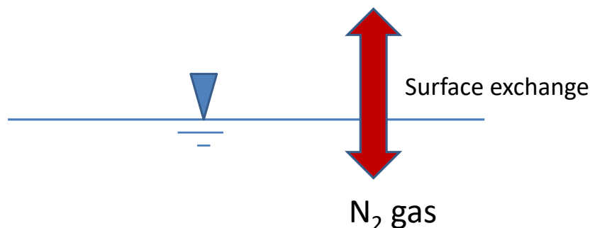
Figure 65. N 2 gas exchange.
