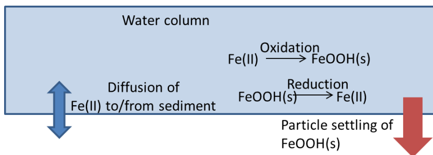
Figure 72. Sources and sinks of Fe in the water column.
