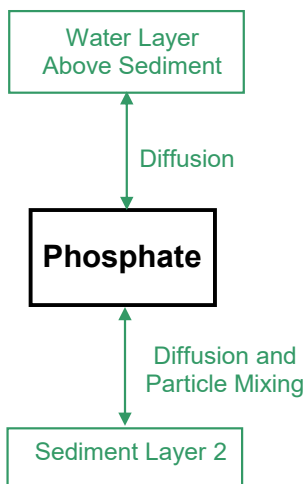
Figure 109. Internal flux between phosphate within the aerobic sediment layer 1 and other compartments.
