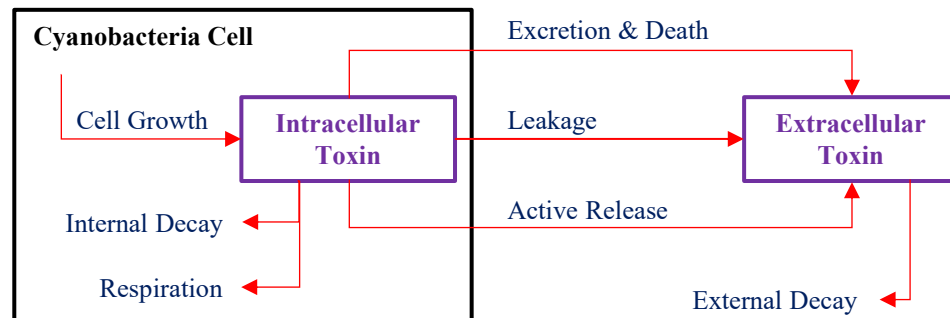
Figure 89. Sources and sinks of the intracellular and extracellular toxins.
