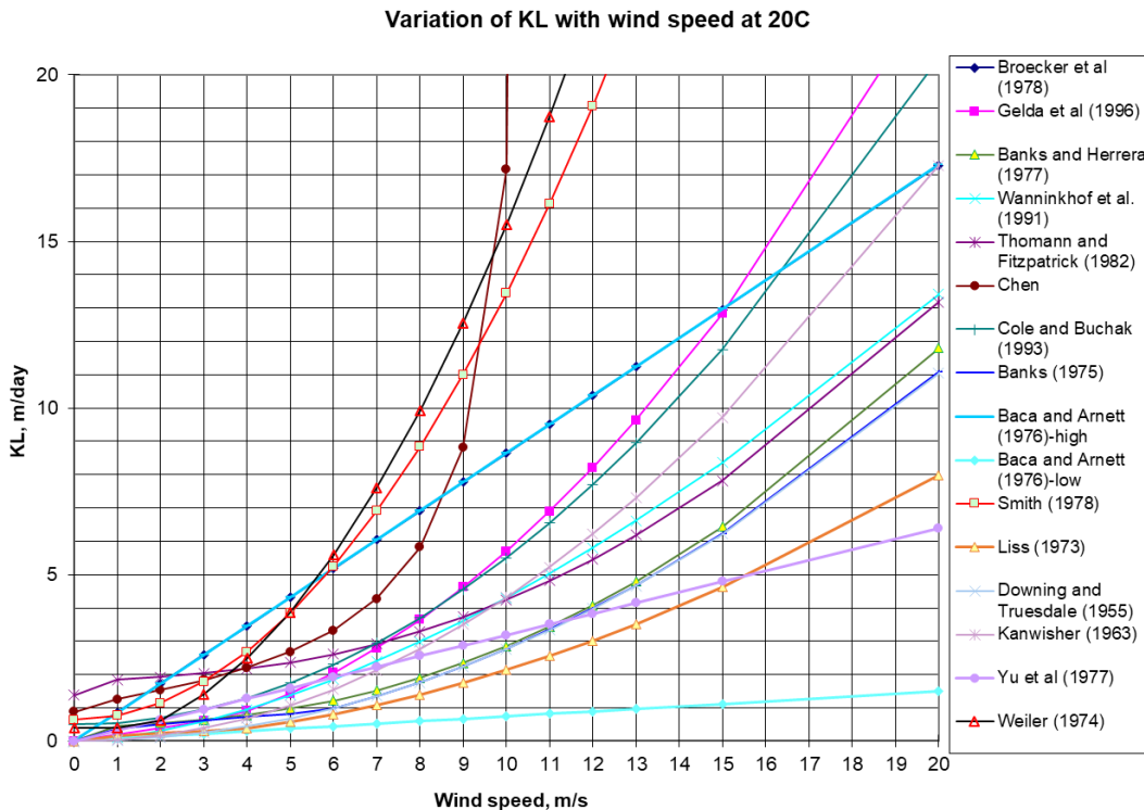
Figure 101. Variation of wind speed and KL for lake/reservoir equations.
