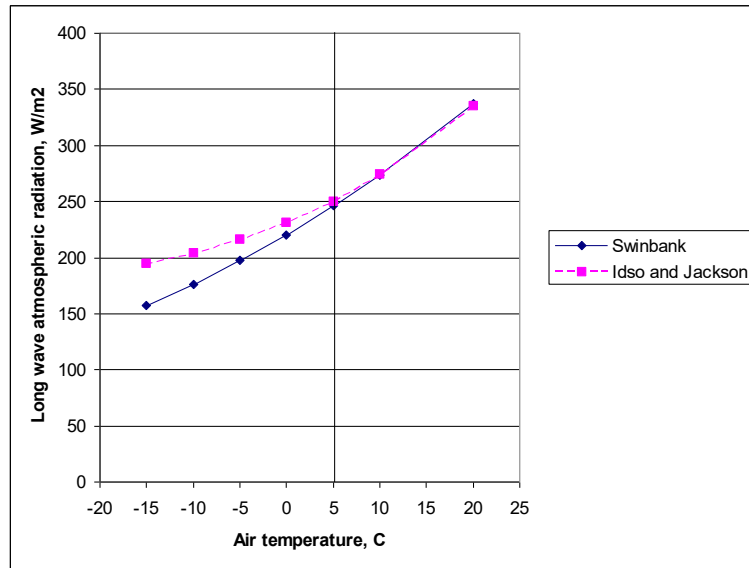
Figure 53. Difference in incoming long wave atmospheric radiation formulae between Swinbank and Idso and Jackson.
