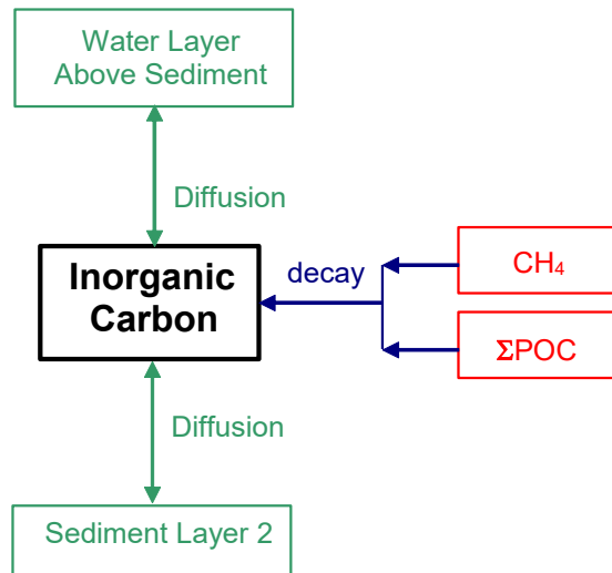
Figure 112 Internal flux between inorganic carbon within the aerobic sediment layer 1 and other compartments.
