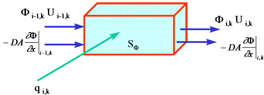
Figure 130. Horizontal advective and diffusive transport.
