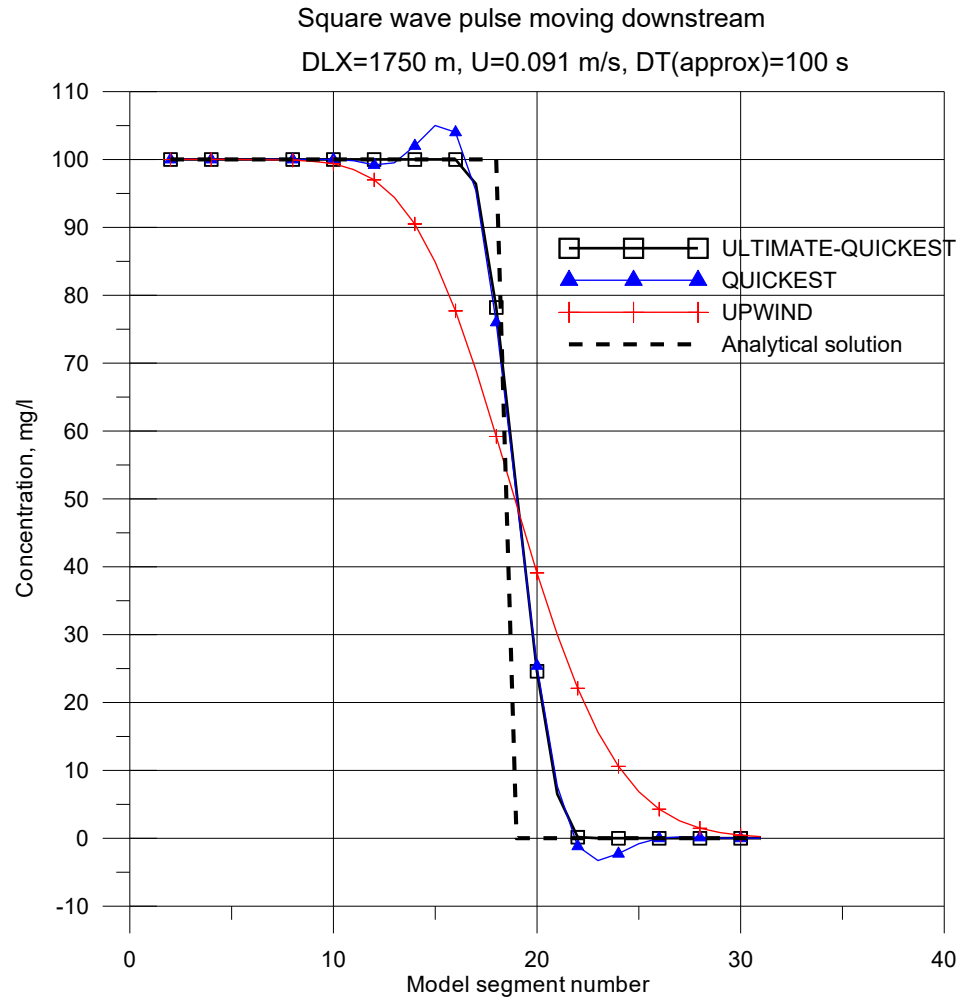
Figure 136. Comparison of UPWIND, QUICKEST, and ULTIMATE/QUICKEST schemes for conservative tracer transport.
