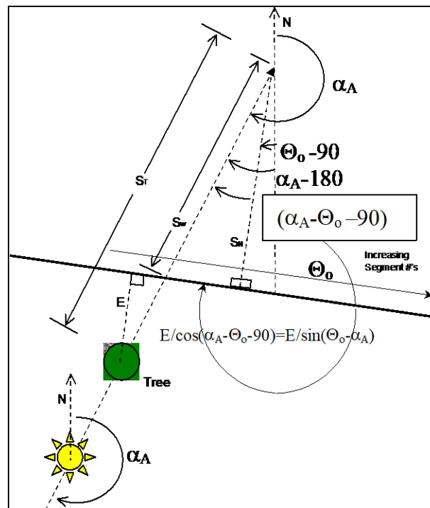
Figure 61. Relationship between azimuth, stream orientation, and shadow length.
