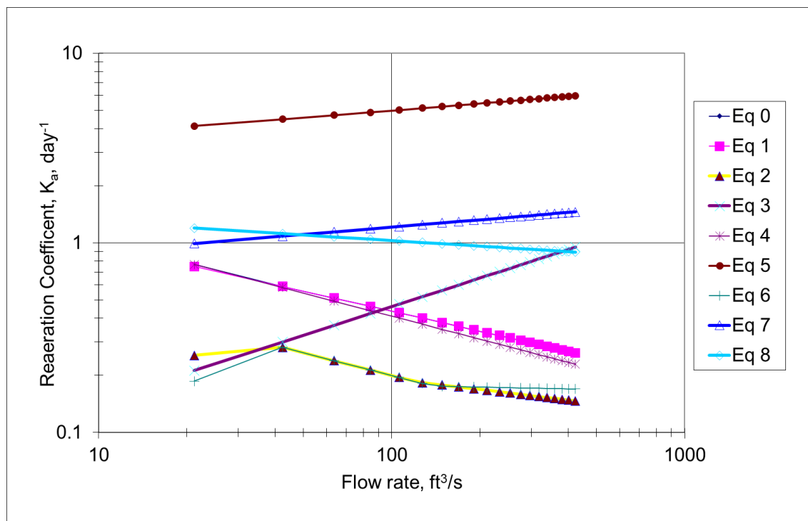
Figure 100. Reaeration coefficient as a function of flow rate.
