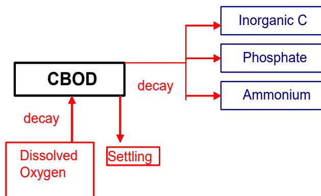
Figure 84. Internal flux between CBOD and other compartments in Version 3.6 and earlier.
