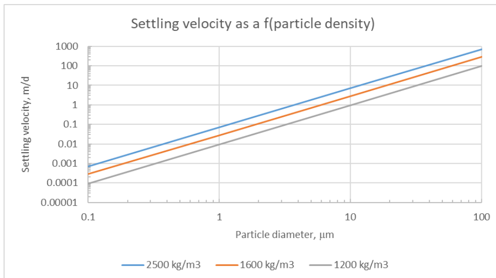
Figure 75. Typical settling of particles based on Stoke's Law based on particle diameter and density.
