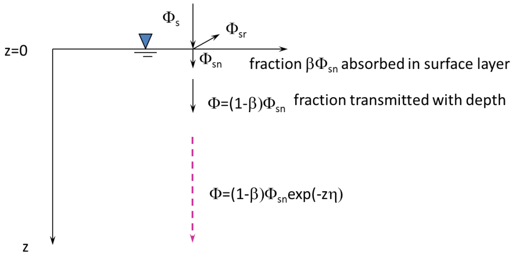
Figure 54. Short-wave solar penetration in a water body.
