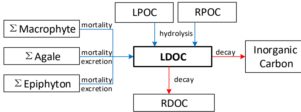
Figure 82. Kinetics of LDOC in the water column.
