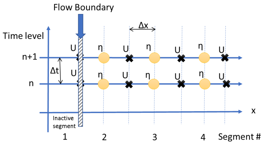
Figure 127. Flow boundary condition where velocities are specified on a boundary.
