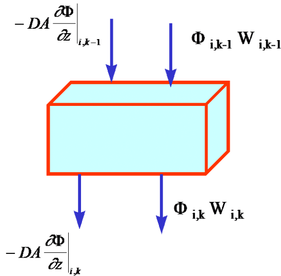
Figure 131. Vertical advective and diffusive transport.
