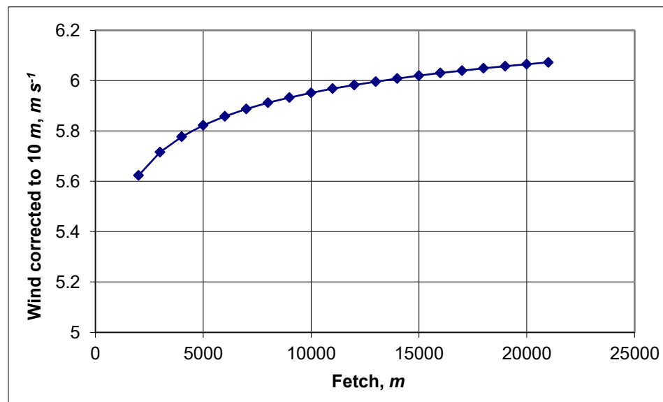
Figure 103. Wind speed of 5 m s^{-1} corrected to 10 m as a function of fetch.
