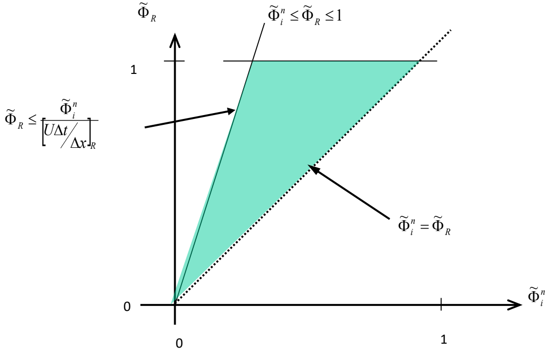
Figure 135. Definition sketch for monotonic solution domain.
