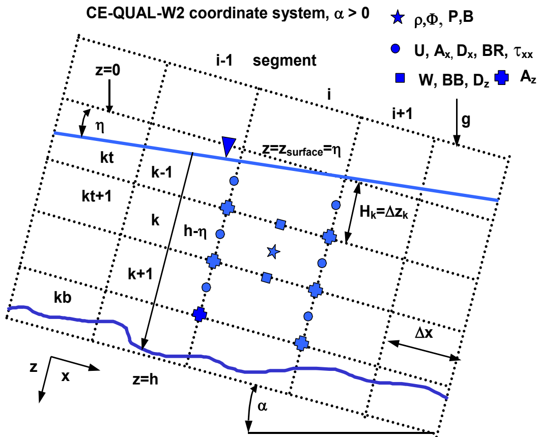
Figure 123. Computational grid variable definitions for arbitrary channel slope.
