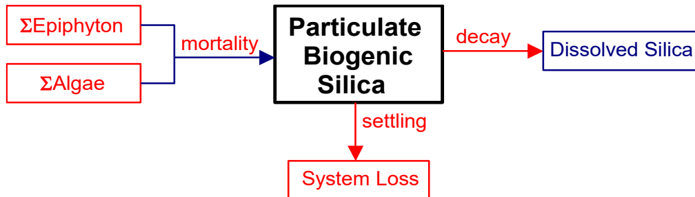
Figure 98. Internal flux between particulate biogenic silica and other compartments
