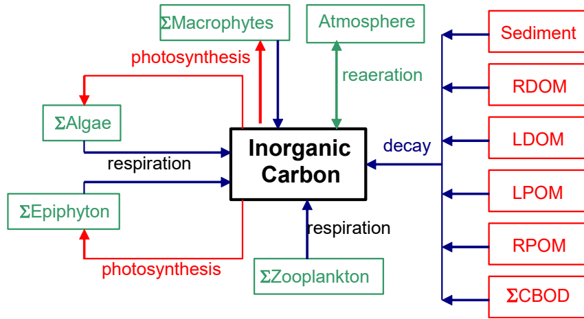
Figure 118. Internal flux between inorganic carbon and other compartments.
