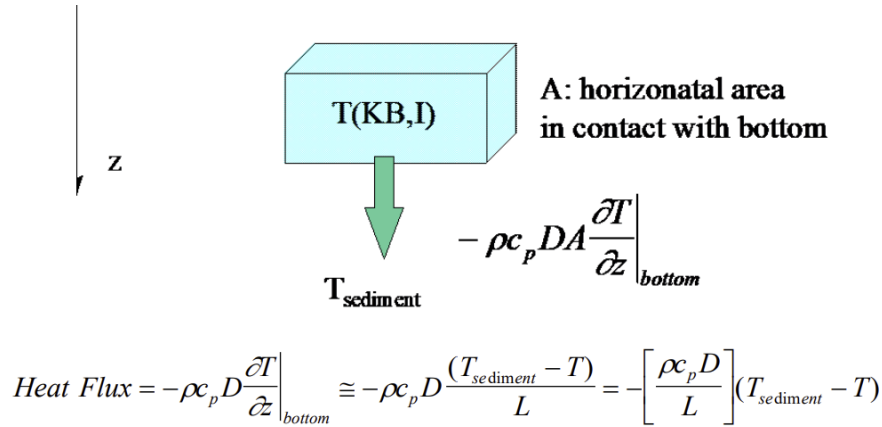
Figure 57. Schematic of sediment heat exchange.
