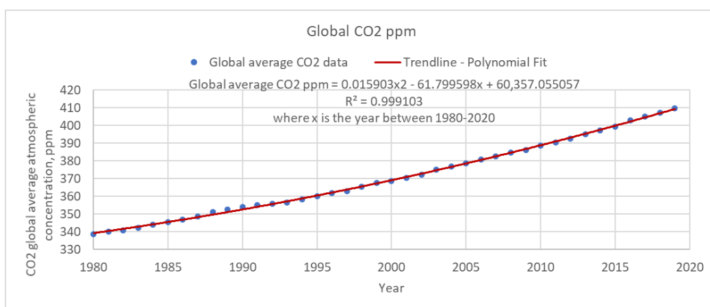
Figure 120. Global average CO2 gas concentration between 1980 and 2019 from NOAA/ESRL (2020) data.
