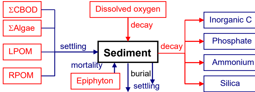
Figure 107. Internal flux between 1st-order sediment compartment and other compartments.
