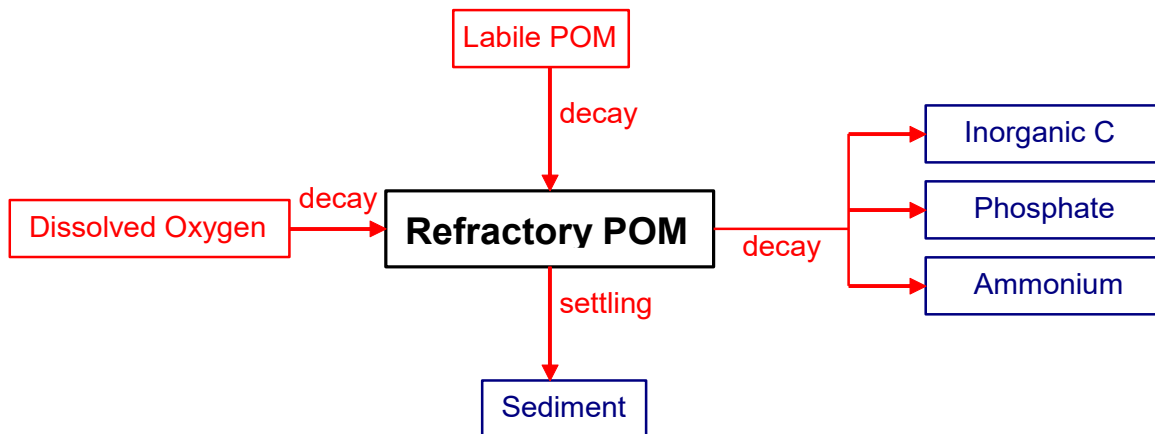
Figure 79. Internal flux between refractory POM and other compartments.
