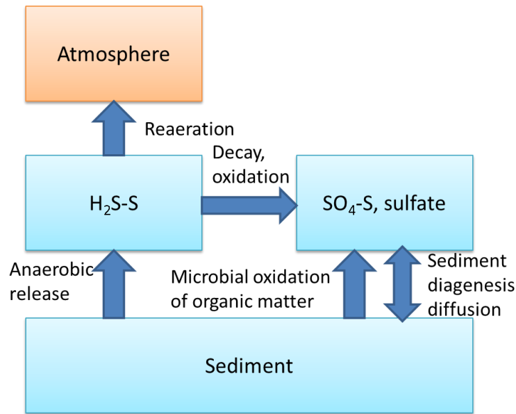
Figure 71. Sources and sinks for hydrogen sulfide and sulfate.
