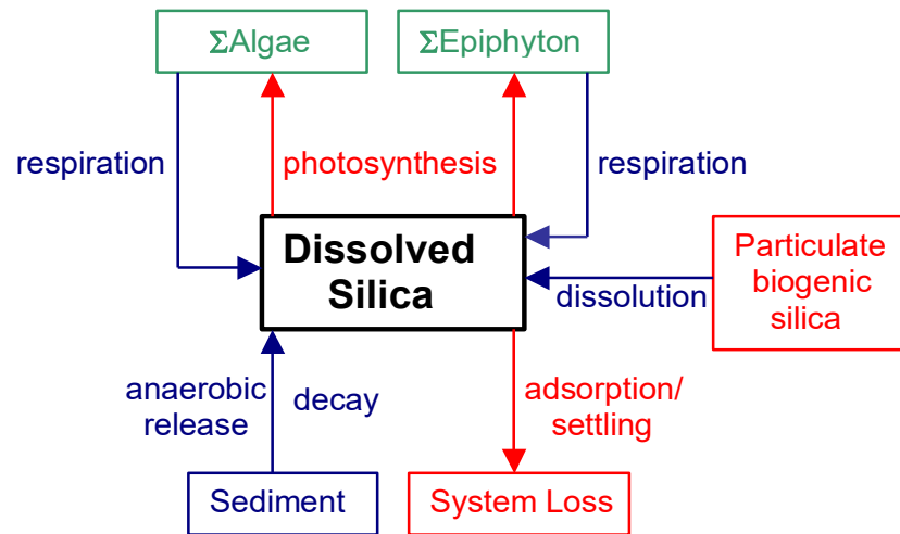
Figure 97. Internal flux between dissolved silica and other compartments.
