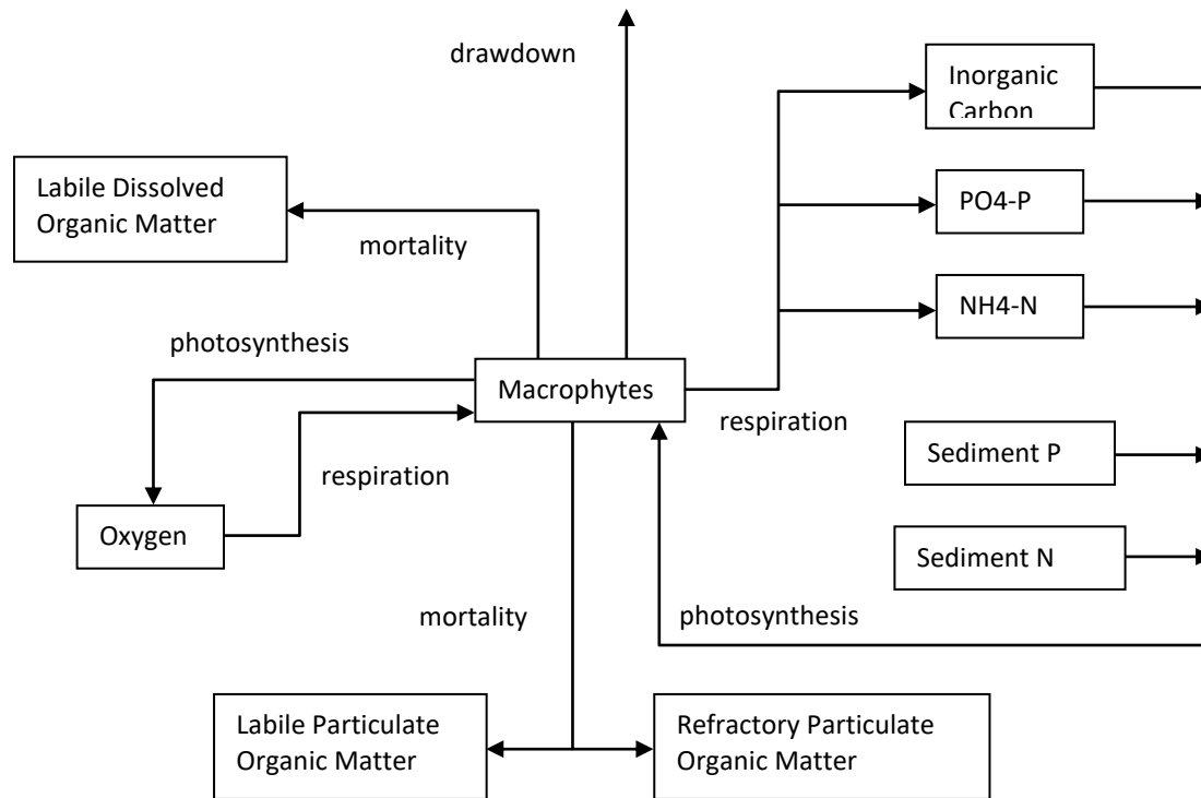
Figure 92. Nutrient fluxes for the macrophyte compartment in CE-QUAL-W2.
