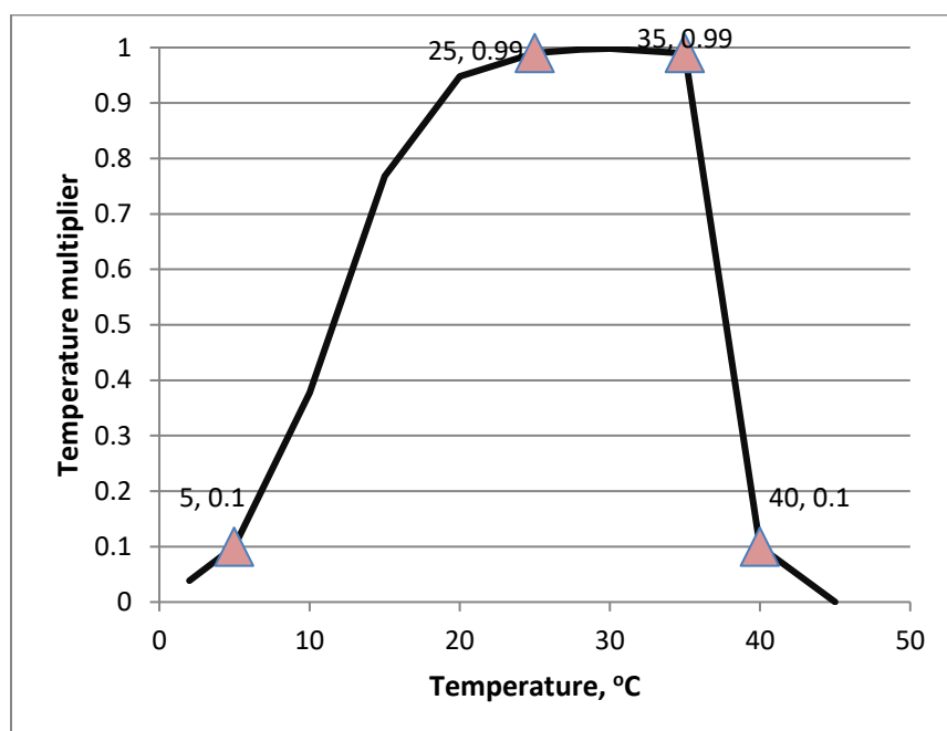
Figure 121. Temperature rate multiplier function.
