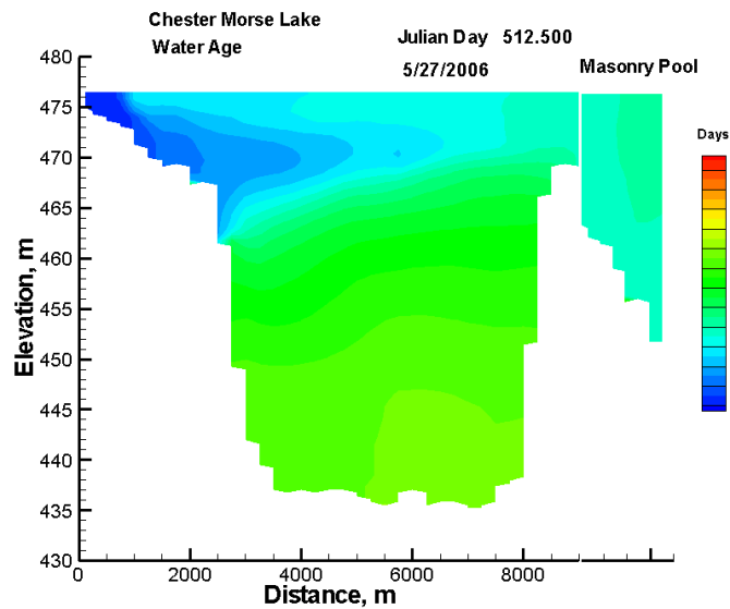
Figure 69. Water age in Chester Morse Lake, WA.
