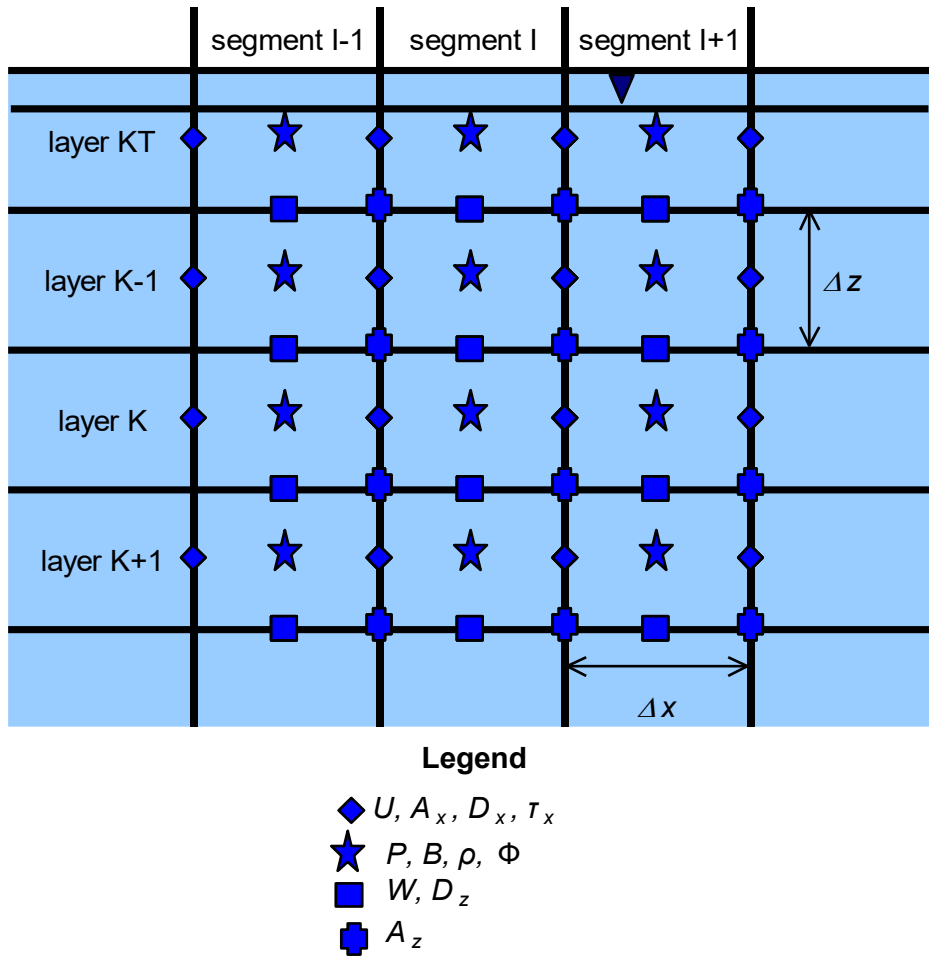
Figure 132. Variable locations in computational grid.
