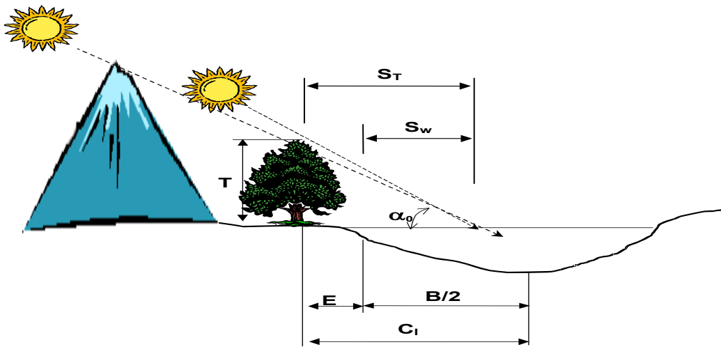
Figure 59. Schematic of topographic and vegetative shading, solar altitude ( \alpha_o ), and vegetation height ( T ) and their effect on shadow length.
