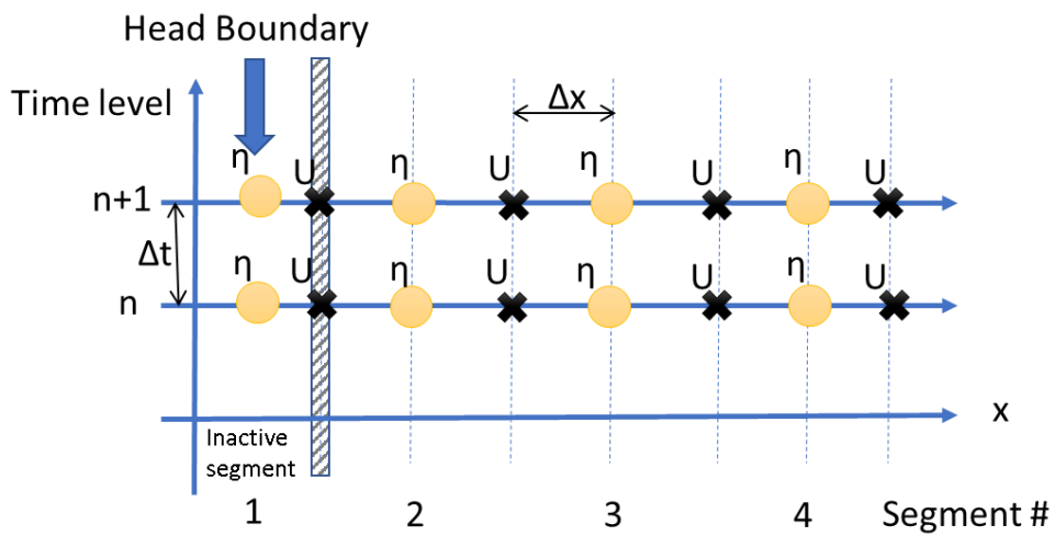
Figure 128. Head boundary condition for solution of momentum equation.
