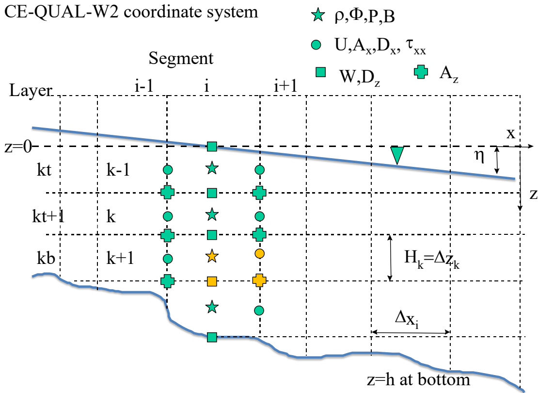
Figure 122. Computational grid variable definitions for no channel slope.
