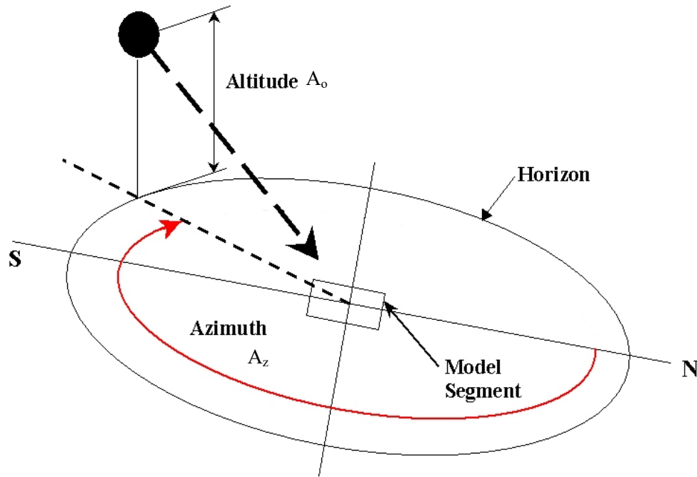
Figure 58. Schematic of solar altitude, A_o , and azimuth, A_z .
