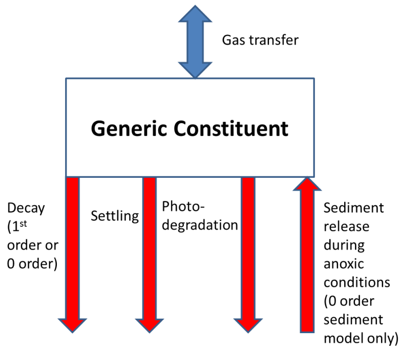
Figure 63. Internal flux for generic constituent compartment.
