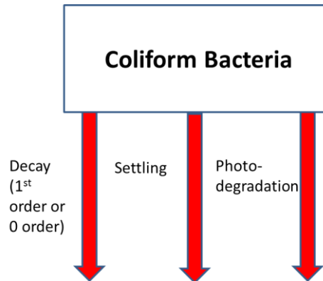
Figure 64. Internal flux for coliform bacteria.
