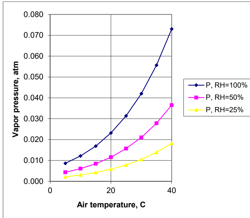
Figure 67. Vapor pressure as a function of air temperature and relative humidity.
