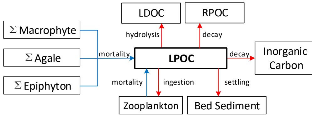
Figure 80. Kinetics of LPOC in the water column.
