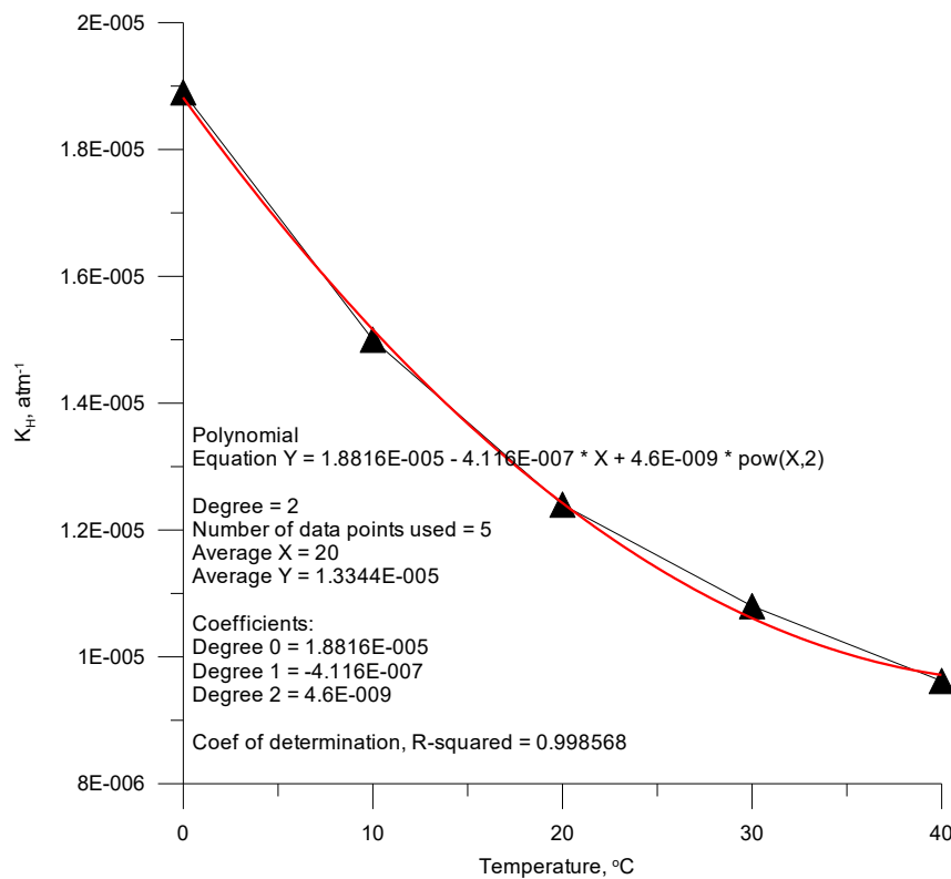
Figure 66. Henry's Law constant dependence on temperature.
