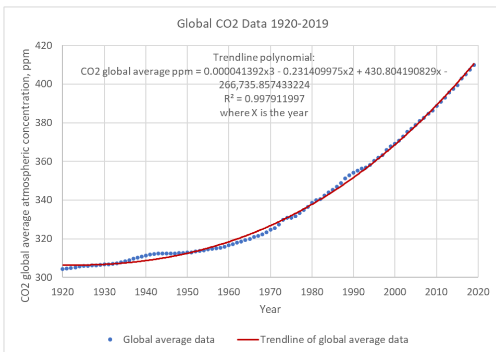
Figure 119. Global average CO2 gas concentration from 1920 to 2019 from NOAA/ESRL (2020) data.
