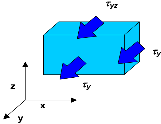
Figure 4. Sketch of turbulent shear stresses in y-direction.
