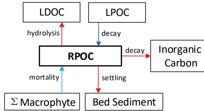
Figure 81. Kinetics of RPOC in the water column.
