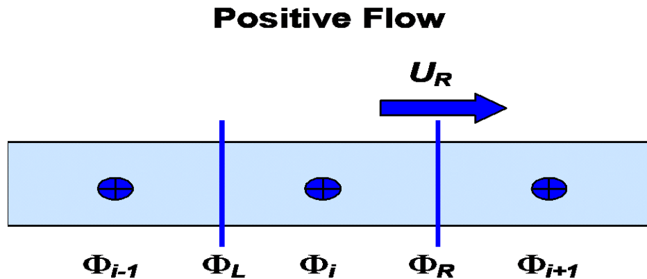
Figure 133. ULTIMATE schematization for positive flow.
