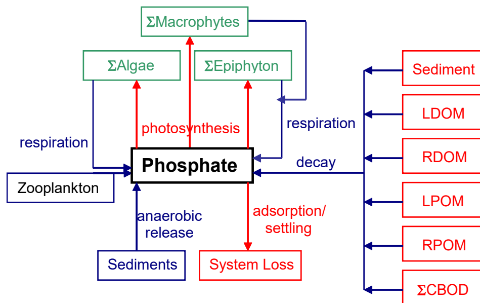
Figure 94. Internal flux between phosphorus and other compartments.
