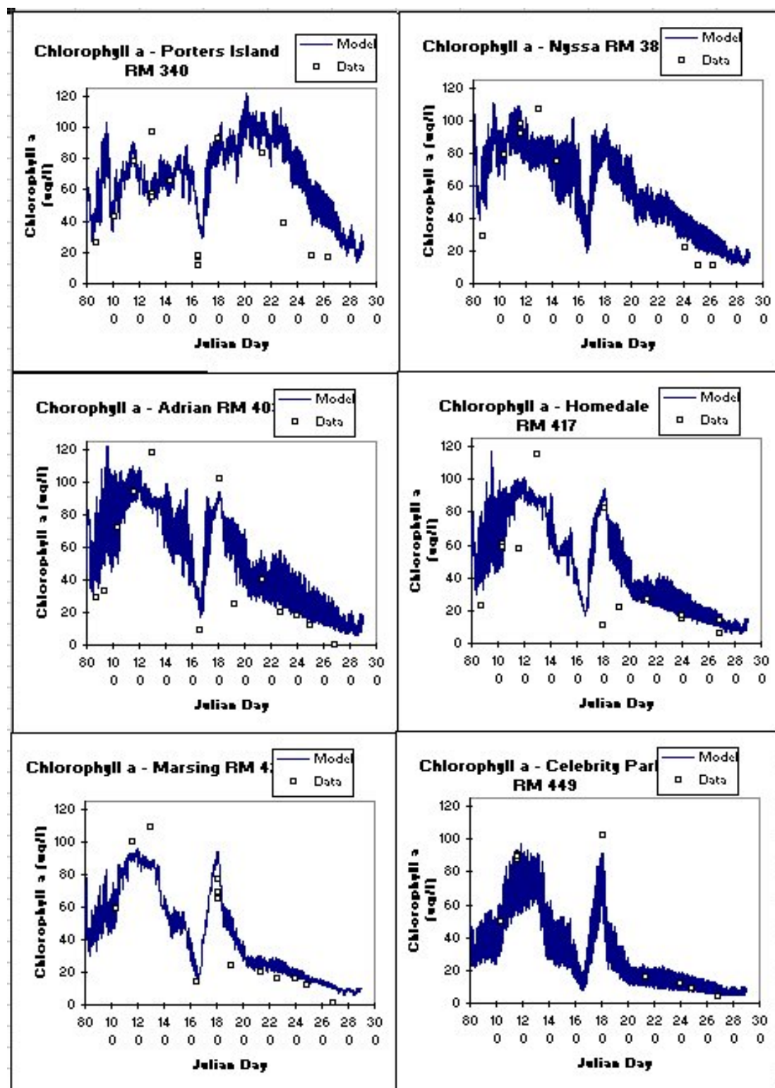
Figure 103. Snake River computed versus observed chlorophyll a at six stations.
