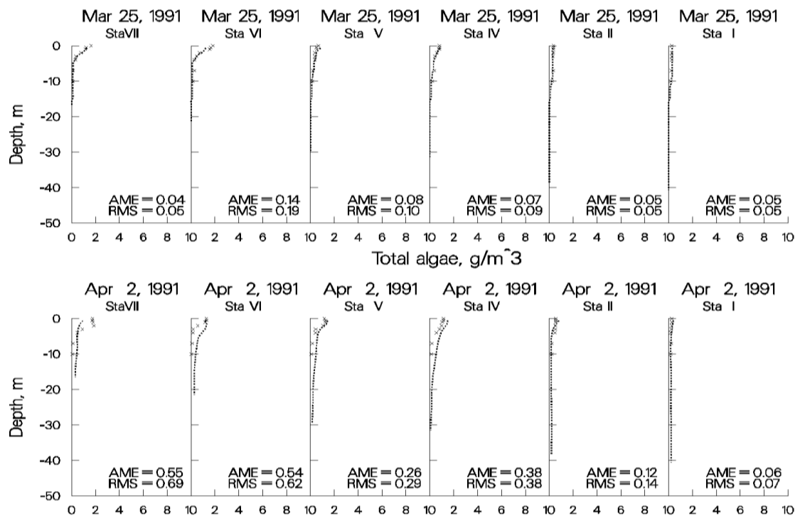
Figure 66. Rimov Reservoir computed vs. observed phytoplankton biomass.
