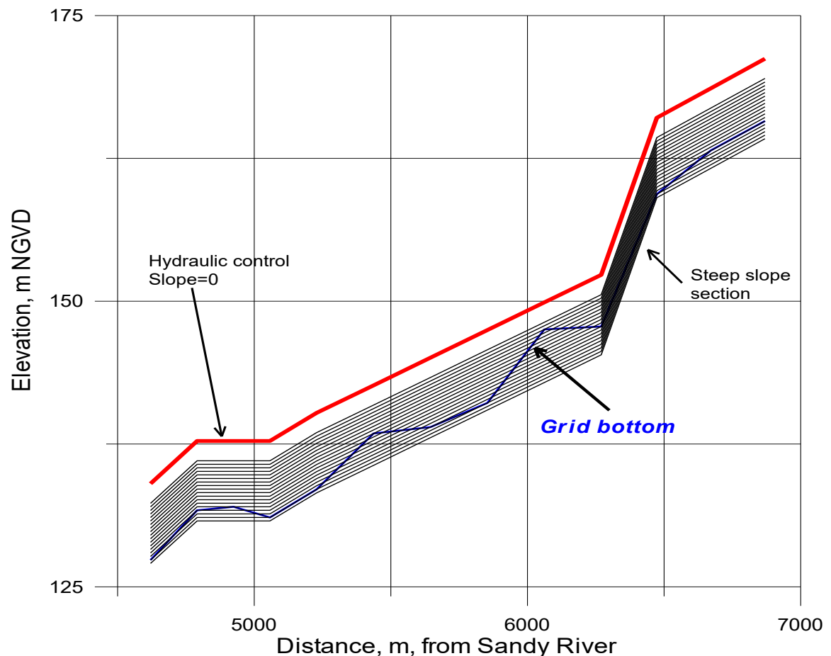
Figure 93. Vertical grid for W2 model of Bull Run Lower River.
