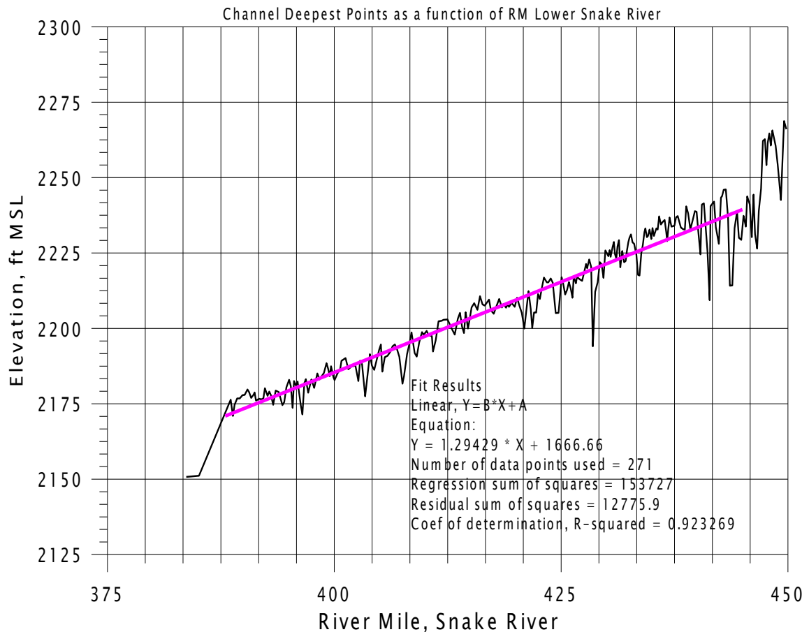
Figure 91. Snake River channel slope determination.
