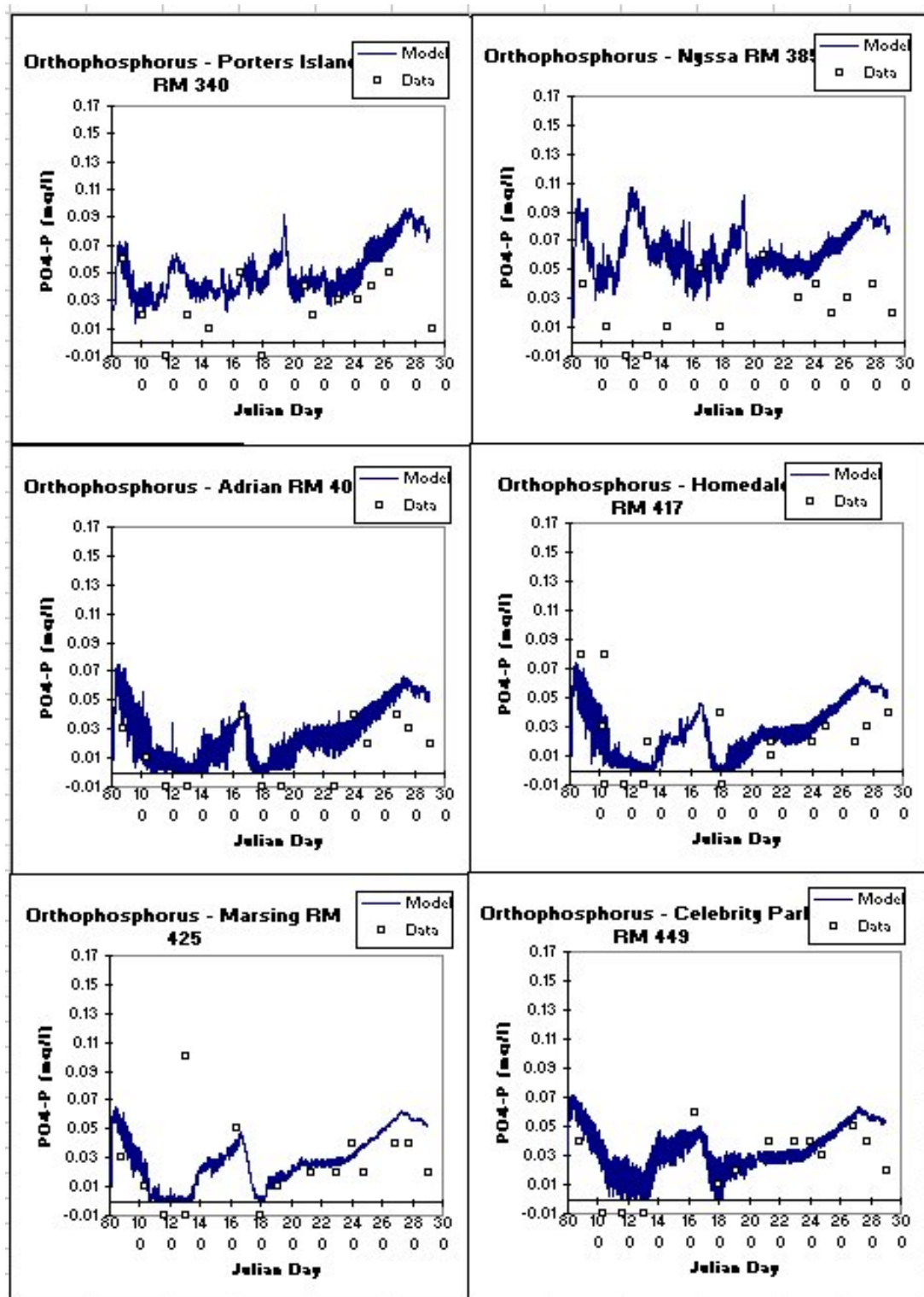
Figure 101. Snake River computed versus observed orthophosphorus at six stations.
