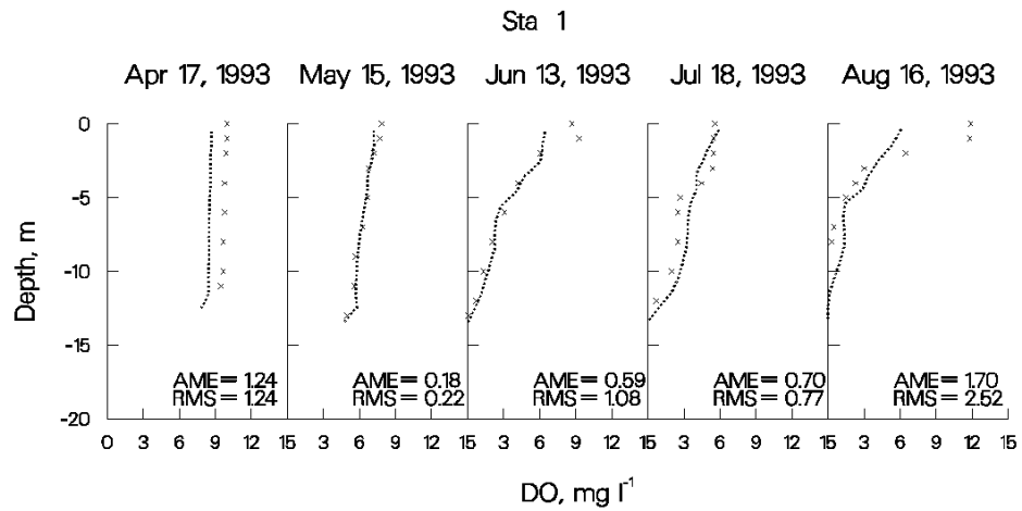
Figure 57. Neely Henry Reservoir computed vs. observed DO.
