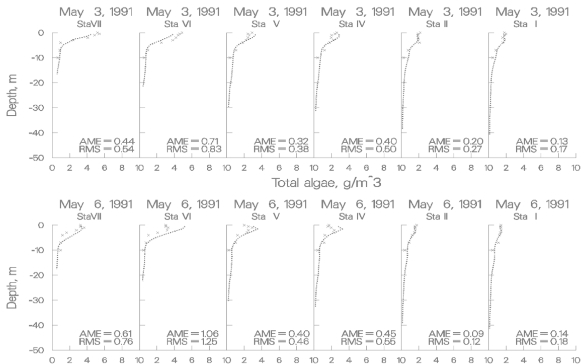
Figure 77. Rimov Reservoir computed vs. observed phytoplankton with wind rotated 90°.
