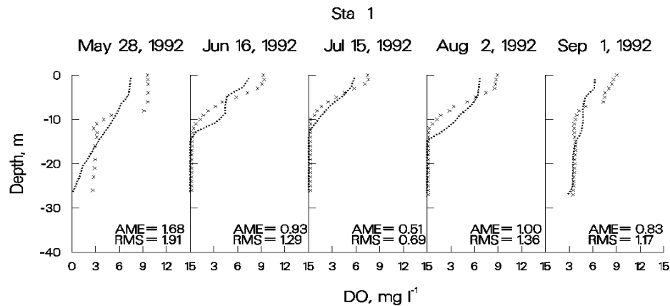
Figure 65. Walter F. George Reservoir computed vs. observed DO.
