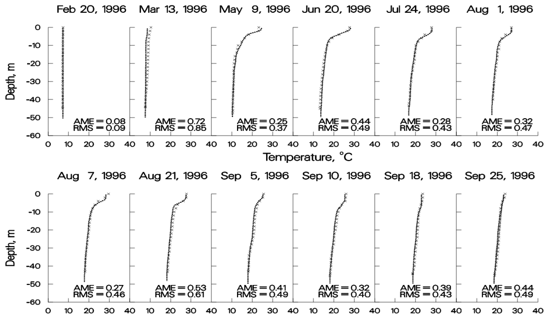
Figure 45. 1996 Richard B. Russell computed versus observed temperatures.
