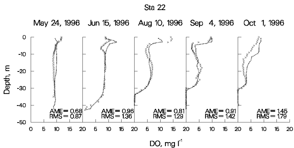
Figure 60. Rimov Reservoir computed vs. observed DO.
