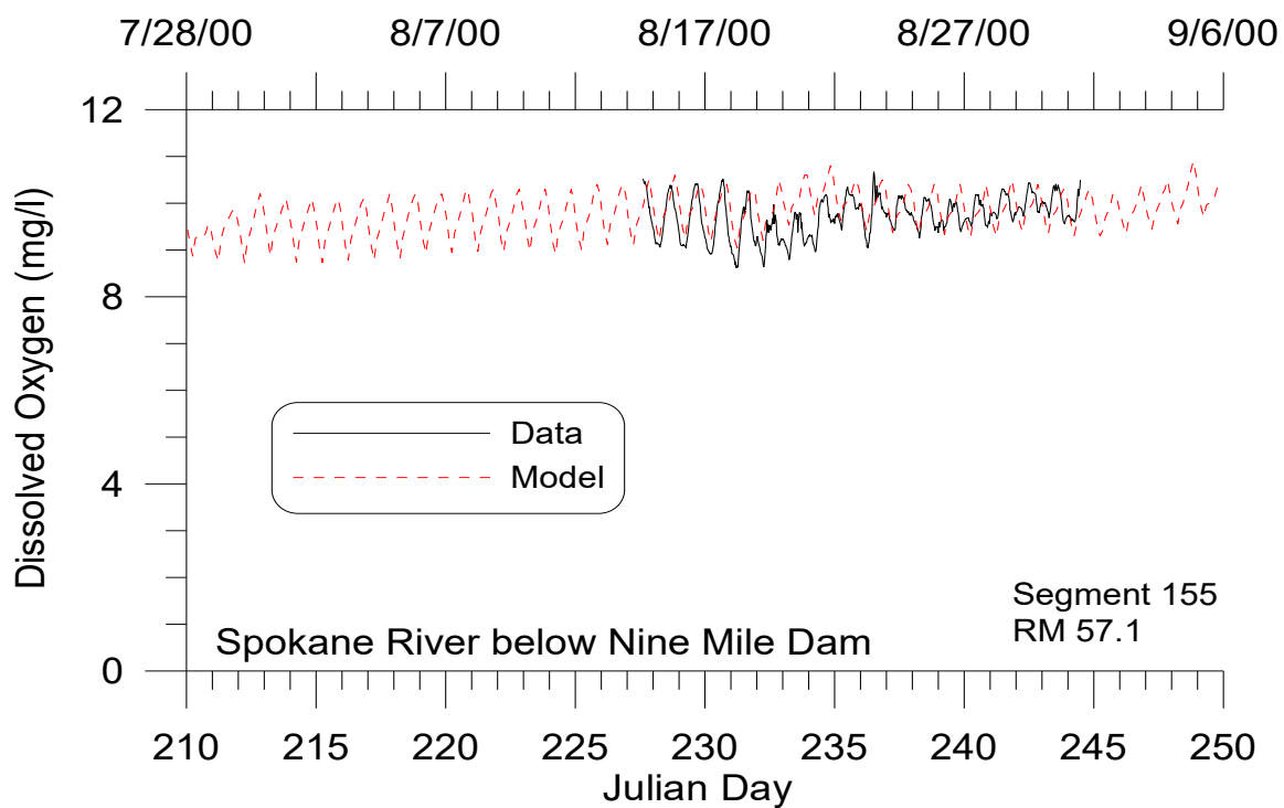
Figure 106. Spokane River computed versus observed dissolved oxygen below Nine Mile Dam.
