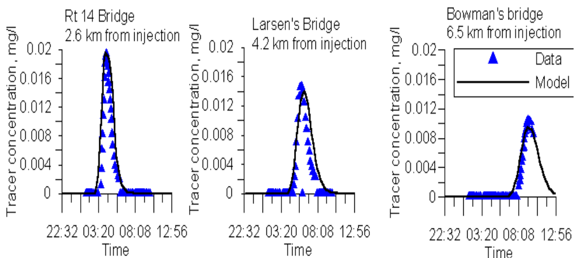
Figure 94. Bull Run River computed versus observed tracer at three stations progressing downstream.
