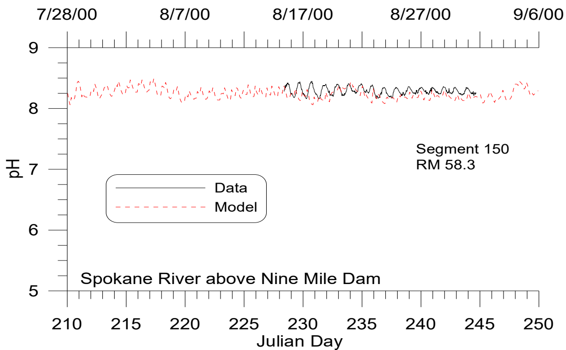
Figure 107. Spokane River computed versus observed pH upstream of Nine Mile Dam.
