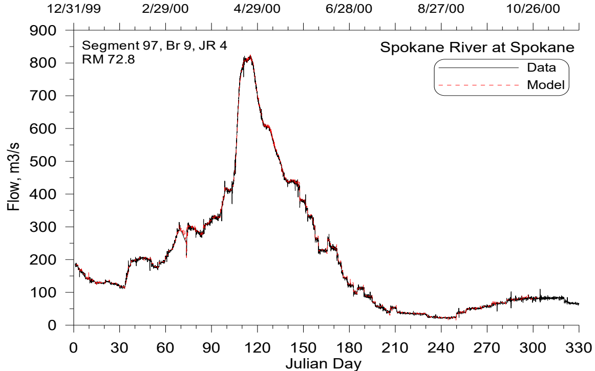
Figure 96. Spokane River computed versus observed flows at the city of Spokane.
