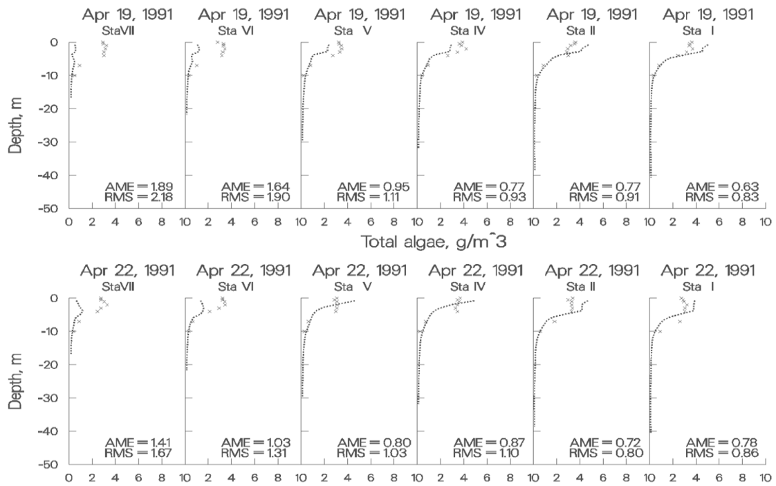
Figure 81. Rimov Reservoir computed vs. observed phytoplankton with no inflowing phytoplankton.
