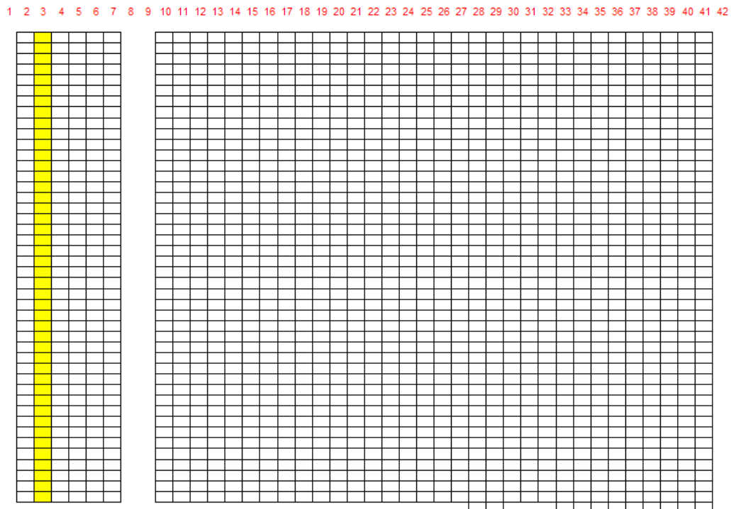
Figure 35. Model vertical layers for Spokane River model.
