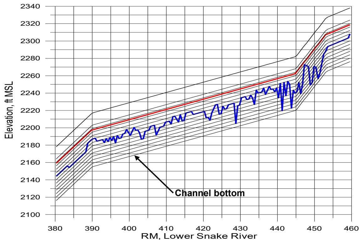
Figure 90. Channel vertical grid where every slope change is a new branch.
