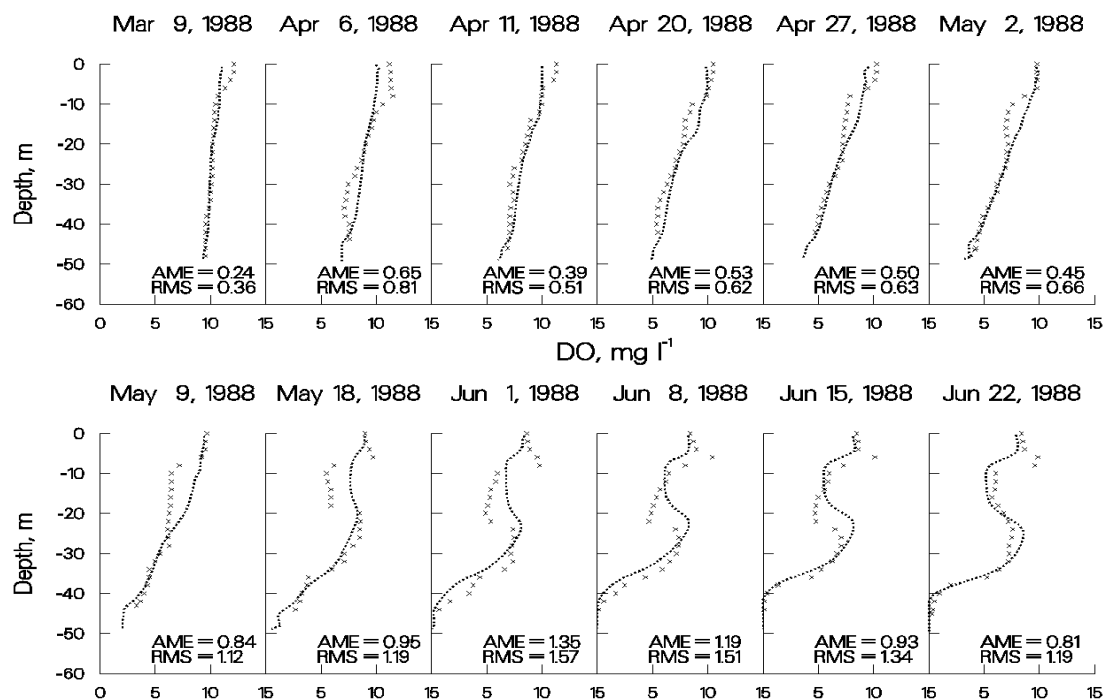
Figure 54. Richard B. Russell Reservoir computed vs. observed DO, March through June, 1988.
