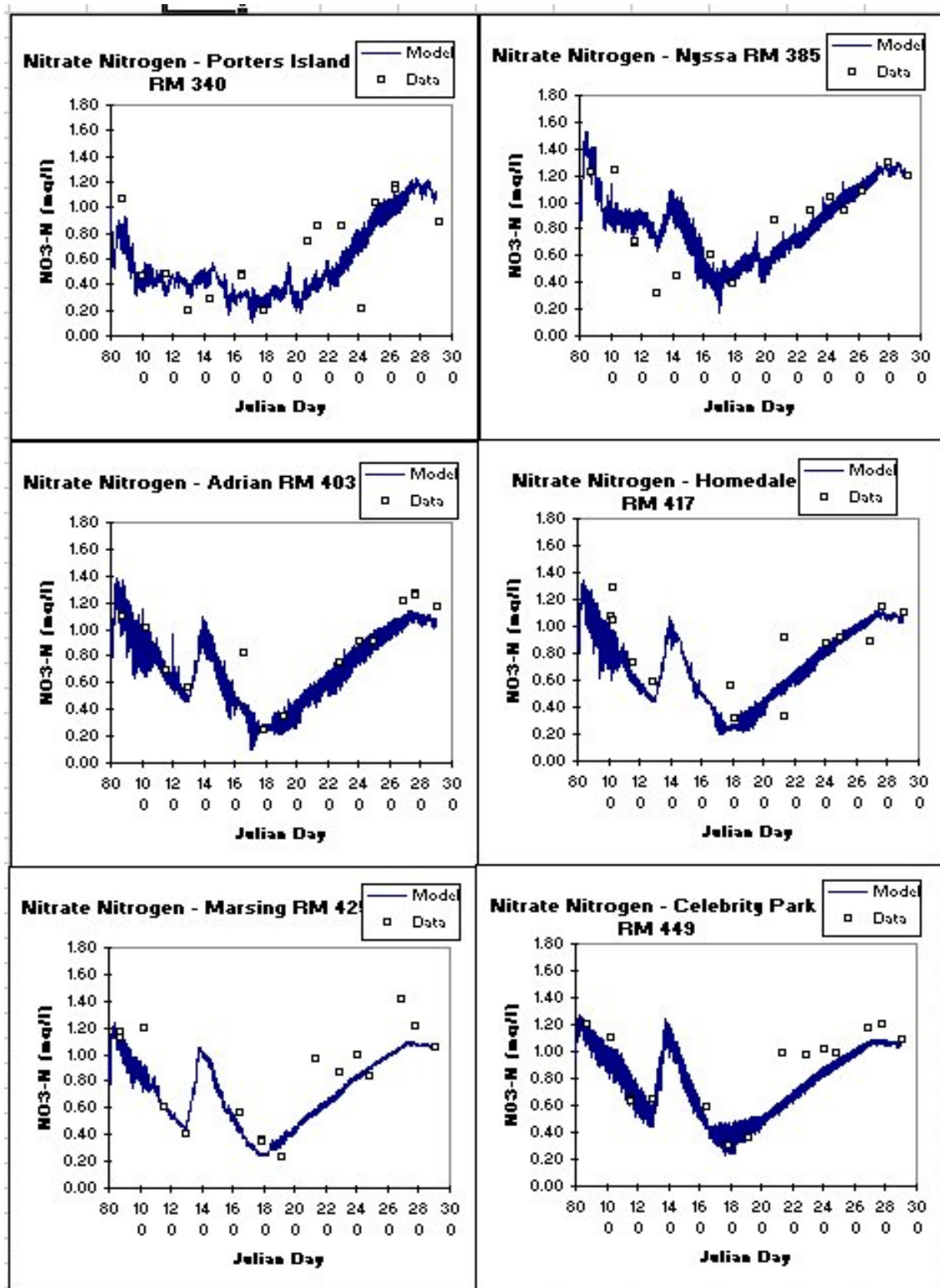
Figure 102. Snake River computed versus observed nitrate-nitrite at six stations.
