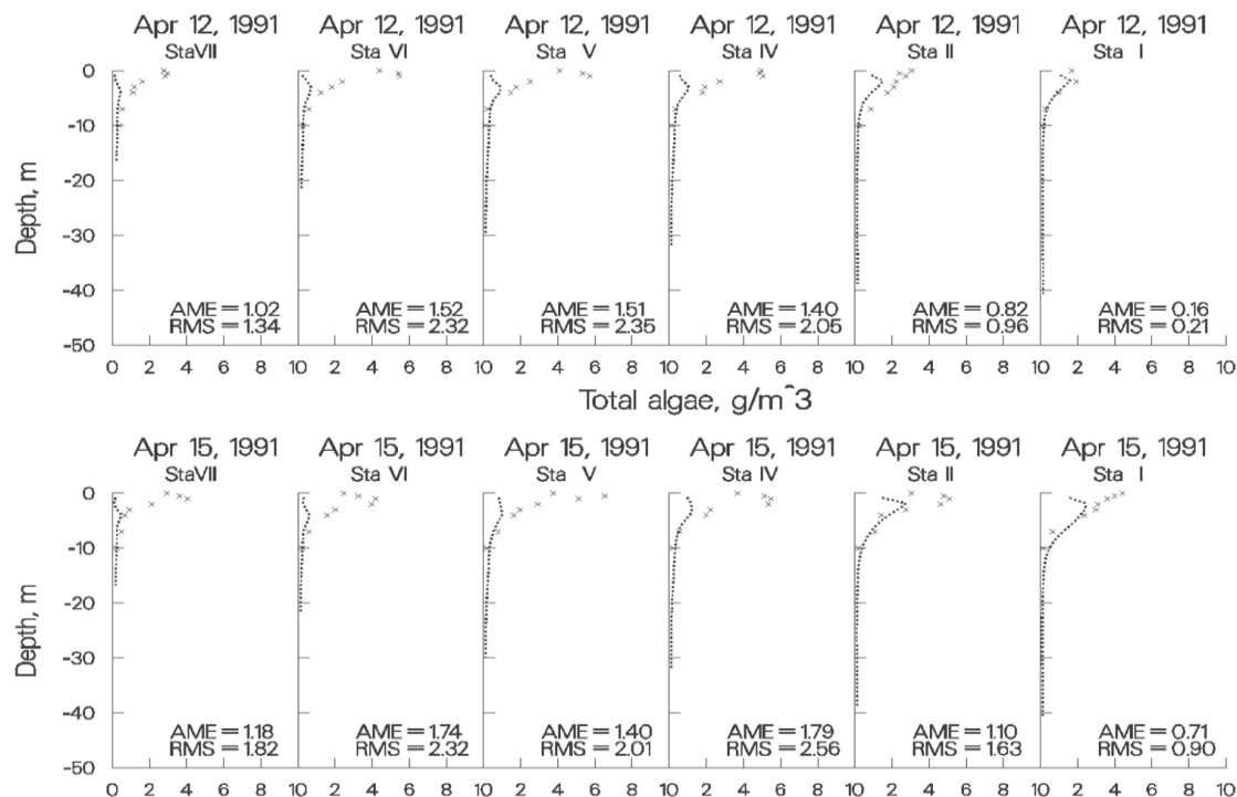
Figure 80. Rimov Reservoir computed vs. observed phytoplankton with no inflowing phytoplankton.
