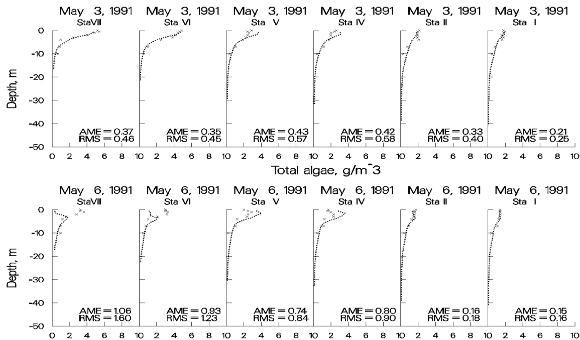
Figure 83. Rimov Reservoir computed vs. observed phytoplankton with no inflowing phytoplankton.
