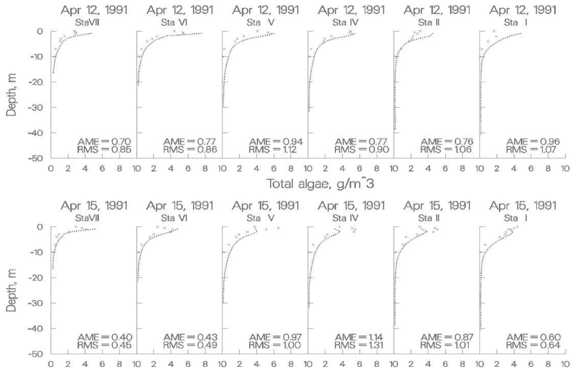
Figure 68. Rimov Reservoir computed vs. observed phytoplankton biomass.
