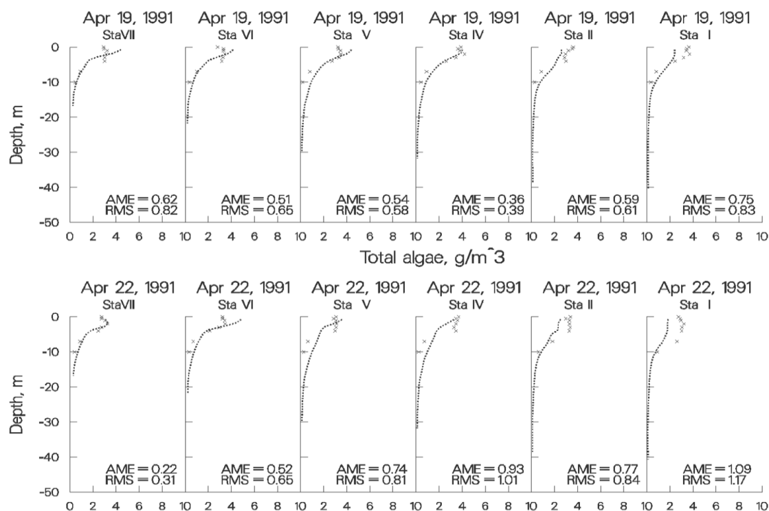
Figure 69. Rimov Reservoir computed vs. observed phytoplankton biomass.
