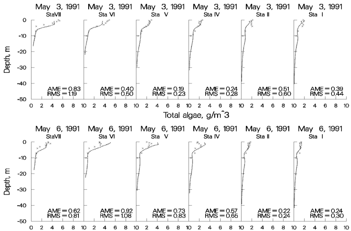
Figure 71. Rimov Reservoir computed vs. observed phytoplankton biomass.
