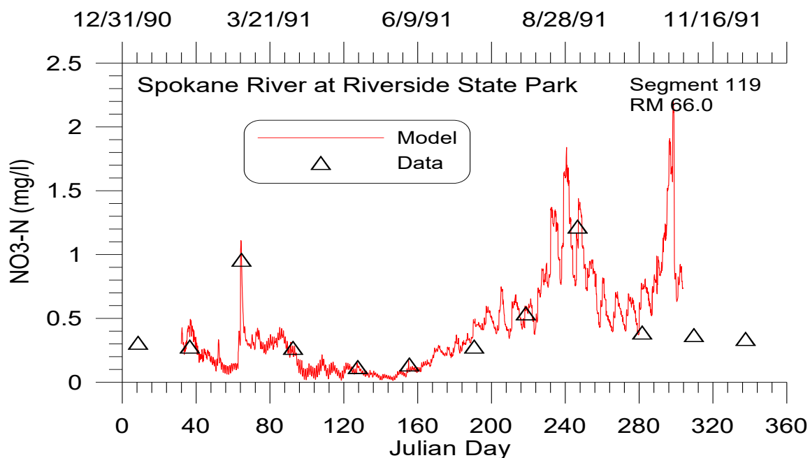
Figure 108. Spokane River computed versus observed nitrate-nitrite at Riverside State Park.
