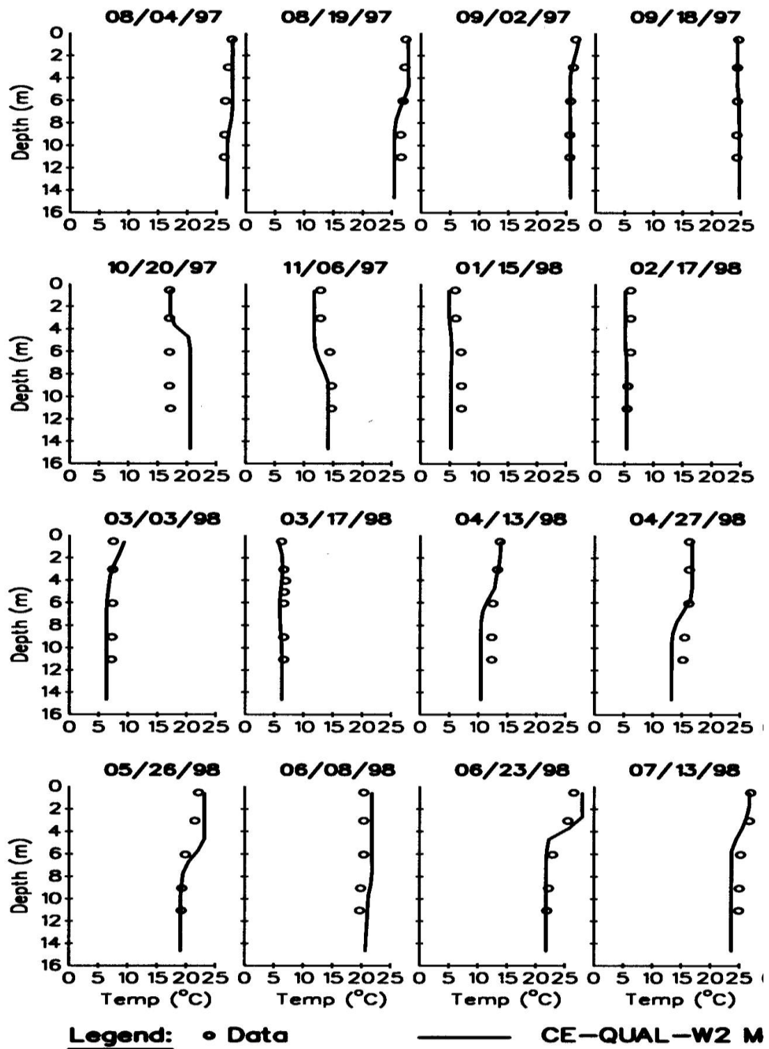
Figure 87. Patuxent River computed versus observed vertical temperature distributions.
