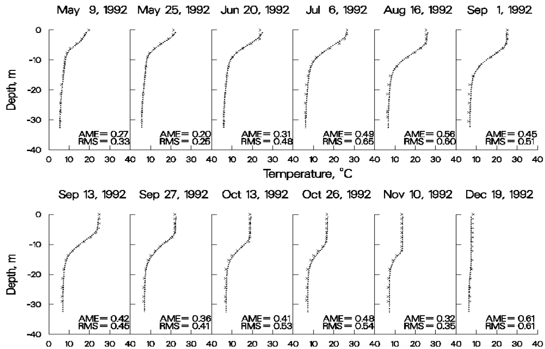
Figure 46. Paintsville Reservoir computed versus observed temperatures.
