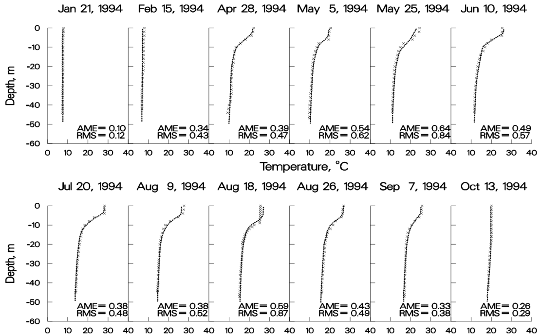
Figure 44. 1994 Richard B. Russell computed versus observed temperatures.
