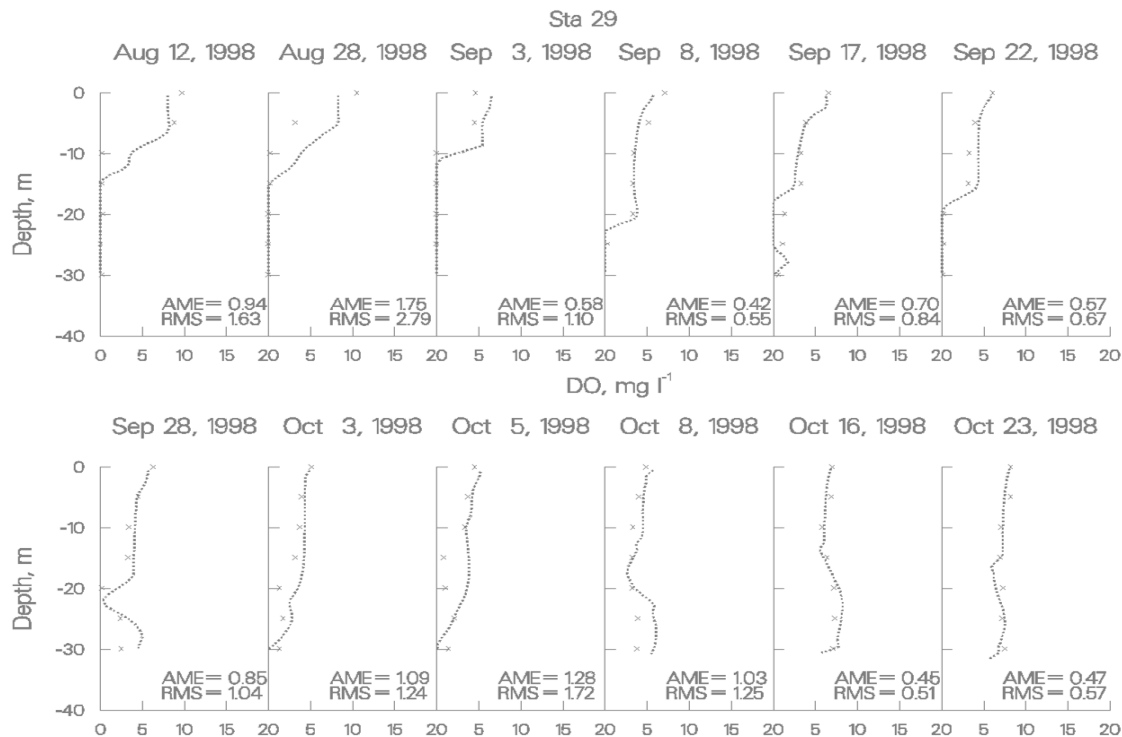
Figure 62. Shepaug Reservoir computed vs. observed DO.
