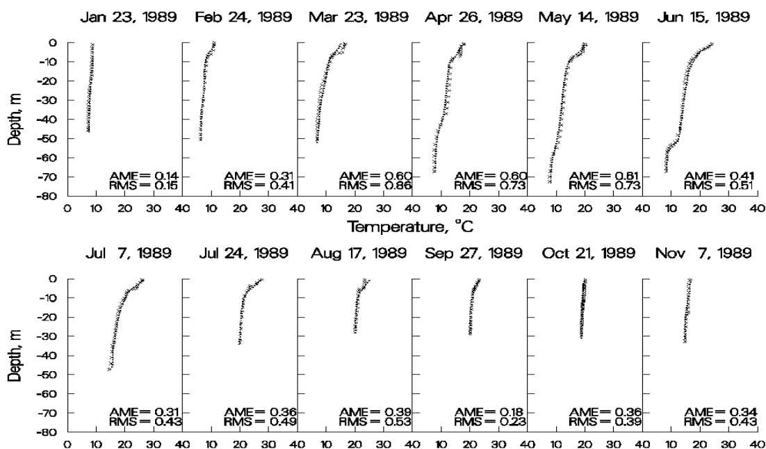
Figure 39. 1989 Pineflat Reservoir computed versus observed temperatures.
