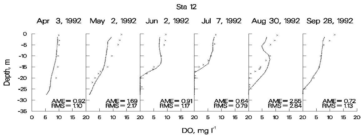
Figure 52. C.J. Strike Reservoir computed vs. observed DO.
