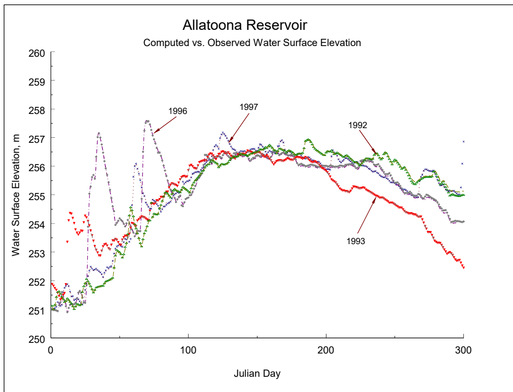
Figure 38. Allatoona Reservoir computed (lines) vs. observed (symbols) water surface elevations for 1992, 1993, 1996, and 1997.
