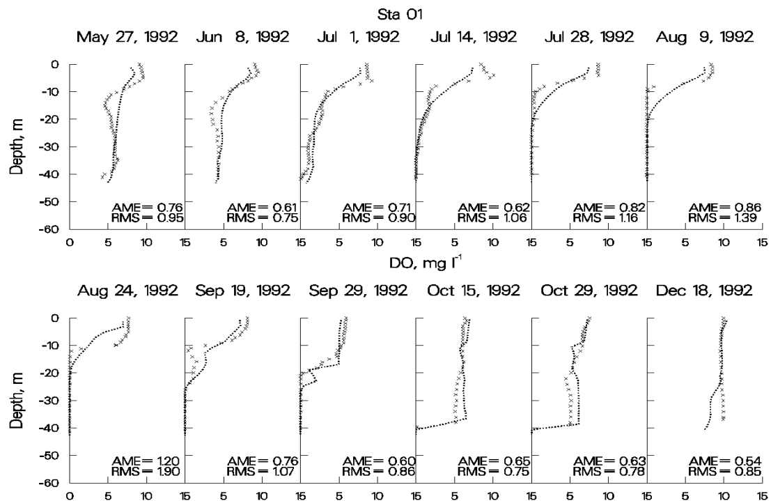
Figure 50. Allatoona Reservoir computed vs. observed DO.
