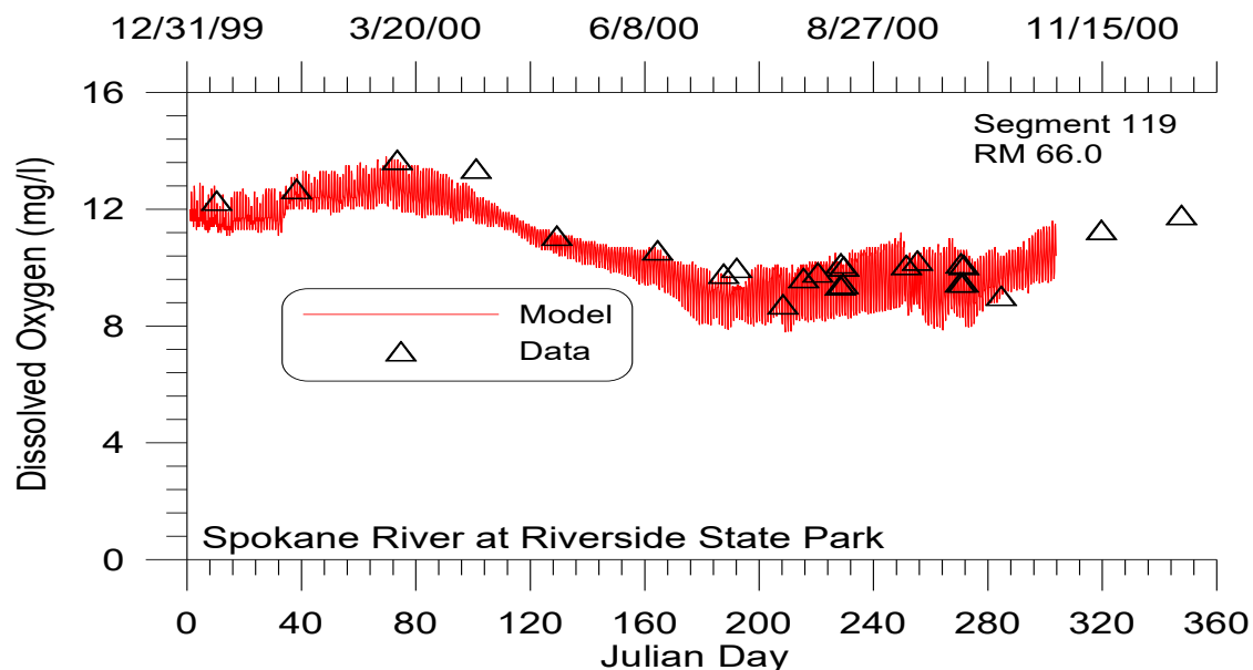
Figure 105. Spokane River computed versus observed dissolved oxygen at Riverside State Park.
