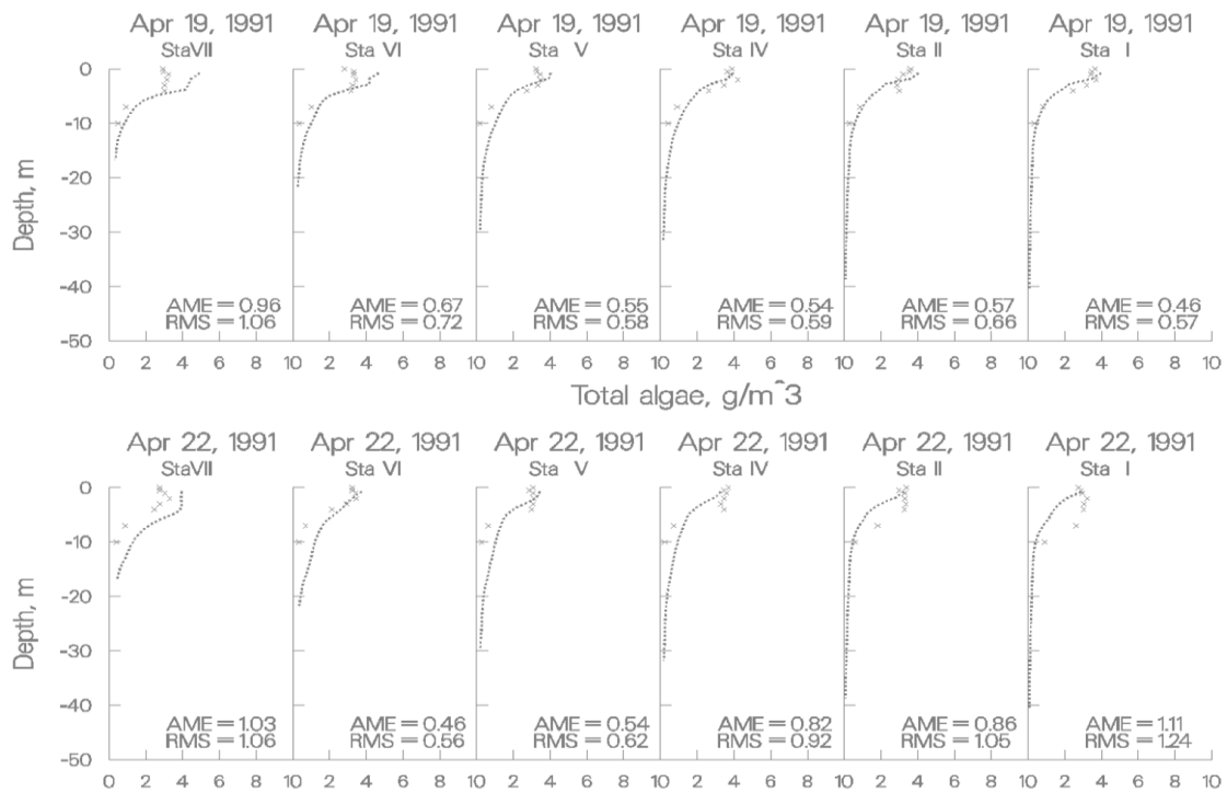
Figure 75. Rimov Reservoir computed vs. observed phytoplankton with wind rotated 90°.
