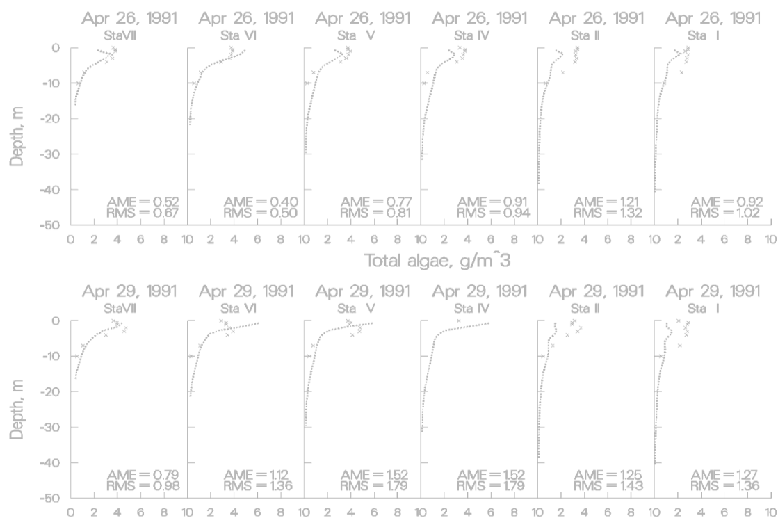
Figure 70. Rimov Reservoir computed vs. observed phytoplankton biomass.
