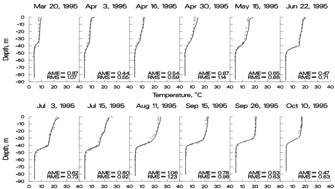
Figure 48. 1995 Brownlee Reservoir computed versus observed temperatures.
