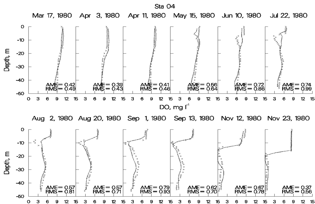
Figure 53. DeGray Reservoir computed vs. observed DO.
