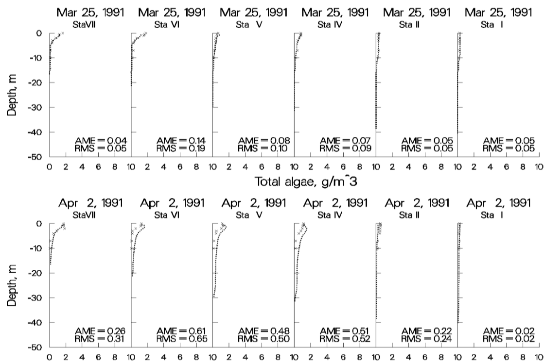
Figure 72. Rimov Reservoir computed vs. observed phytoplankton with wind rotated 90°.
