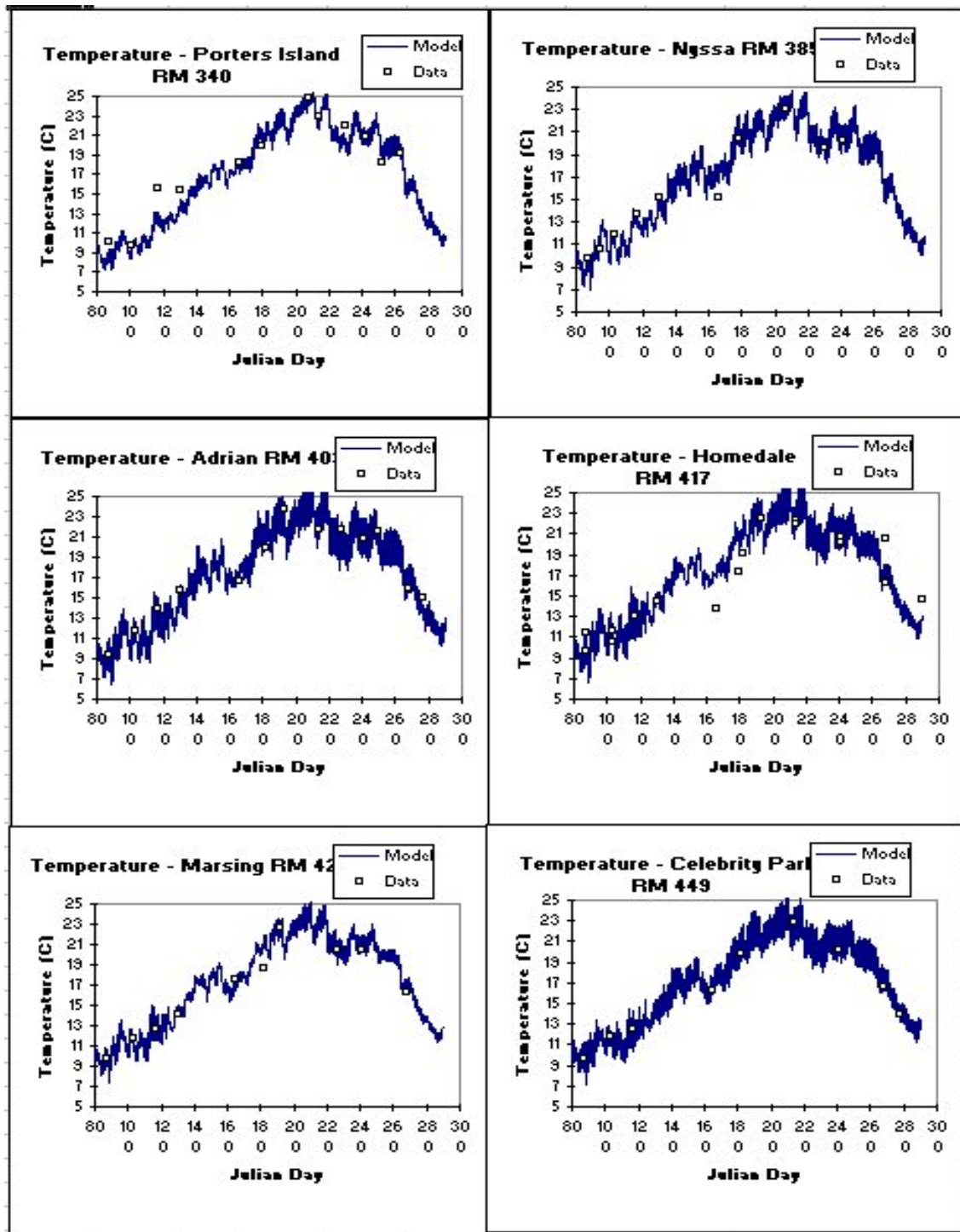
Figure 97. Snake River computed versus observed temperature at six stations.
