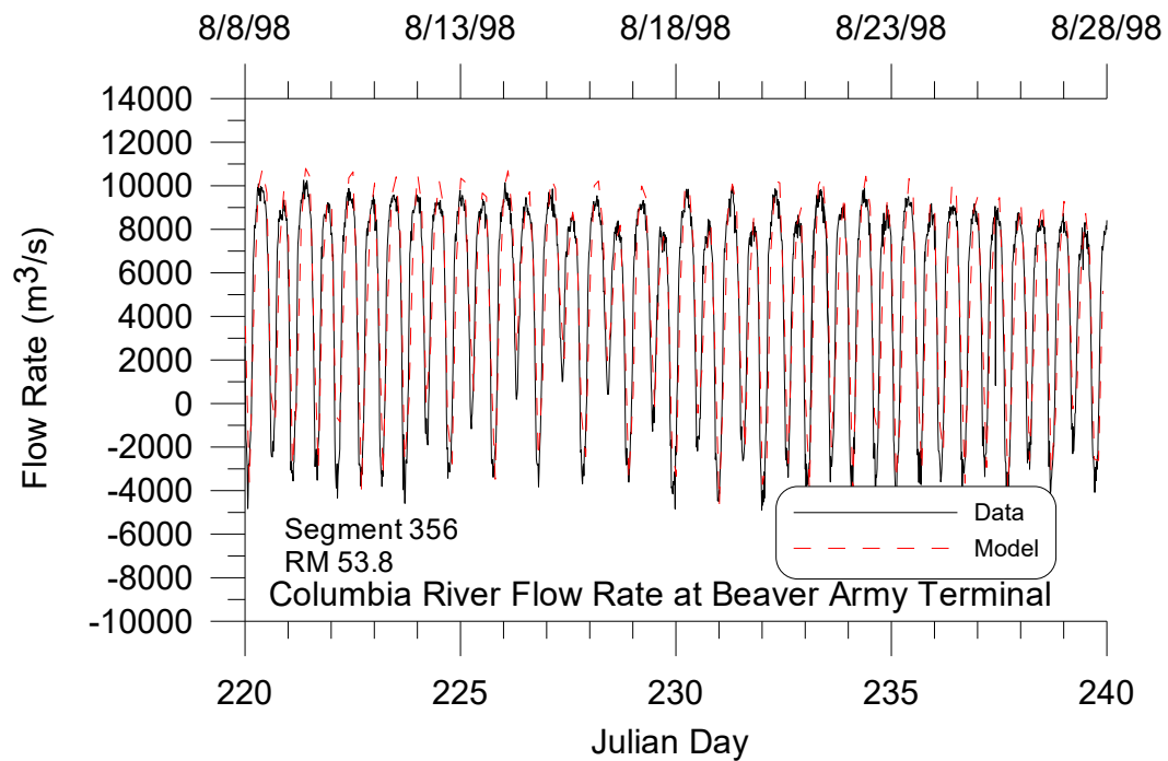
Figure 85. Model flow predictions versus data for a 20-day period during 1998 at Beaver Army Terminal near Quincy, OR.
