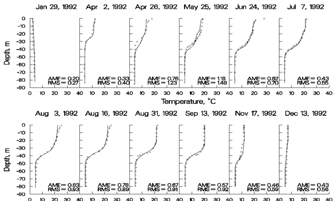
Figure 47. 1992 Brownlee Reservoir computed versus observed temperatures.
