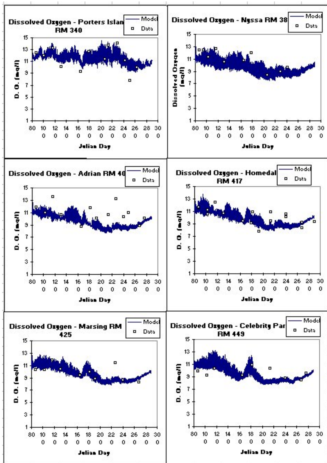
Figure 100. Snake River computed versus observed dissolved oxygen at six stations.
