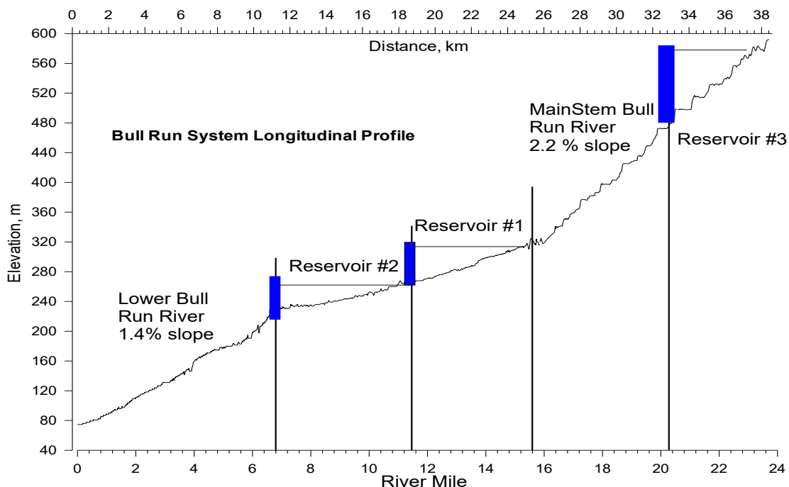
Figure 92. Channel slope for the Bull Run system.
