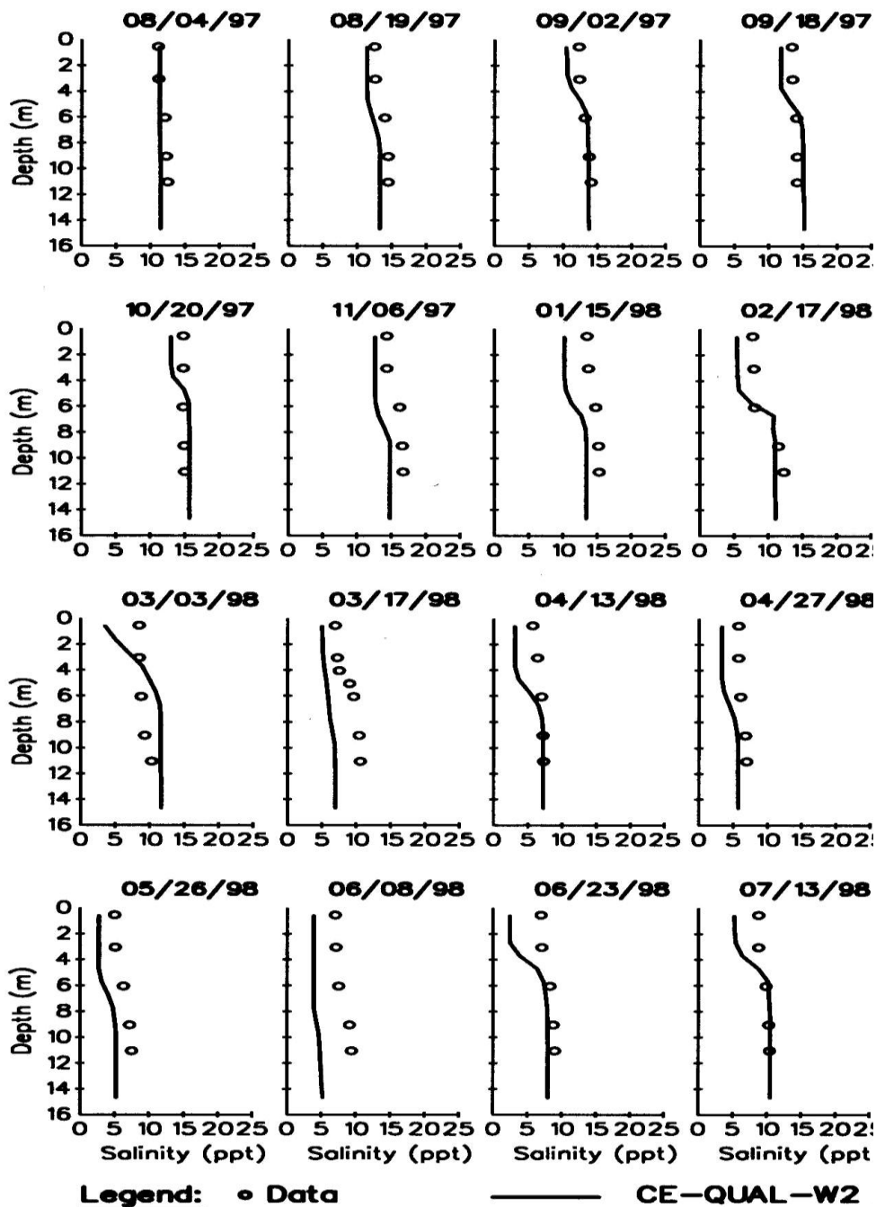
Figure 86. Patuxent River computed versus observed vertical salinity distributions.
