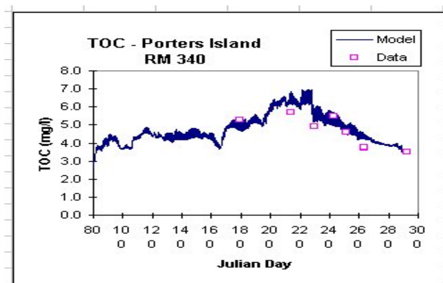
Figure 104. Snake River computed versus total organic carbon.
