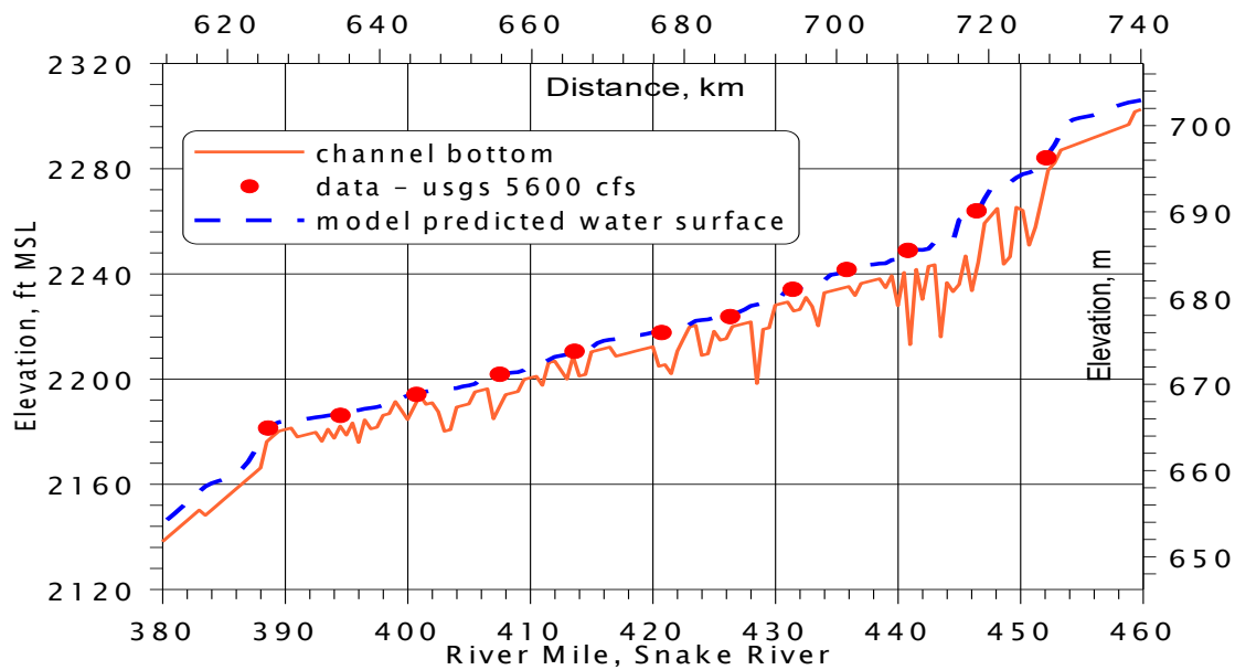
Figure 89. Snake River water level comparison between CE-QUAL-W2 V3 and USGS field data.
