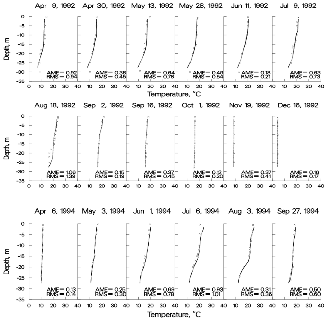
Figure 49. C.J. Strike Reservoir computed versus observed temperatures.
