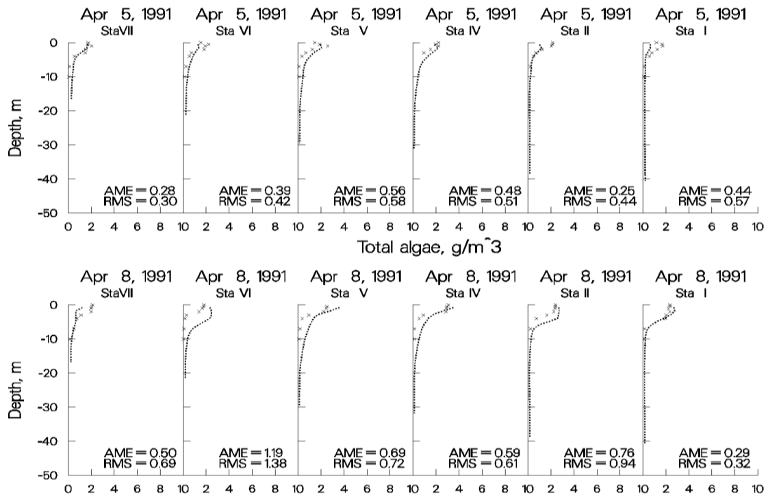
Figure 67. Rimov Reservoir computed vs. observed phytoplankton biomass.
