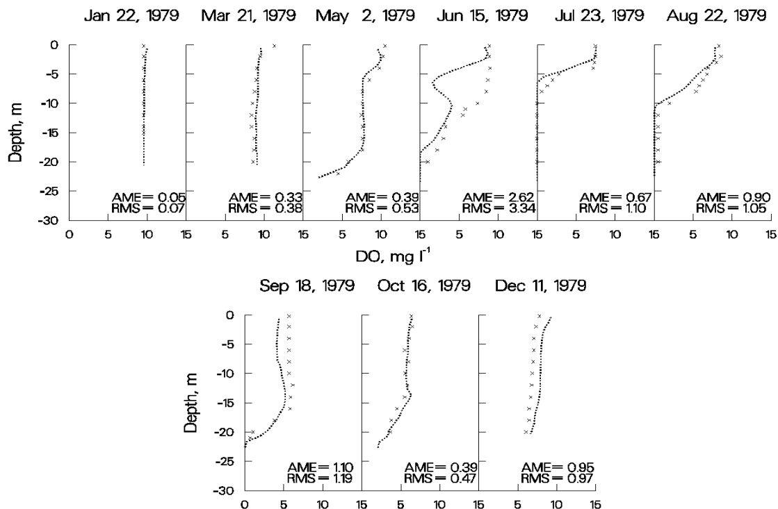
Figure 64. West Point Reservoir computed vs. observed DO.
