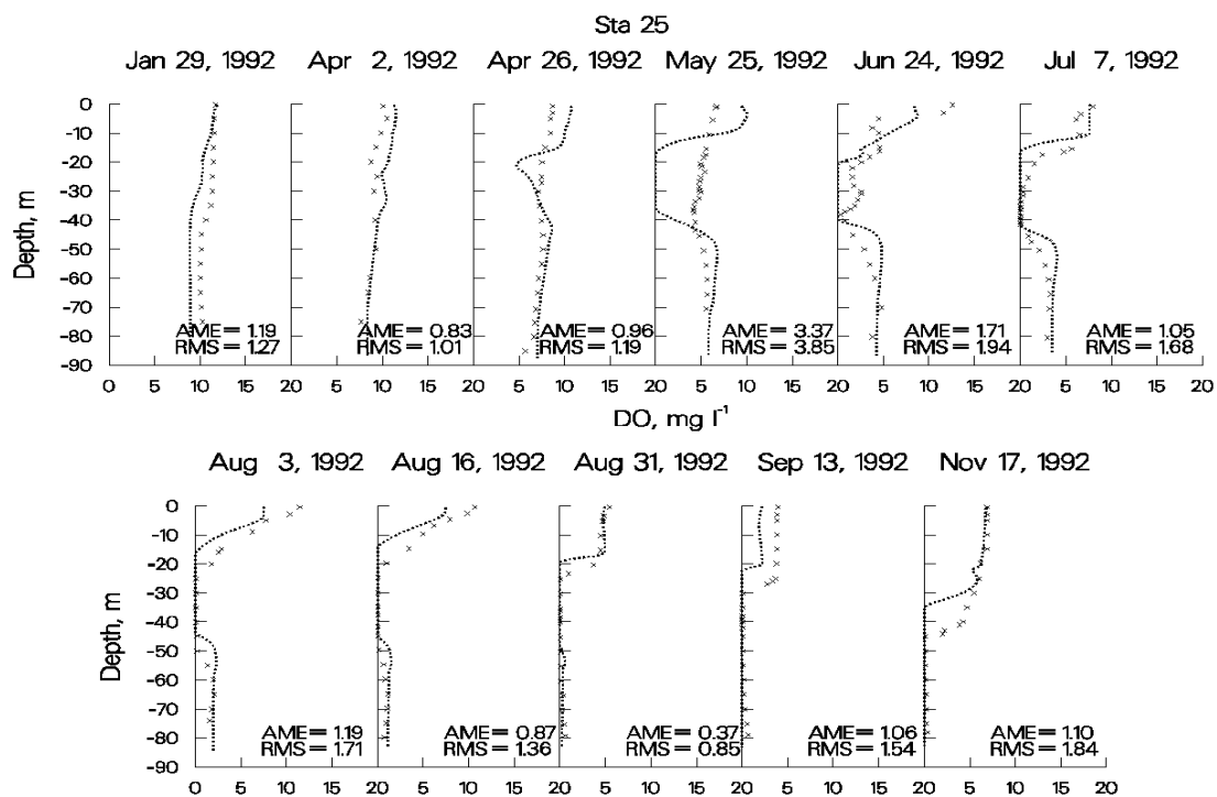
Figure 51. Brownlee Reservoir computed vs. observed DO.
