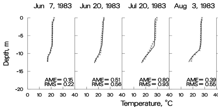
Figure 42. 1983 Bluestone Reservoir computed versus observed temperatures.
