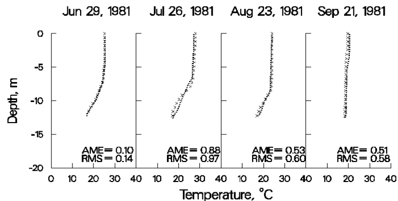
Figure 41. 1981 Bluestone Reservoir computed versus observed temperatures.
