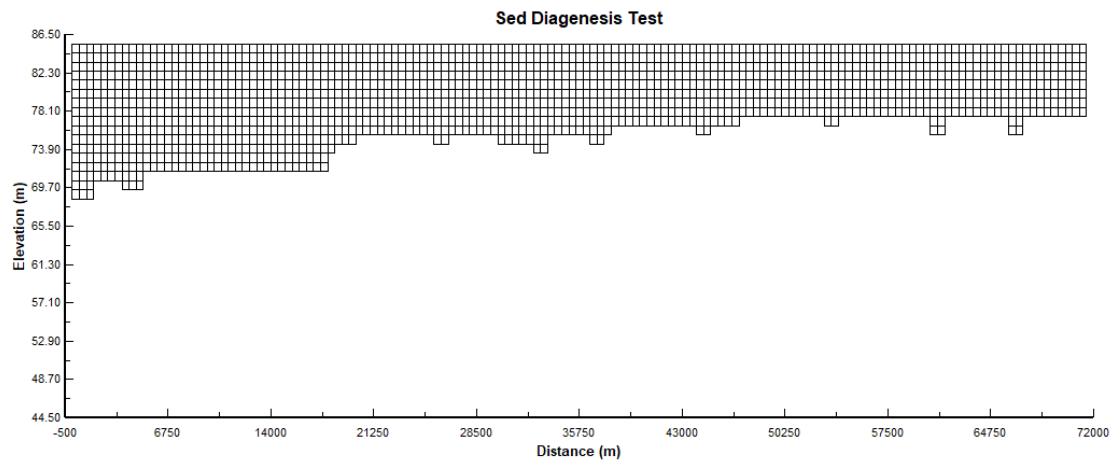
Figure 31. Side view of Branch 1 of sediment diagenesis example.
