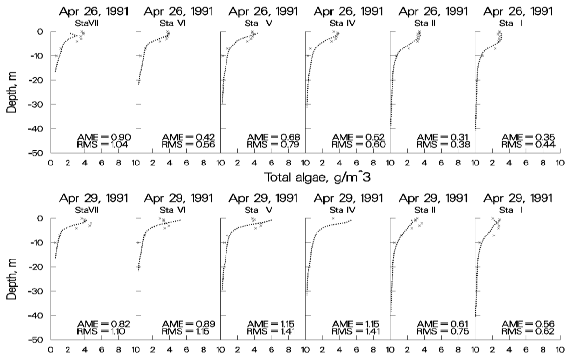
Figure 76. Rimov Reservoir computed vs. observed phytoplankton with wind rotated 90°.
