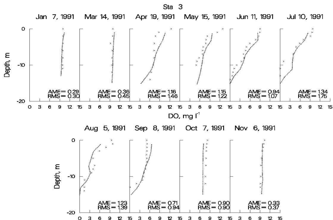
Figure 63. Weiss Reservoir computed vs. observed DO.
