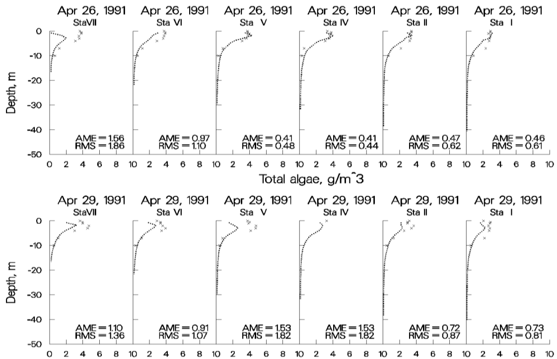
Figure 82. Rimov Reservoir computed vs. observed phytoplankton with no inflowing phytoplankton.
