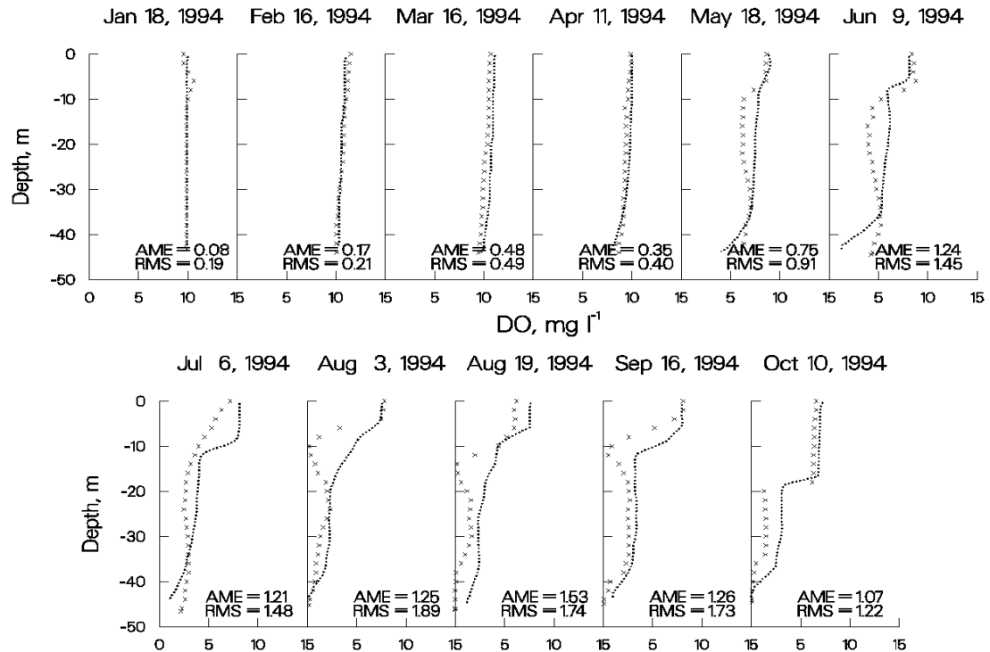
Figure 58. J. Strom Thurmond Reservoir computed vs. observed DO.
