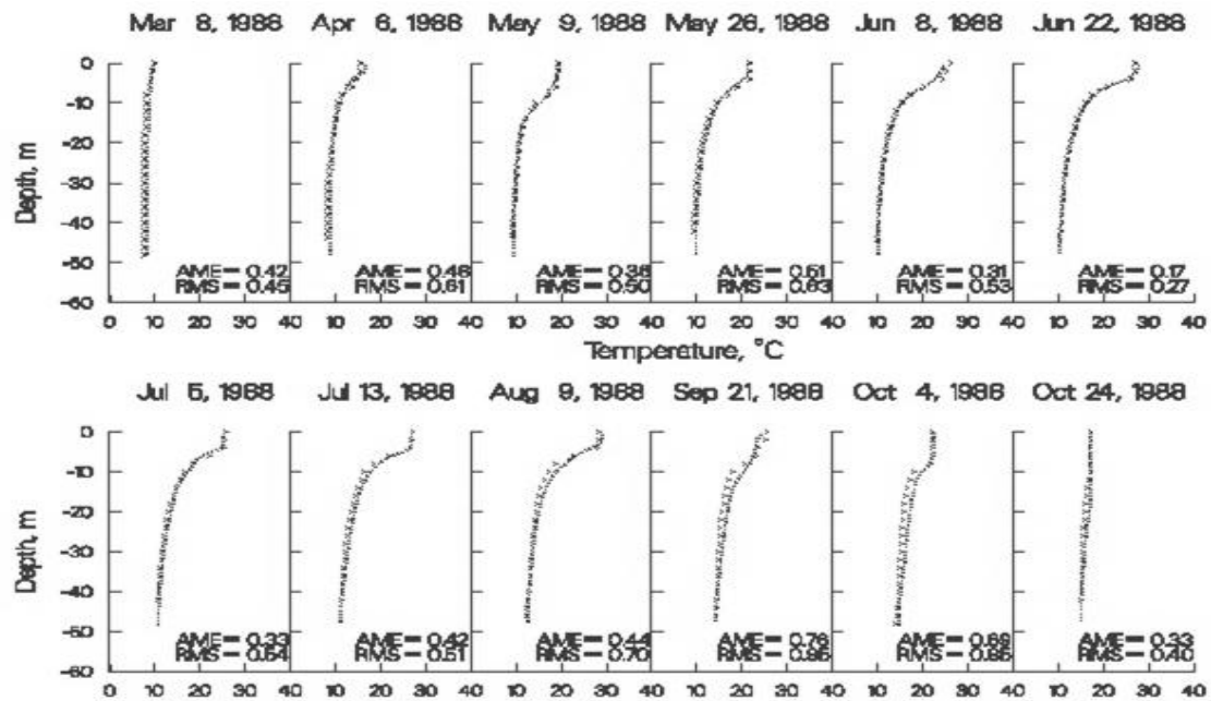
Figure 43. 1988 Richard B. Russell computed versus observed temperatures.
