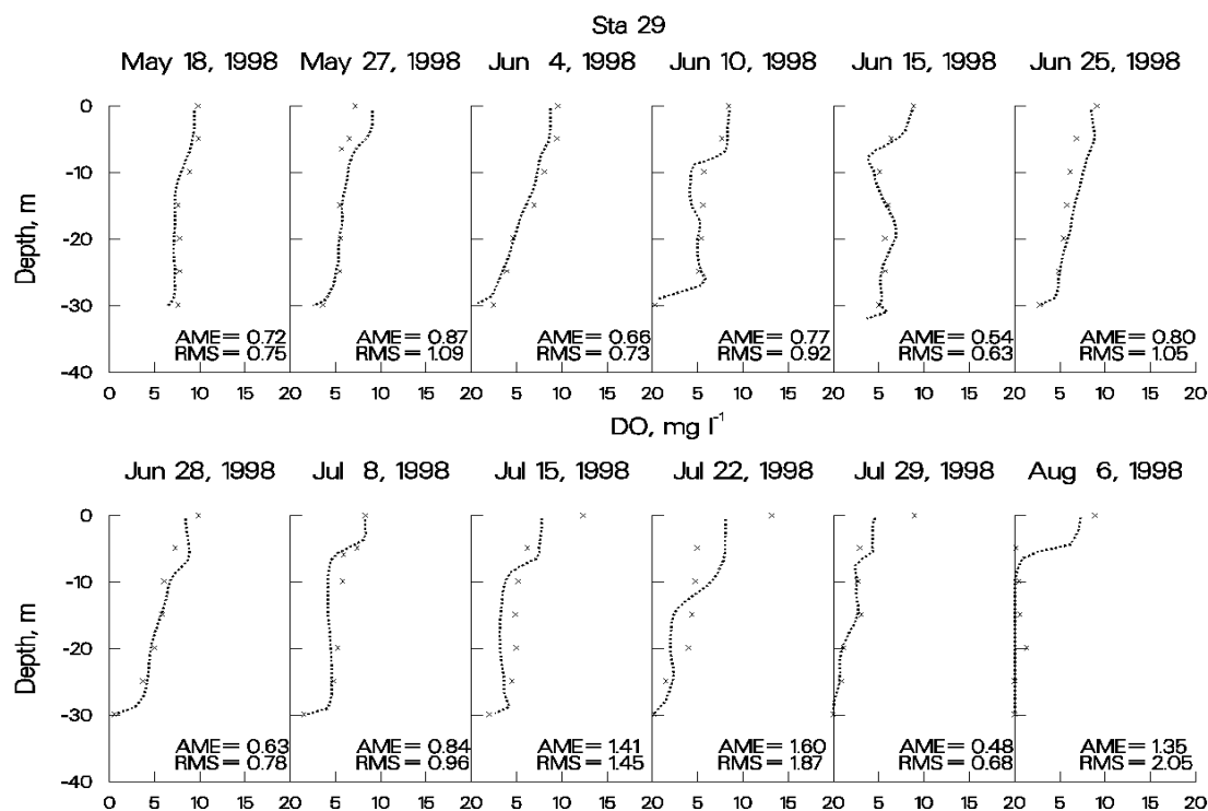
Figure 61. Shepaug Reservoir computed vs. observed DO.
