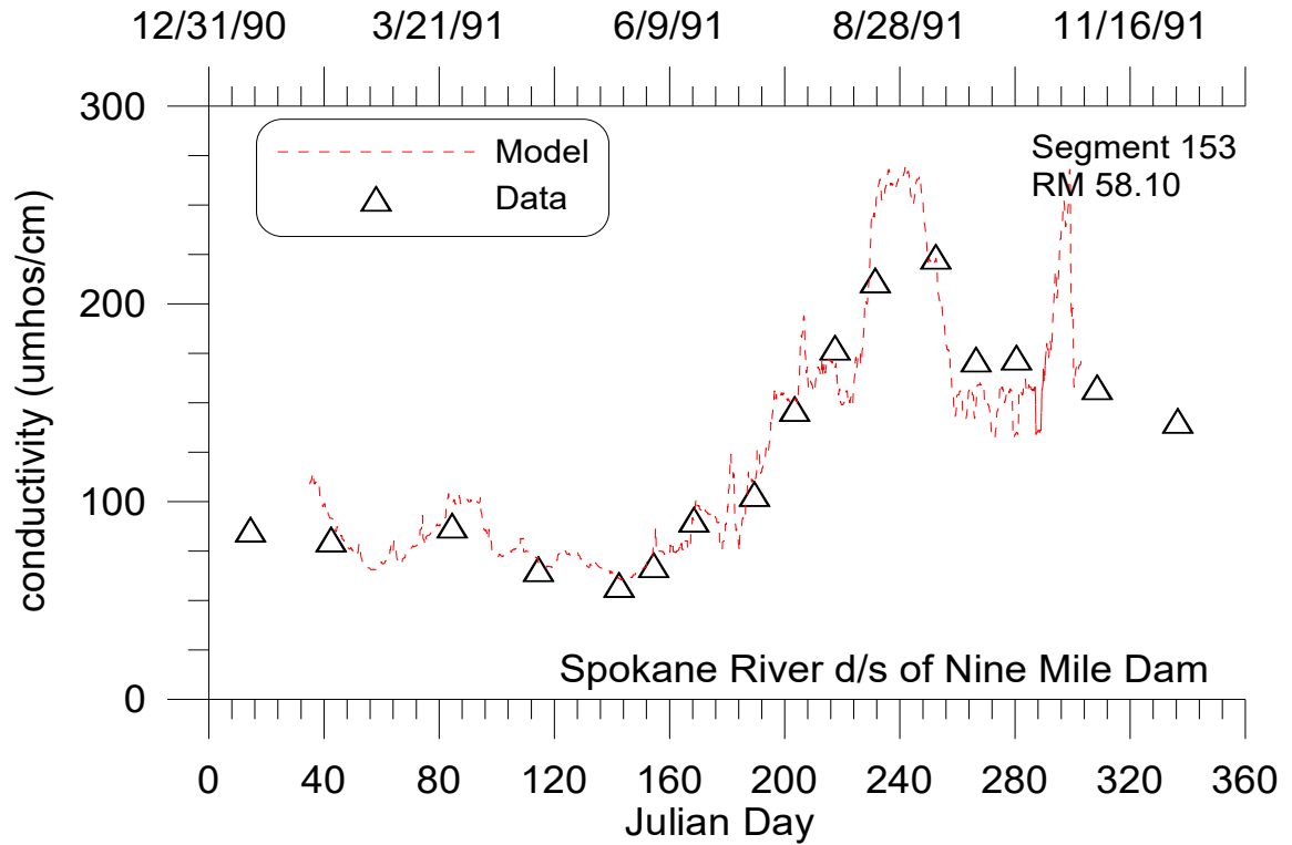
Figure 99. Spokane River computed versus observed conductivity below Nine Mile Dam.
