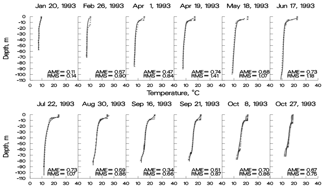
Figure 40. 1993 Pineflat Reservoir computed versus observed temperatures.
