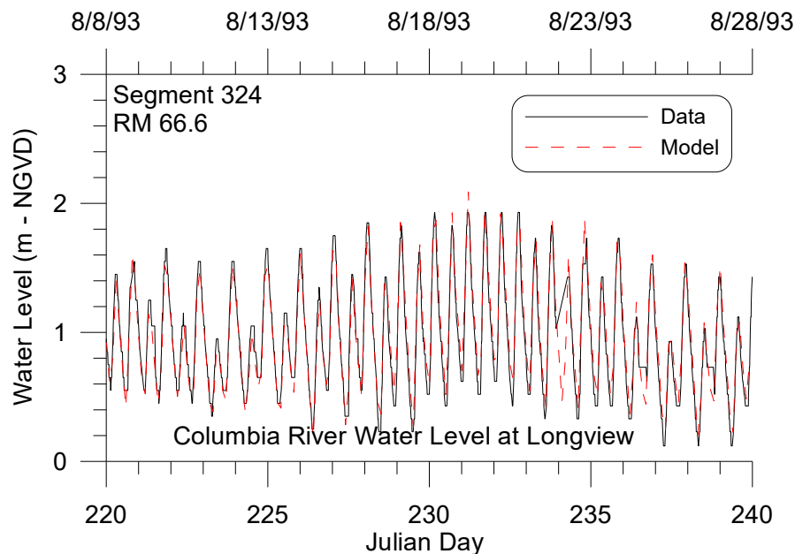
Figure 84. Water level data versus model predictions for Longview, WA during a 20-day period in 1993.
