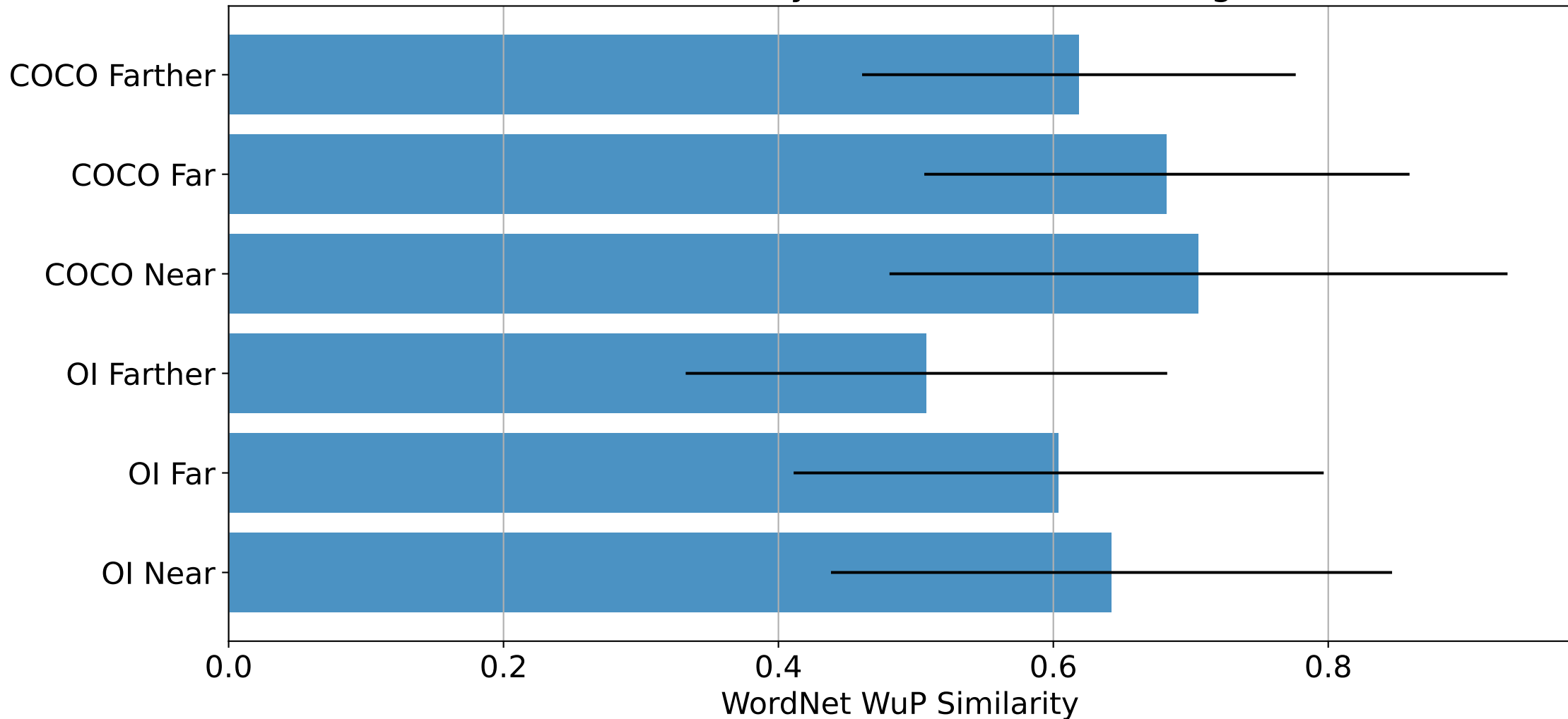
WordNet similarity to VOC and BDD categories
