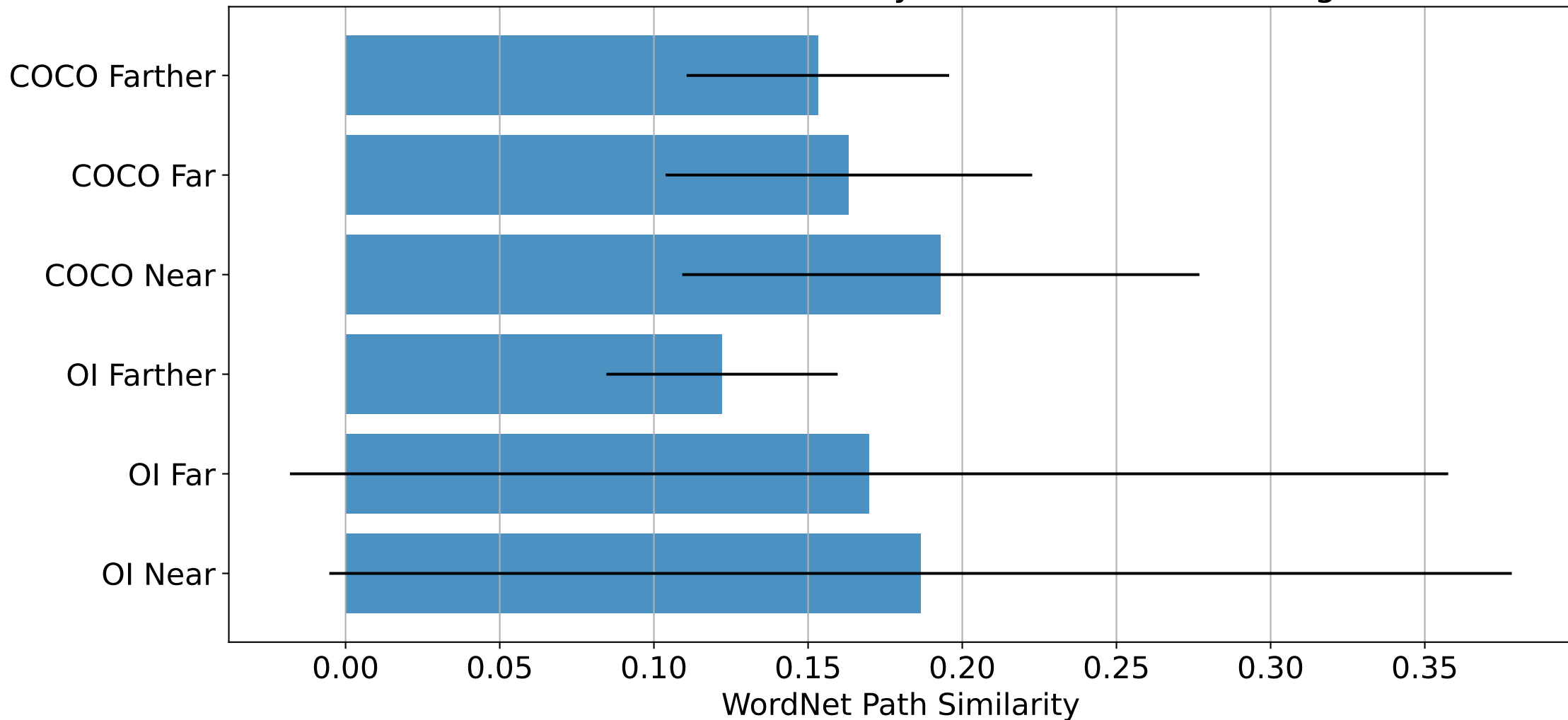
WordNet Path mean similarity to VOC and BDD categories
