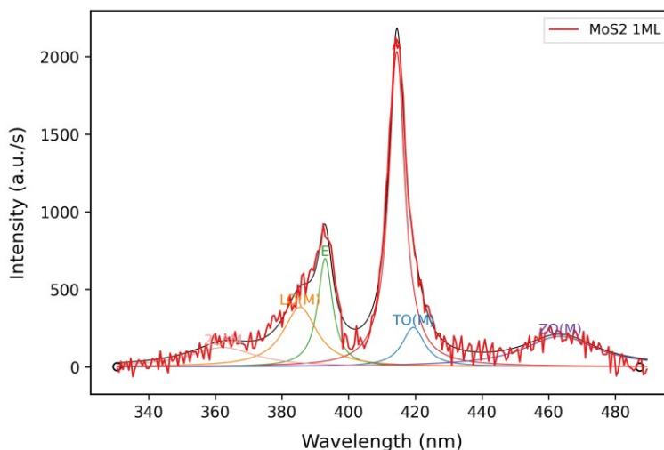
Figure 4: Example of a \text{MoS}_2 spectrum after baseline subtraction and multi-peaks fitting.
