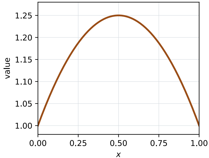
(b) Exact function u
