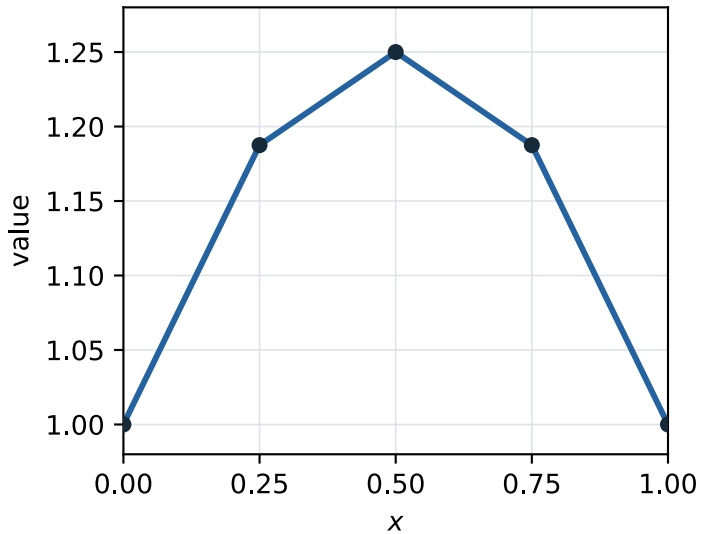
(a) Interpolant \mathcal{I}_h u
