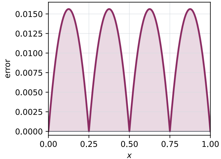
(c) Error u - \mathcal{I}_h u
