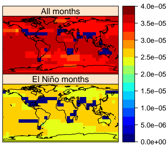
Closeness centrality
