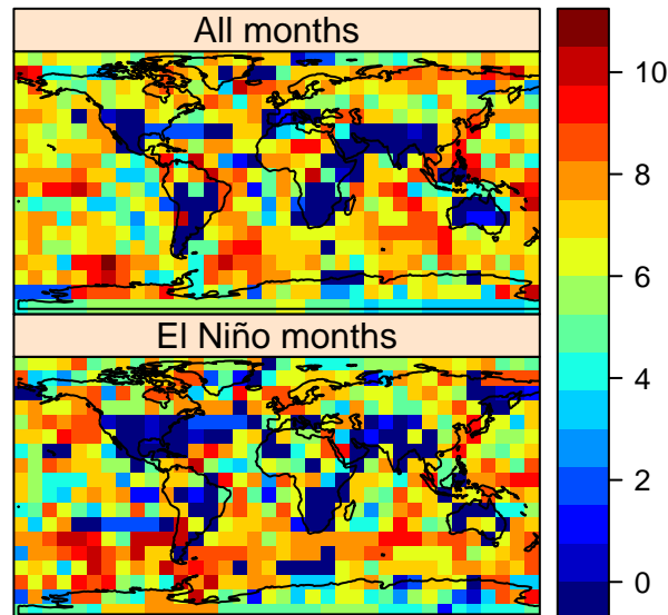
Betweenness centrality
