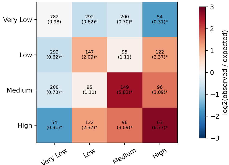
Top 2,000 isolated-isolated pairs ( \leq 5 per protein)
