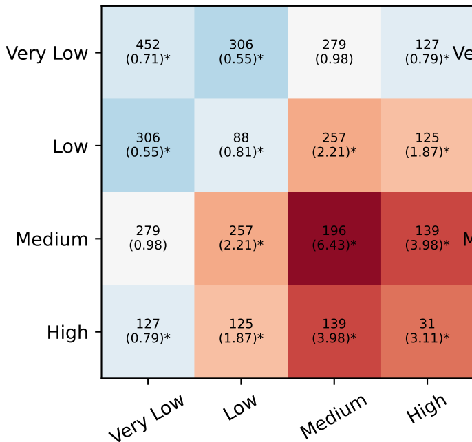
Top 2,000 isolated-connected pairs ( \leq 5 per protein)
