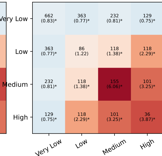
Top 2,000 isolated-isolated pairs ( \leq 5 per protein)
