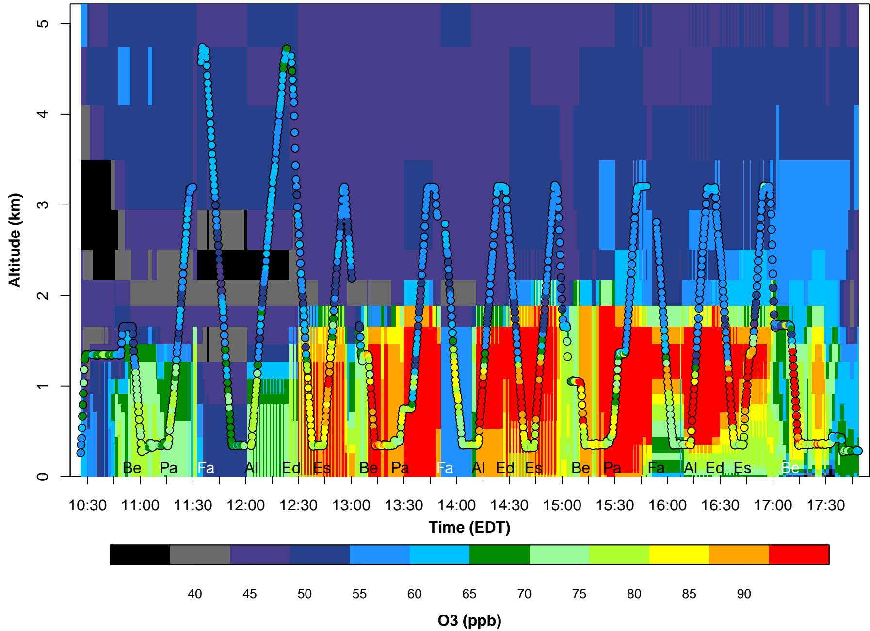
P3B (15s) vs pNLDN (hourly) O3 (ppb) on 2011-07-28
