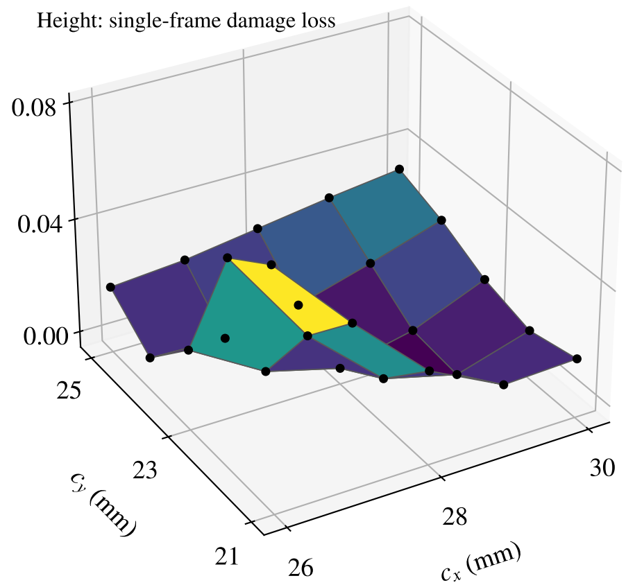
(a) 25 retained FEM evaluations
