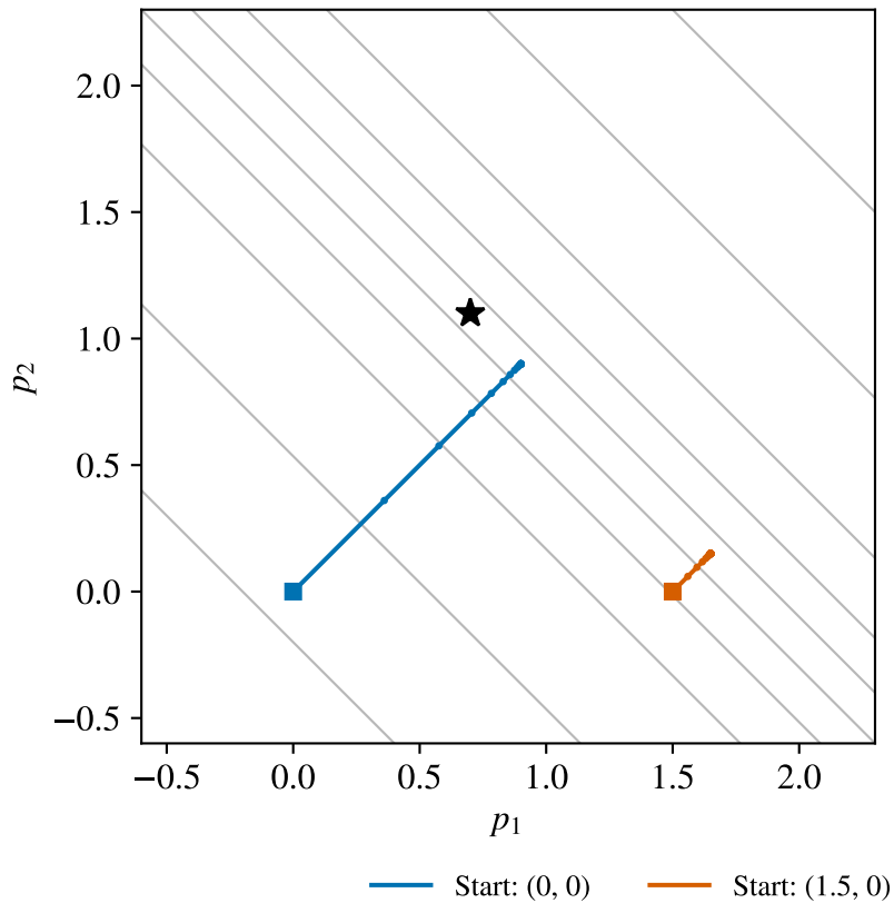
One observation
