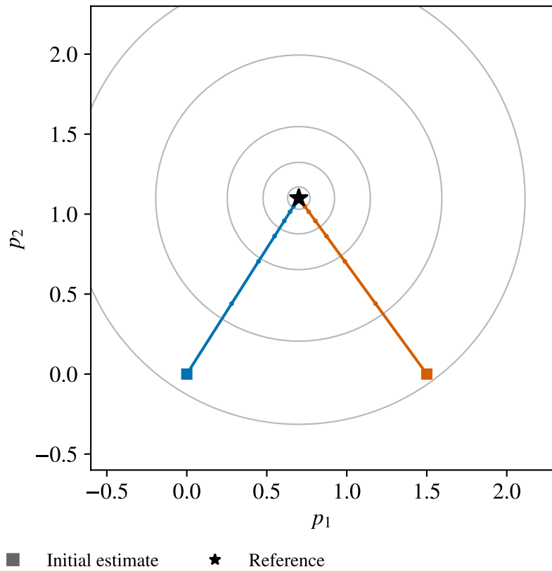
Two observations
