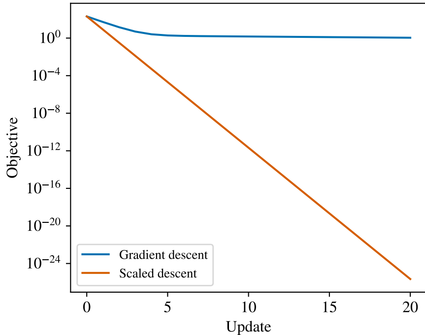
(b) First 20 updates
