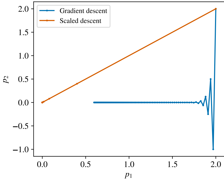
(a) Recorded parameter paths
